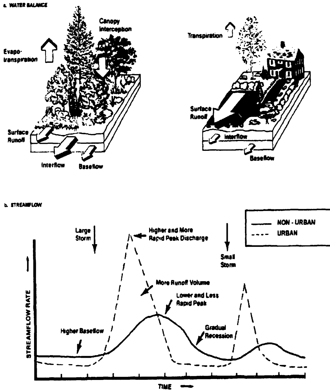
Figure 1. Watershed Hydrology as a Result of Urbanization (Schueler, 1987:1.3)
