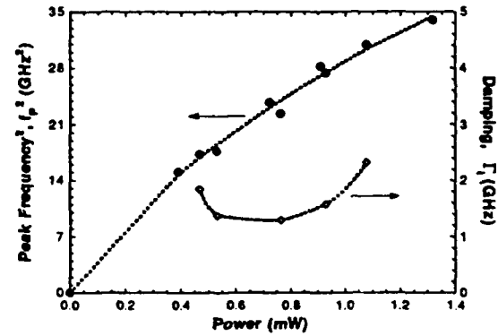
Fig. 3 Relaxation resonance frequency, f_p , and damping factor, \Gamma_i , of 6µm VCSEL extracted from RIN data
