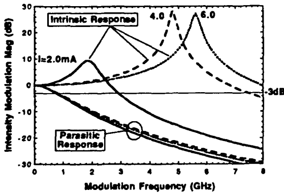
Fig. 4 Calculated intrinsic (using RIN data) and extrinsic (measured parasitics) response of 6µm VCSEL.
