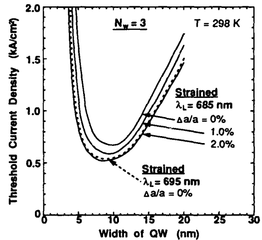
Fig. 4 Comparison of calculated results for threshold current density which depends on oscillation wavelengths and net compressive strains induced by lattice-mismatch in strained MQWs.
