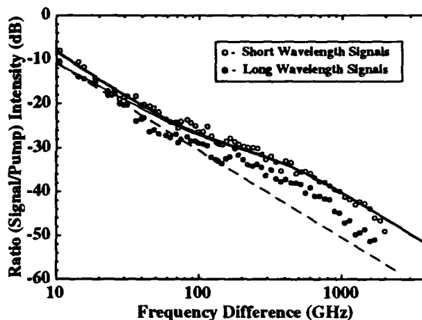
Fig.2: Ratios of conjugate to pump beam intensities for an 16-well strained-layer TWA.
