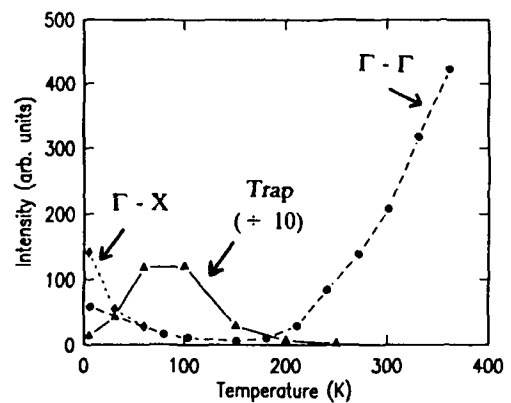
Fig. 5: Temperature dependence of PL peaks
