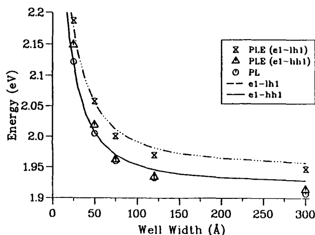
Fig.2. 5K e1-hh1 and e1-lh1 transition energies vs. well width and envelope function fitting for \sim 0.5\% compressively strained structures.
