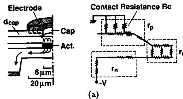
Fig. 2 Current flow and device resistance of CPBH-SELD. (a) Analysis model and (b) theoretical and experimental results versus thickness of cap layer.
