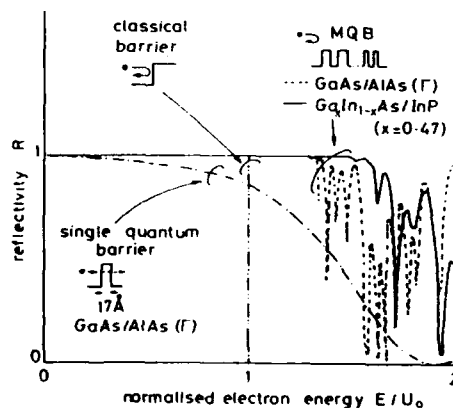
Fig. 2 The reflectivity of MQB
