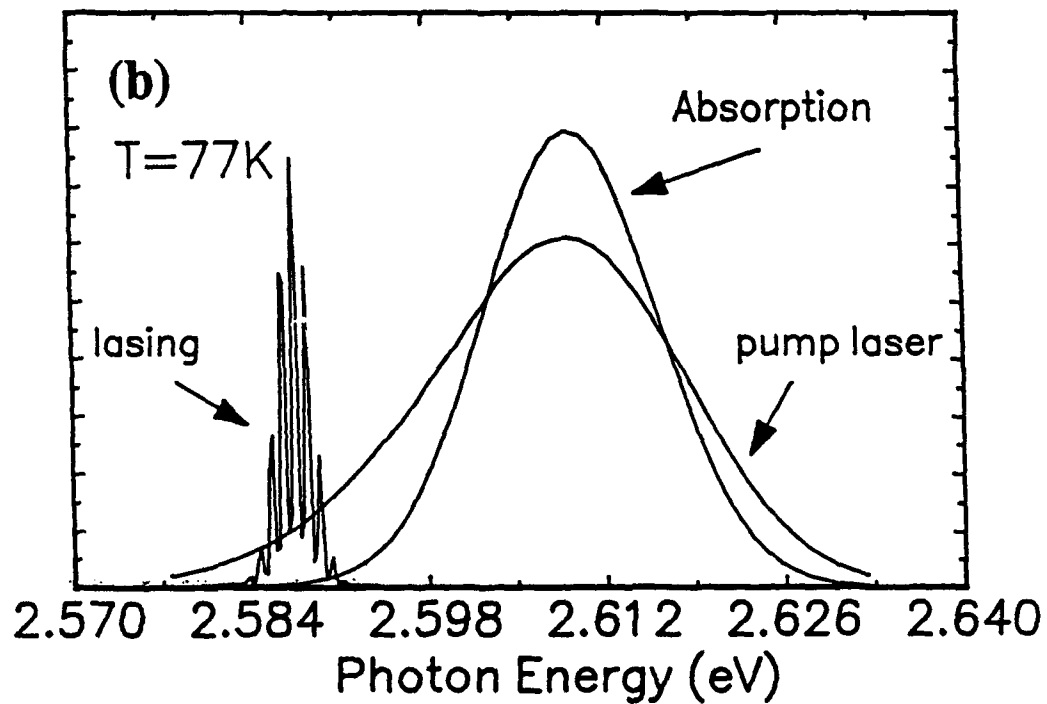
Figure 1: (a) Schematic of the experimental arrangement; (b) The absorption spectrum near the n=1 HH exciton resonance of the (Zn,Cd)Se/ZnSe QW, pump laser spectrum, and laser emission from a QW structure at T=77\text{K} , respectively.
