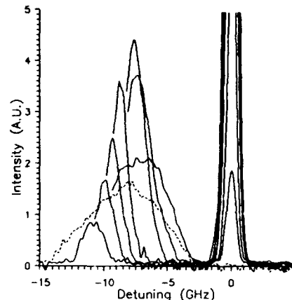
Fig. 3: A gain peak appears at \nu_{inj} - 7 GHz and is pushed to lower frequencies with increased injection.
