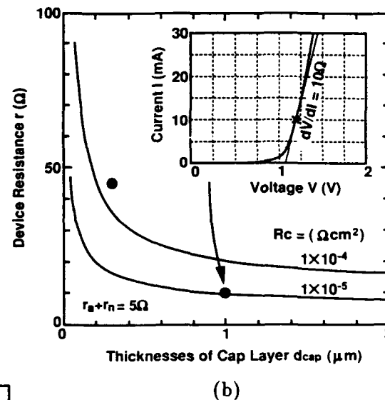
Fig. 2 Current flow and device resistance of CPBH-SELD. (a) Analysis model and (b) theoretical and experimental results versus thickness of cap layer.
