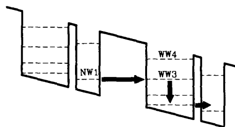
Figure 3: NW1 \rightarrow WW3 resonant electron transport mechanism proposed to explain the data.
