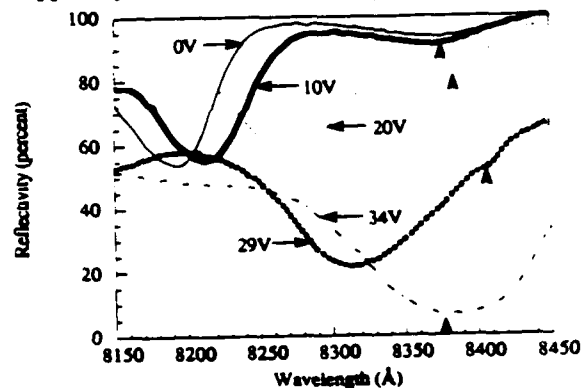
FIGURE 2: Reflectivity versus wavelength for varying bias. Vertical arrows depict the movement of the Fabry-Perot dip.
