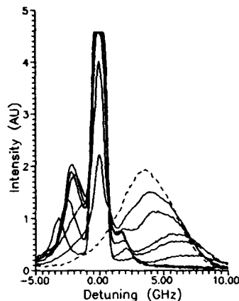
Fig. 1: The original VCSEL spectrum (dashed) is modified (solid) by increased injection power.
