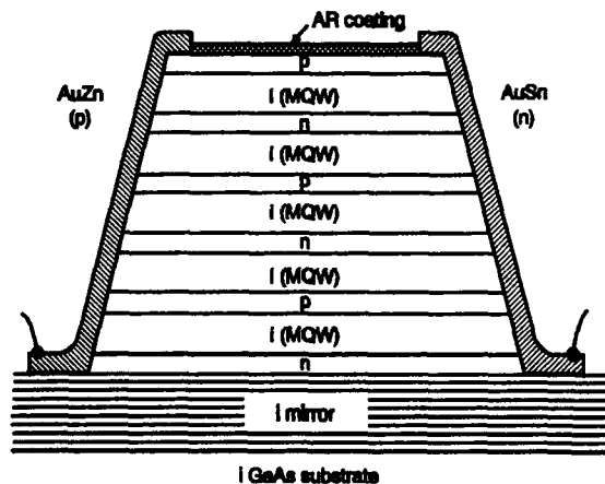
Fig. 1: Schematic of our modulator. A p^+(n^+) region forms under the AuZn(AuSn) electrodes, forming selective contacts to the p(n) layers. Each MQW consists of twenty periods.
