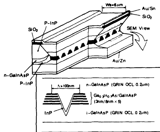
Fig.3 Schematic structure of Ga_{0.3}In_{0.7}As/InP GRIN-SCH 5-layered compressive strained quantum-well laser with wire active region.
