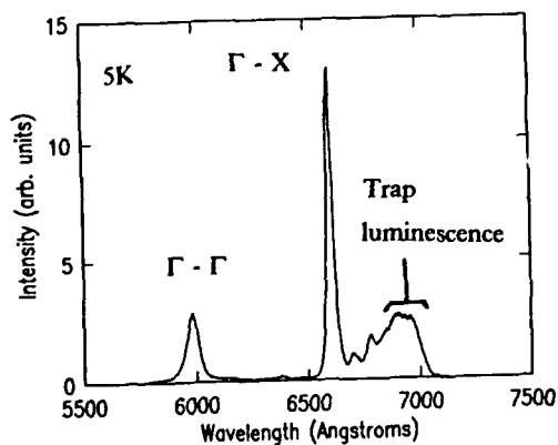
Fig. 4: Low temperature PL spectra
