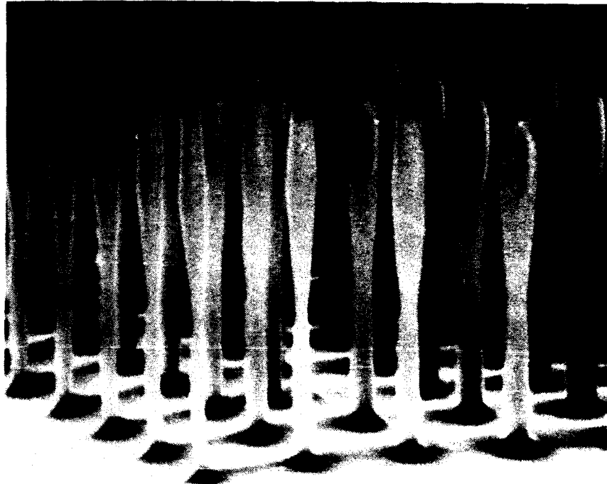
Fig. 1. Scanning electron micrograph of the smallest microcavity VCSELs: 0.4 \mu\text{m} wide by 8 \mu\text{m} tall.
