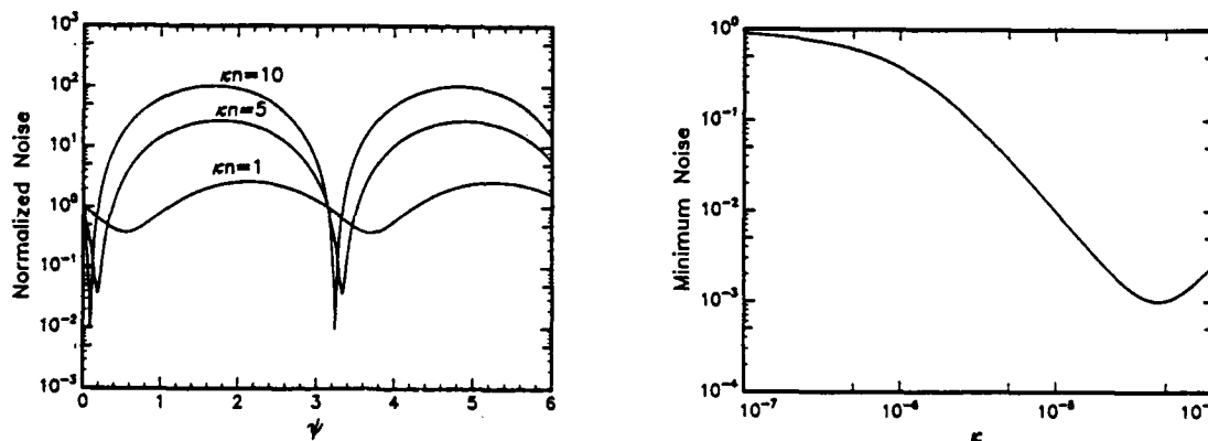
Fig. 2 Noise characteristics for n=10^6
