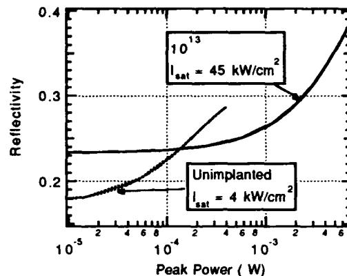
Figure 3: Fit to reflectivity data as a function of incident power for implanted ( 1 \times 10^{13} \text{ cm}^{-2} ) and unimplanted AlAs barrier samples at 8V and 849 nm.
