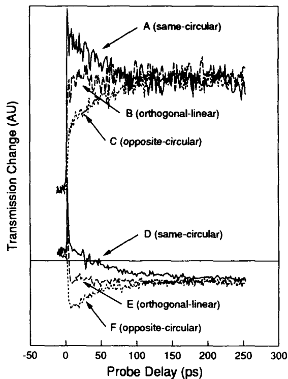
Figure 2. Excite-probe scans for a variety of beam polarisation. Curves A-C were performed at heavy hole resonance while curves D-F were taken on the low energy side of the exciton.
