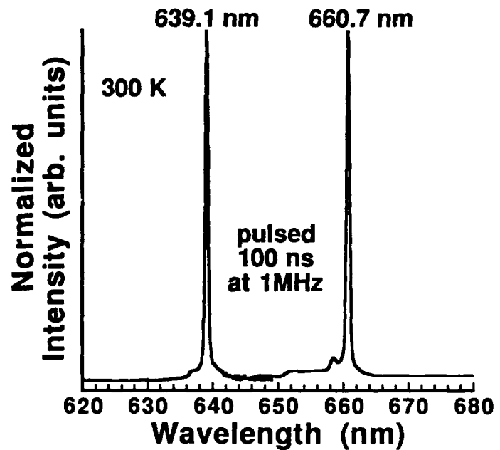
Visible VCSEL diode lasing spectra.
