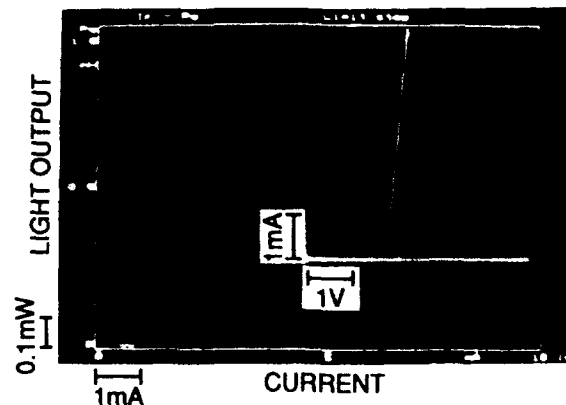
Fig. 6. L-I characteristics for the VCSEL-thyristor. The inset shows I-V characteristics.
