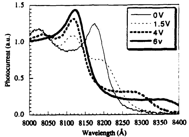
Figure 2: Photocurrent measurements for the structure shown in Figure 1 at various low applied biases where the overlap integral changes dominate absorption changes.
