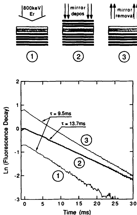
Fig. 3 Luminescence decay measurements after pulsed excitation of an Er-implanted structure before top mirror deposition, in a completed cavity at 1.44\ \mu\text{m} , and after removal of the top mirror. The curves are normalized to their peak intensity and offset for clarity.
