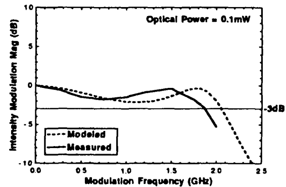
Fig. 5 Total calculated (intrinsic + extrinsic) and measured response of 6µm VCSEL at 2.0mA current.
