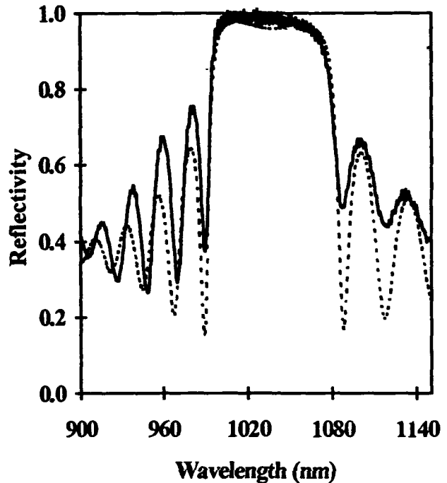
Fig. 2 Zero bias reflectivity: measured (solid line) and calculated (dashed line)
