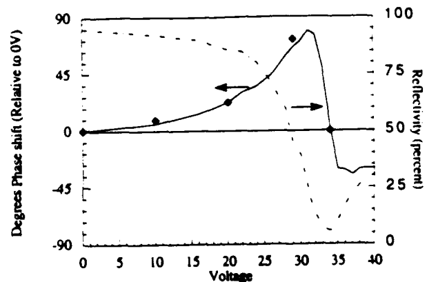
FIGURE 3: Phase and reflectivity versus bias at 8375Å. Reflectivity changes from 94% to 6% as bias changes from 0 to 34 volts. The device exhibits zero phase shift between these two bias points. Dots are simulated phase shift at the voltages of Figure 2.
