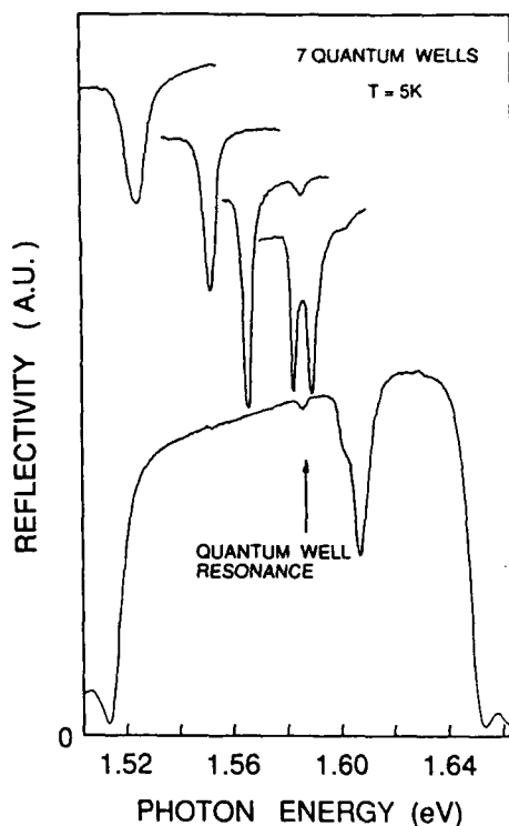
Fig.1 : QW microcavity reflectivity curves for various detuning conditions between cavity and QW exciton frequencies, obtained by choosing various points on the wafer. Note the line narrowing approaching and at resonance, the resonance mode splitting, and the indication of a light-hole exciton mode splitting around 1.605eV.
