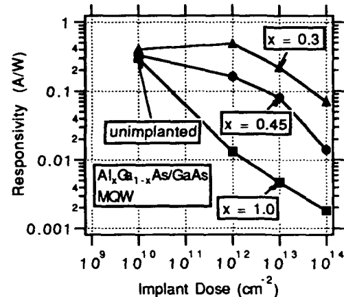
Figure 1: The peak longer-wavelength AR-coated responsivity of samples with Al x Ga 1-x As barriers of x = 0.3 , 0.45, and 1.0, as a function of implant dose at 10 V.
