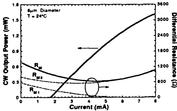
Fig. 2 LI Curve and DBR mirror resistance characteristics of 6µm diameter single-mode VCSEL
