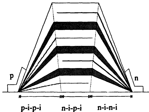
Fig. 1 Inter-digited contact structure. White regions are the AlGaAs bulk layers, 840 Å thick, cross hatched regions are the MQW InGaAs/GaAs layers, with 4 100 Å InGaAs wells and 3 70 Å GaAs barriers. \delta doped contact layers are the thin lines in the middle of the bulk AlGaAs layers.
