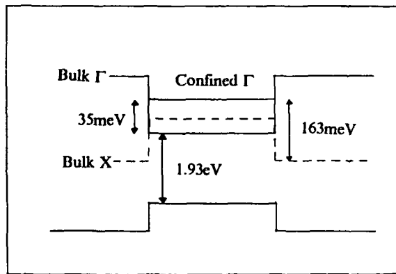
Fig. 3: Approximate 300K band diagram of Al_{0.4}Ga_{0.6}As/AlAs QWs
