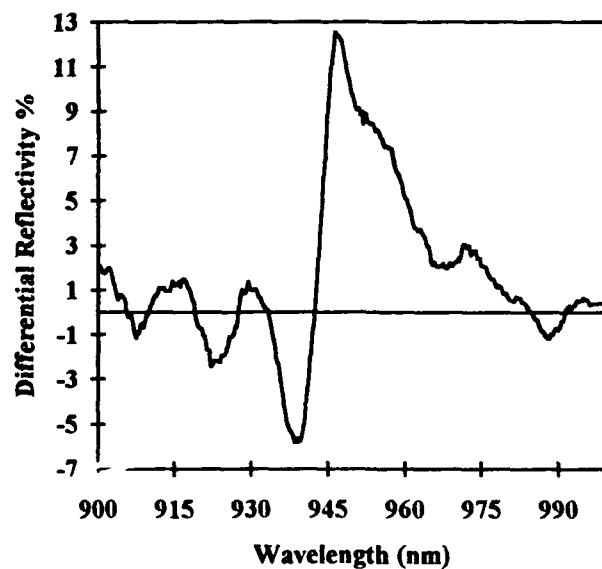
Fig. 3b Measured \Delta R/R for +1V applied
