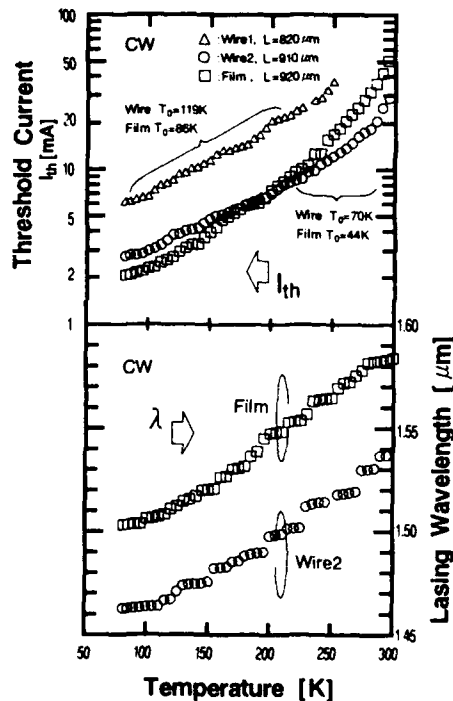
Fig.4 Temperature characteristics of Ga_{0.3}In_{0.7}As/InP GRIN-SCH 5-layered compressive strained quantum-well laser with wire active region.
