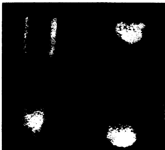
Fig.6 a. ^1\text{H} image of PS beads in tetrahydrofurane. b. - d. corresponding ^{19}\text{F} images after addition of derivatized glycine. Spin-Echo sequence.
