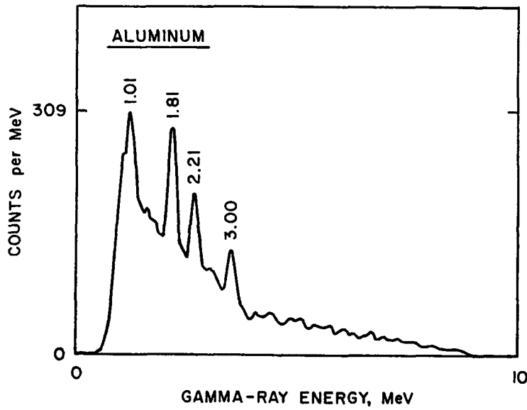
Fig. 11. APSTNG system gamma-ray energy spectra of C and Al targets.
