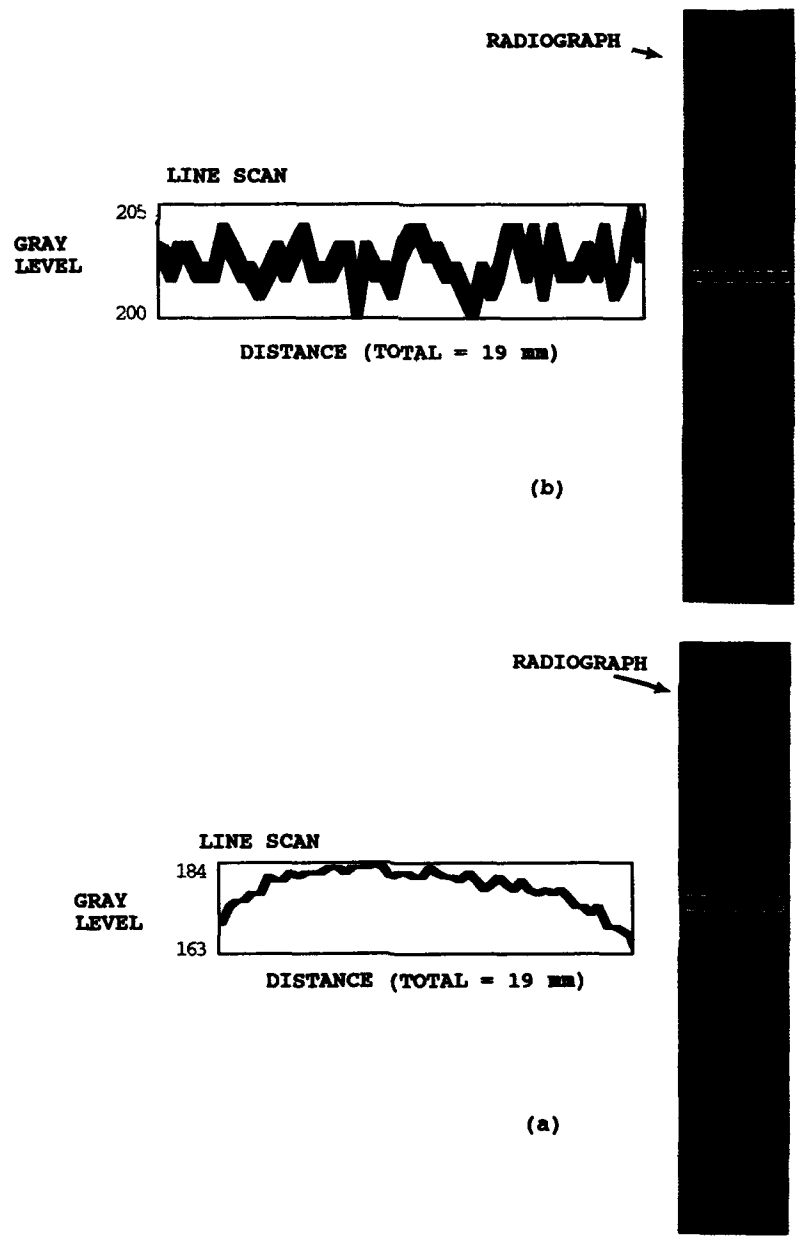
Figure 4. Digitized Radiographs and Line Scans of Carbon Foams of: (a) Bulk Density of 38 mg/cm 3 and (b) Density of 16 mg/cm 3 .
