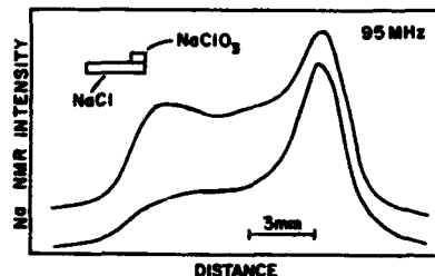
Figure 2. 1-d projections of Na NMR intensity for a sample, illustrated in the inset, containing NaCl and NaClO 3 , for two different pulse lengths showing "pulse length contrast."
