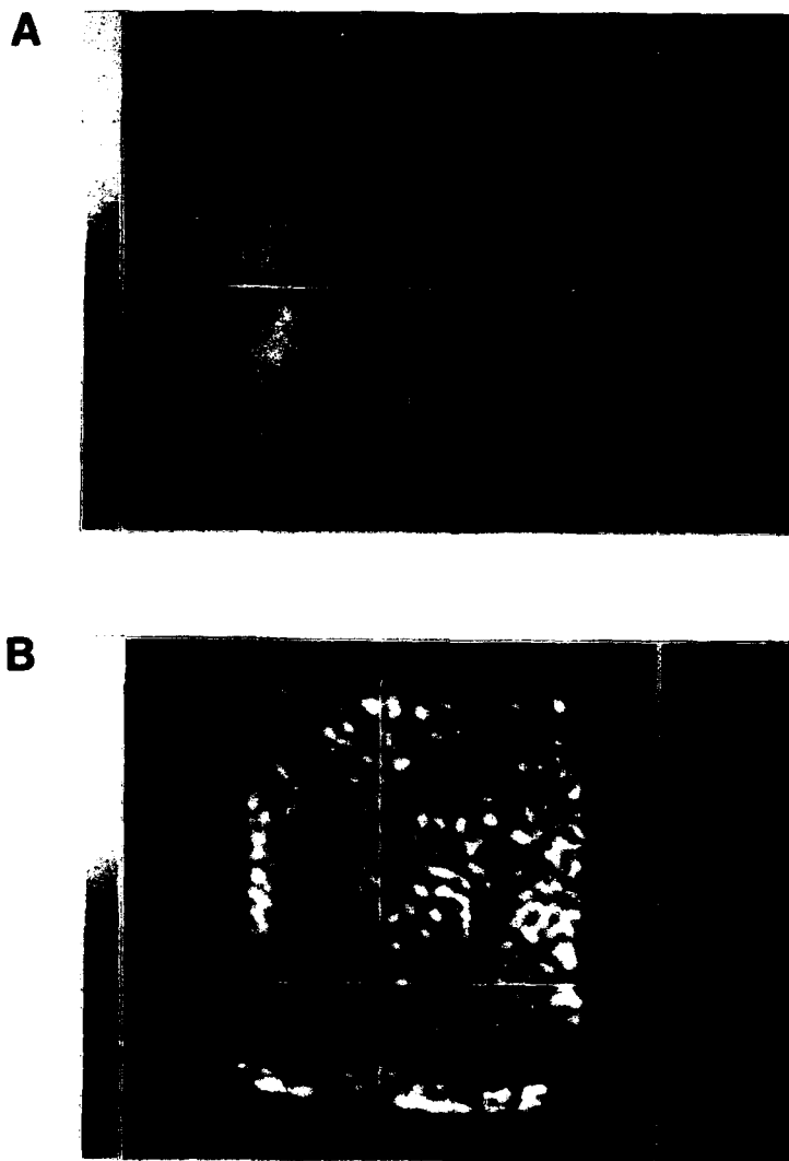
Figure 7. A) {}^7\text{Li} NMR image of a portion of a sintered glass disk (35% porosity, 170-220 \mu\text{m} pore size) with 2 M \text{LiCl} . (1 x 1 x 5 mm voxels; TE = 2 ms; FOV, 64 x 64 mm) B) {}^{19}\text{F} NMR image of a sintered glass disk (40% porosity, 4-5.5 \mu\text{m} pore size) with 50% hexafluorobenzene. (200 x 200 x 2000 \mu\text{m} voxels; TE = 2.8 ms; FOV, 12.8 x 12.8 mm)
