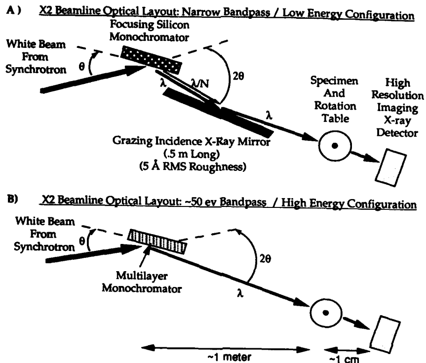
Figure 3. Schematic diagram of two configurations for x-ray tomography experiments on beamline X-2. The configuration shown at the top (Figure 3A) provides a \sim 8 eV bandpass while the configuration shown at the bottom (Figure 3B) provides a \sim 20 eV bandpass. The sample rotation stage and detector are represented with a scale factor different from the rest of the drawing.
