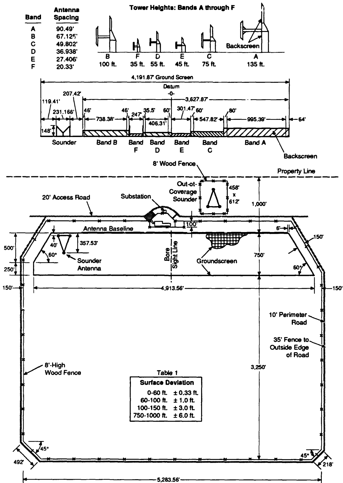
FIGURE 2.1.1 TYPICAL PLAN FOR OTH-B CRS TRANSMIT SECTOR
