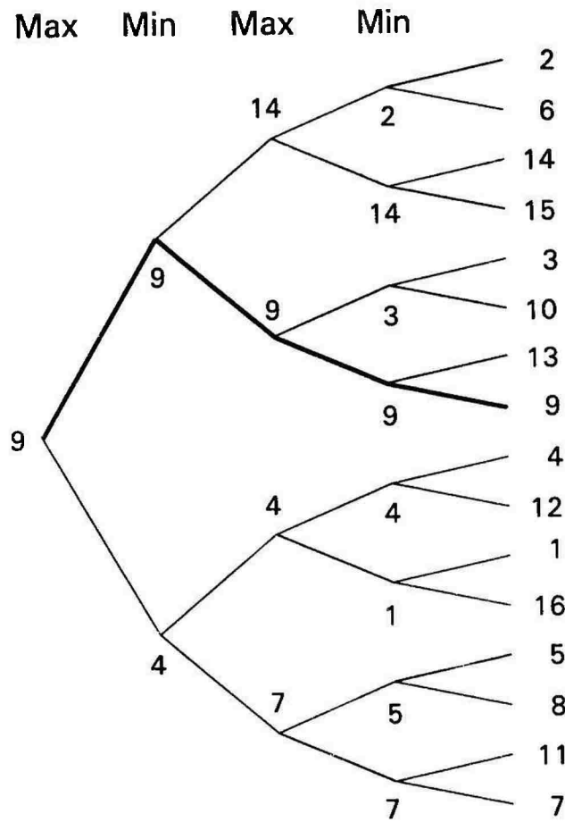
Minimax Search
