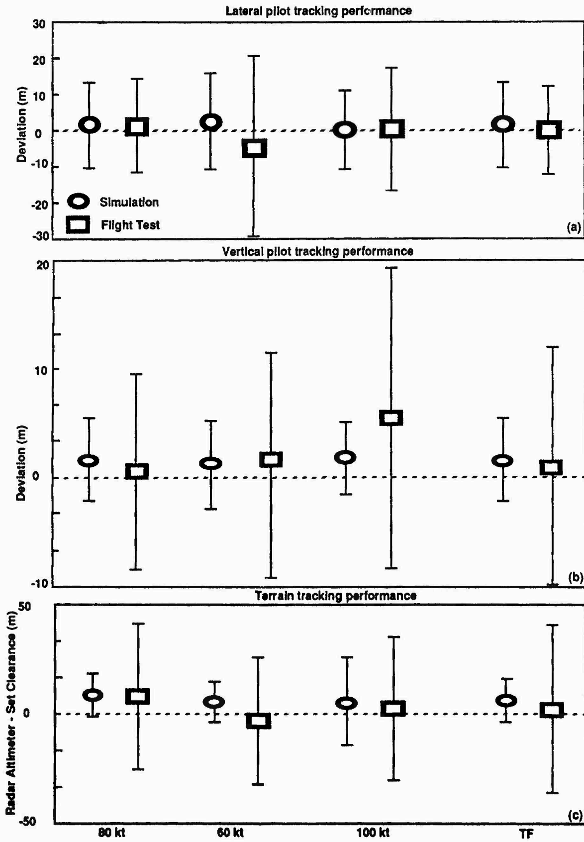
Figure 9, Flight test & simulation statistical comparison
