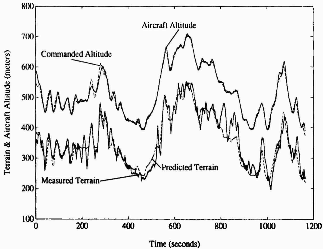
Figure 8, Example vertical trajectory and terrain profile
