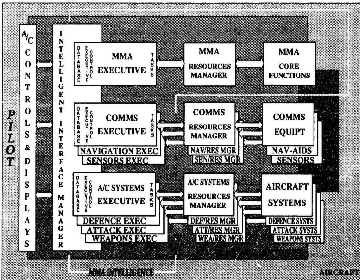
Fig. 2 MMA INTEGRATION WITH BASIC AIRCRAFT ARCHITECTURE
