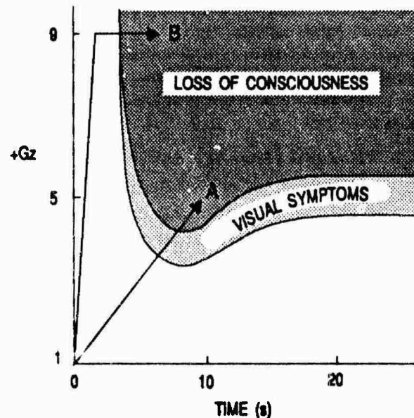
Figure 4. Tolerance to +Gz and effect of onset rate. Line A indicates a moderate G onset rate (1G/s), with loss of consciousness being preceded by greyout and blackout. Line B represents a rapid G onset rate (10 G/s) where loss of consciousness occurs without visual warning.
