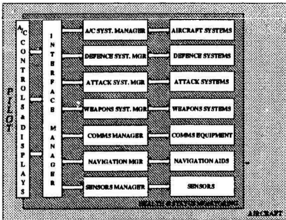
Fig. 1 BASIC AIRCRAFT ARCHITECTURE
