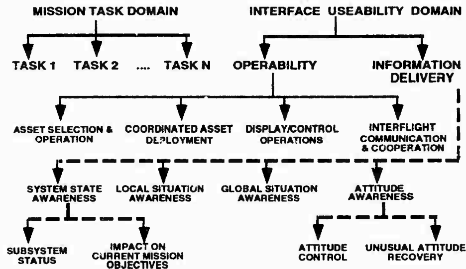
Figure 1. Possible domains or areas where an Intelligent Cockpit might provide knowledge-based aiding to the crew.
