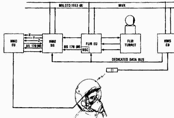
Figure 8. Electronic System Architecture
