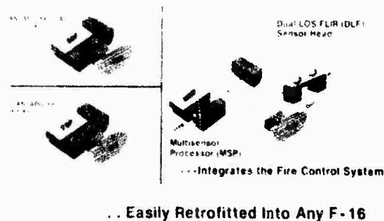
Figure 17. Falcon Knight FLIR/Radar Integration designs were developed for both the F-16A/B's AN/APG-66 FCR and the F-16C/D's AN/APG-68 FCR.
