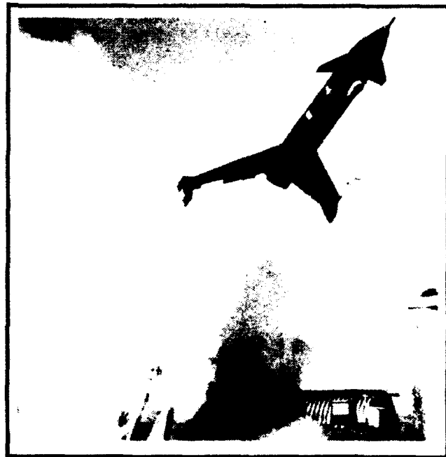
The ROBOT-X with Five CRV-7 Rocket Motors Used for Launch Boost
