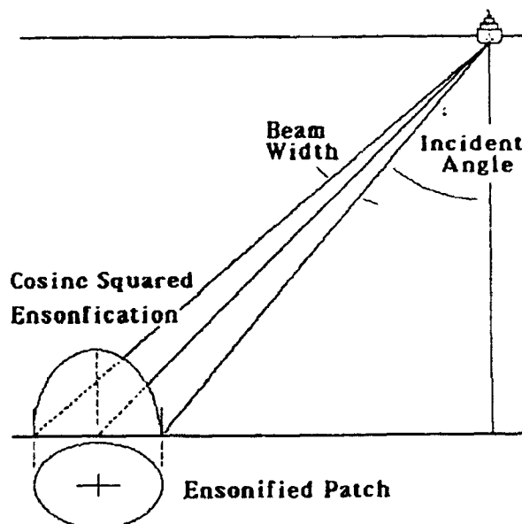
FIGURE 2: Scattering geometry
