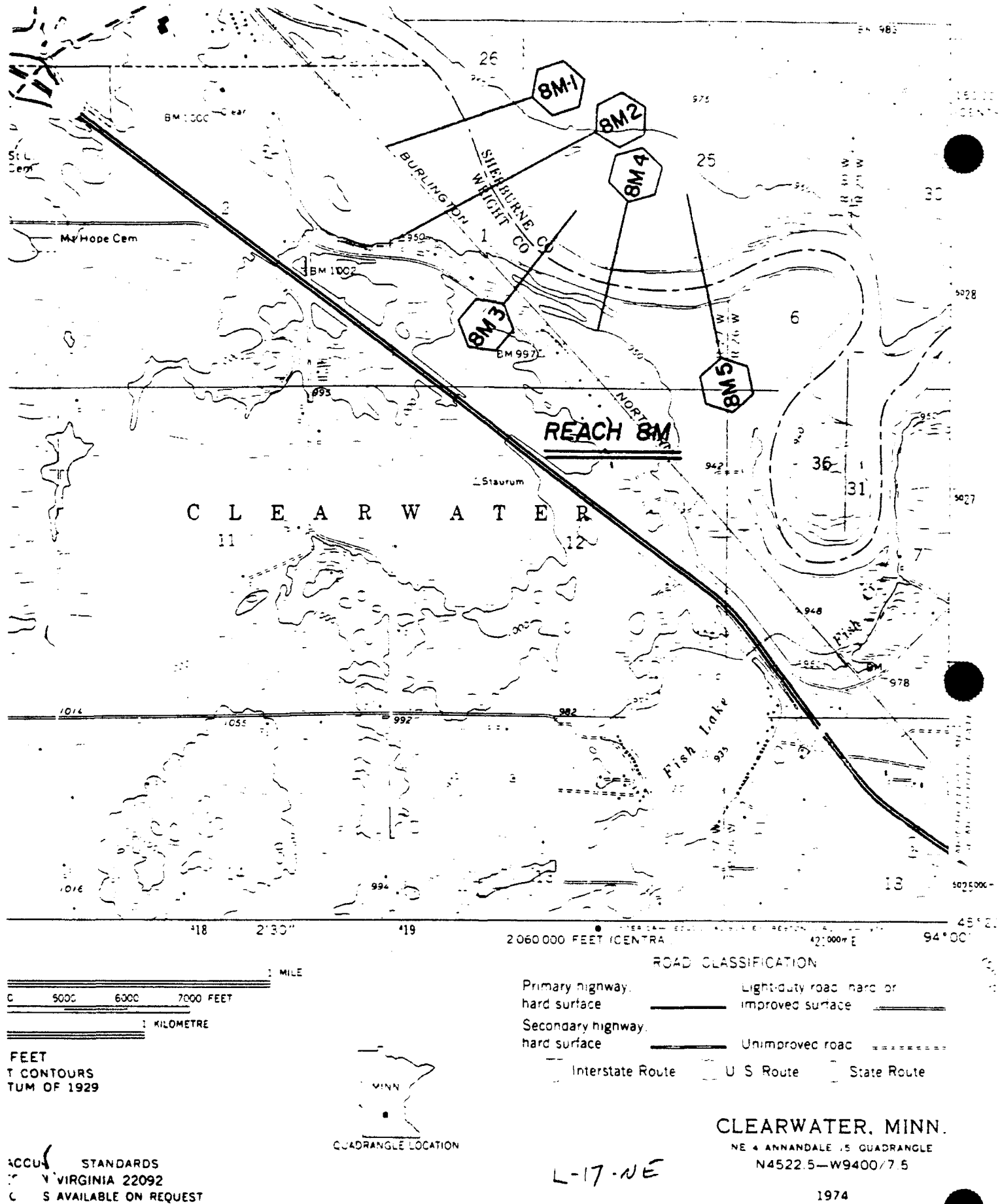
E-16 Figure E-7. Location of hydraulic survey transects, reach 8M, Mississippi River near Clear Lake, Minnesota.
