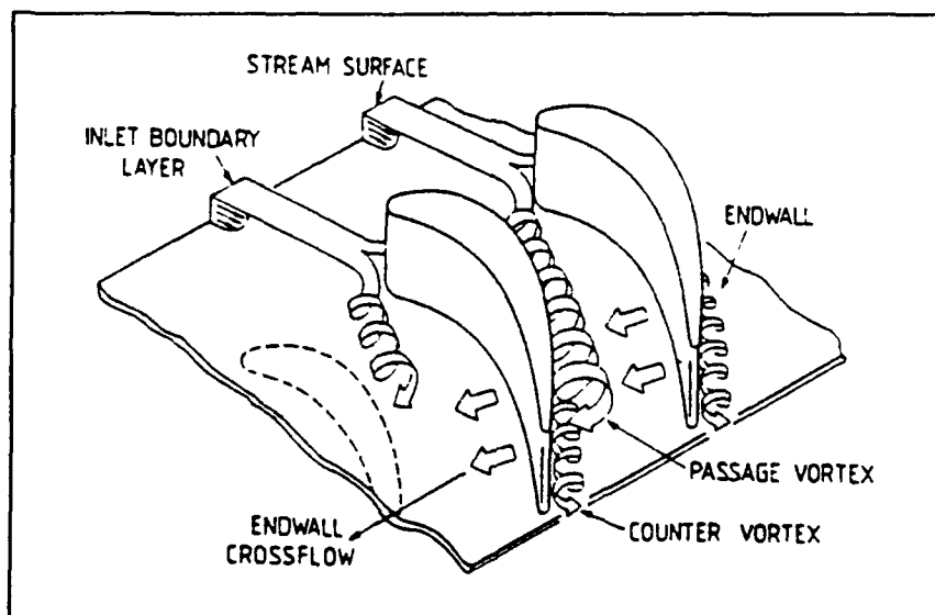
Figure 1. Development of Vortical Flow Within Blade Passages
