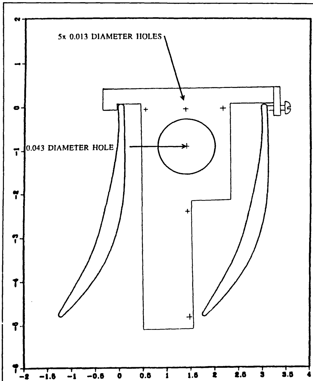
Figure 11. Aligning Tool
