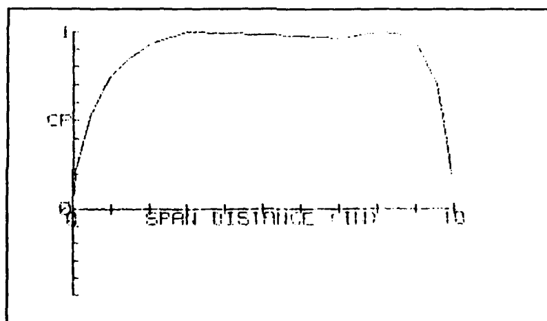
Figure 15. Upstream Spanwise Pressure Distribution for Station 6
