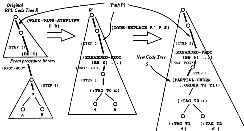
Figure 7 Transforming Code Trees
