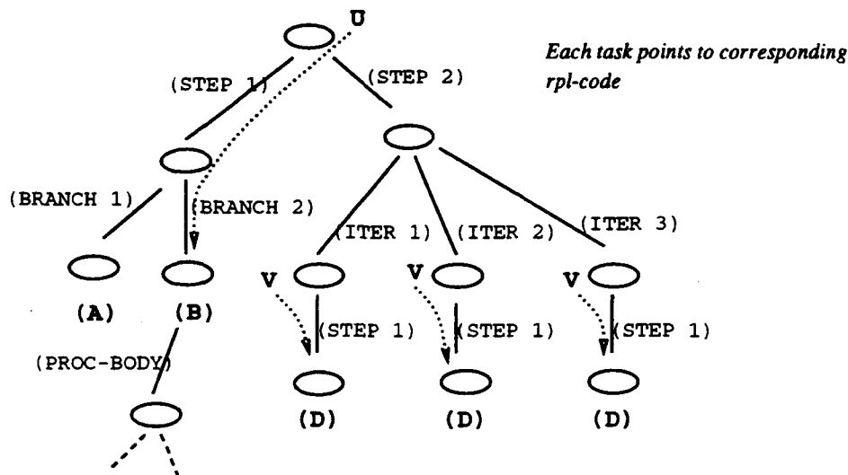
Figure 5 Task network for the plan in Figure 4
