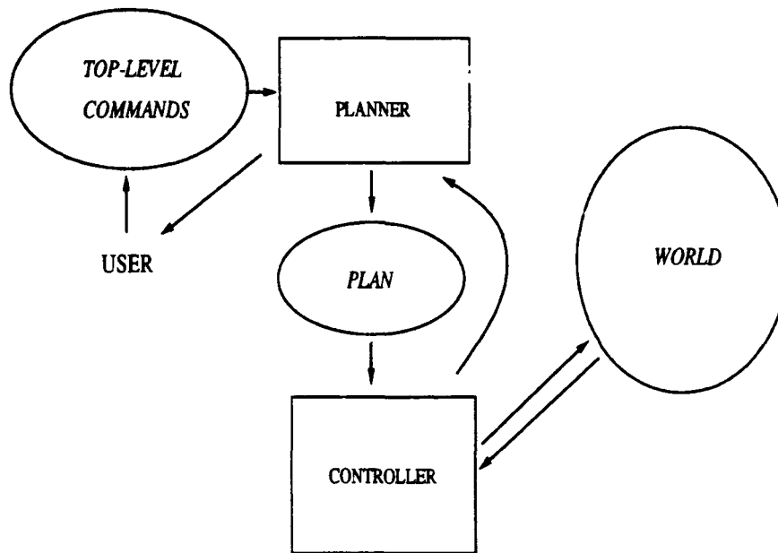
Figure 3 Agent Architecture
