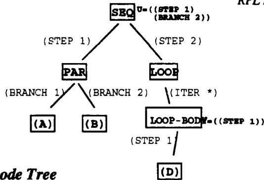
Figure 4 Rpl-code tree for a plan
