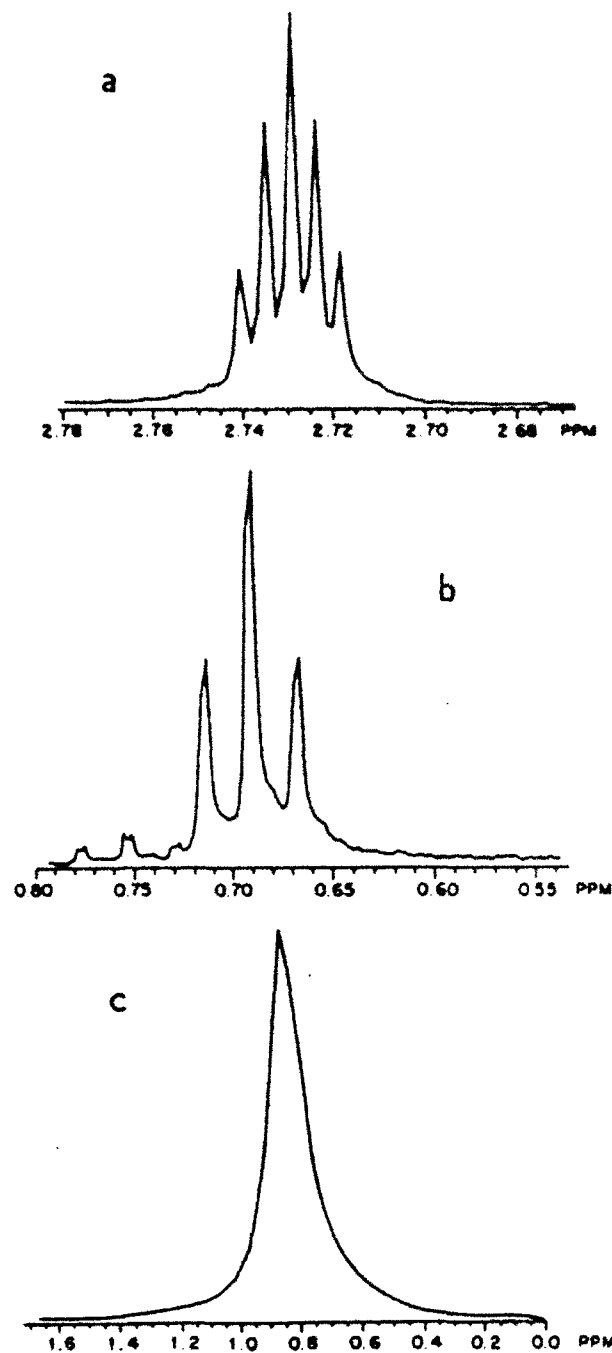
Figure 4. NMR spectra for Zn(O_2P(OEt)_2)_2 : (a) methylene (-CH 2 -) protons; (b) methyl (-CH 3 ) protons; (c) phosphorus atoms.
