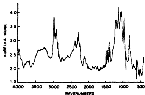
Figure 5. Infrared spectrum of Zn(O_2P(OC_2H_5)_2)_2 .
