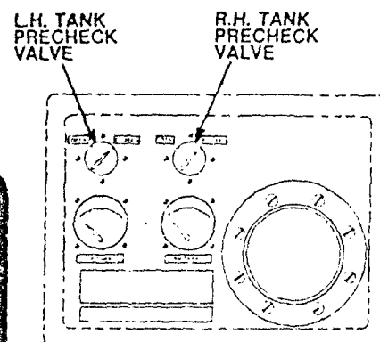
GROUND REFUELING PANEL CH-53A/D
