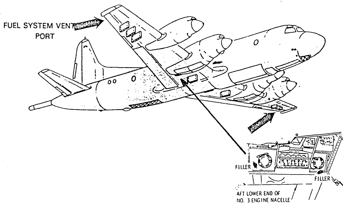
GROUND REFUELING PANEL AND RECEPTACLE
