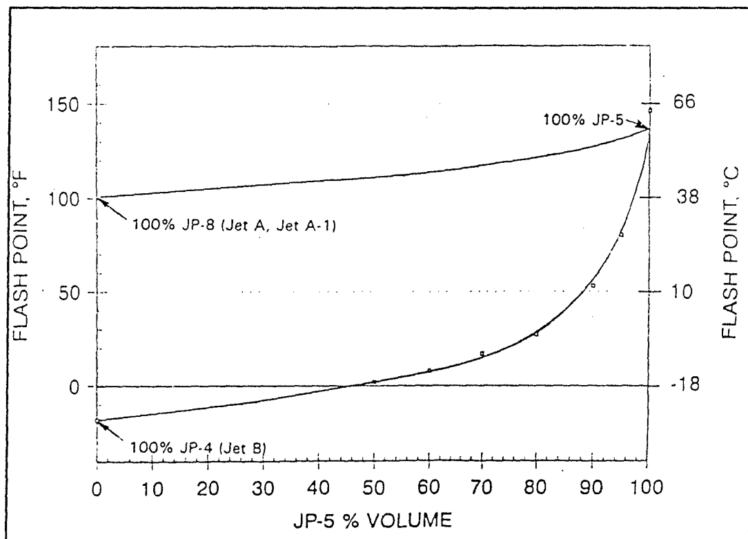
Figure 6-3. Flash Point of Turbine Fuel Mixtures.
