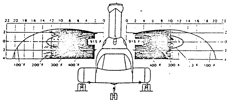
ENGINE EXHAUSE WAKE PROFILE - FEET
