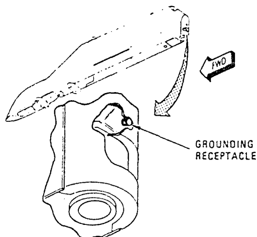
WING PYLONS
