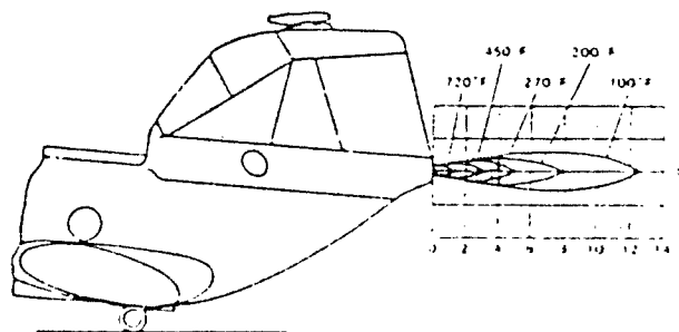
APIJ EXHAUST WAKE PROFILE - FEET
