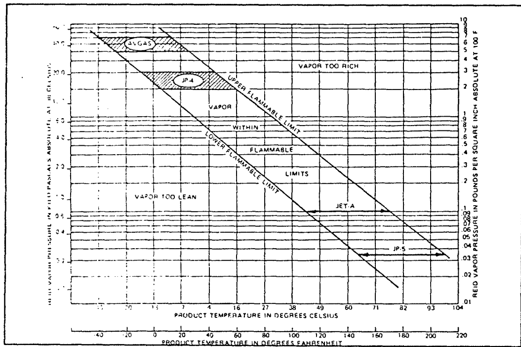
Figure 6-1. Relationship Between Temperature, Rvp, and Flammable Limits of Petroleum Products at Seat Level
