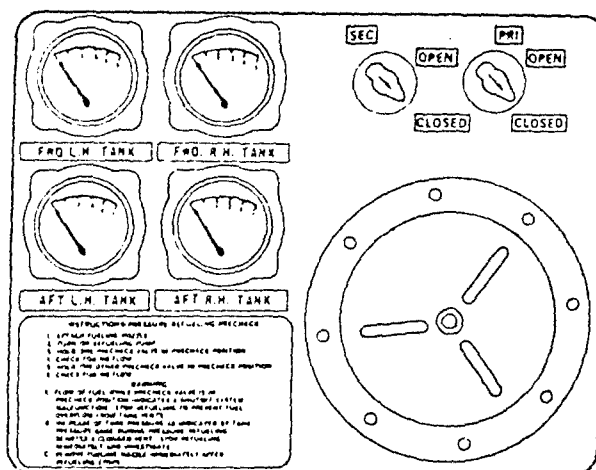
GROUND REFUELING PANEL CH-53E and MH-53E
