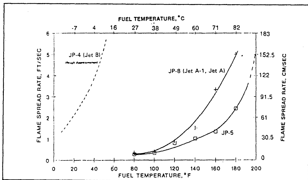
Figure 6-2. Flame Spread Rate Versus Fuel Temperature.
