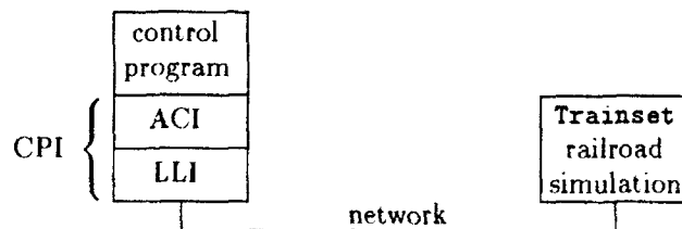
Figure 3.1: Communication interface layers.
