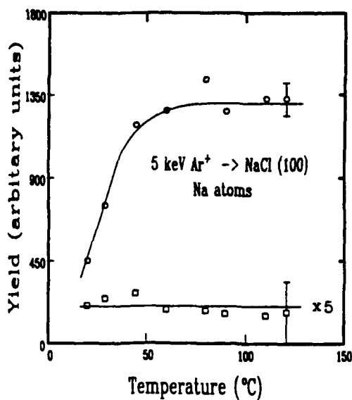
Fig. 3. The dependence of the thermal (O) and the collisional (□) contributions on the target temperature. The solid line is drawn only as an aid to the eye.
