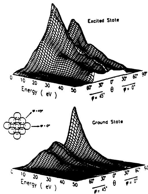
Fig. 1. Energy- and angle-resolved distributions of Rh atoms in the {}^4F_{7/2} excited state and {}^4F_{9/2} ground state, ejected from 5 keV \text{Ar}^+ ion bombarded Rh(100). The data correspond to ejection along \varphi=0^\circ ( \langle 100 \rangle ) and \varphi=45^\circ ( \langle 110 \rangle ) crystallographic directions, as defined in the inset. Due to the symmetry of the surface and the angular resolution ( \Delta\varphi=\pm 10^\circ ), the results represent the behavior over \sim 50\% of all space. Both plots are normalized to the maximum intensity peaks.
