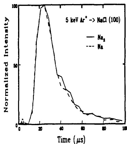
Fig. 5. The TOF distributions of \text{Na}_2 dimers (solid line) and Na atoms (dashed line) emitted from ion-bombarded \text{NaCl}(100) at 130^\circ\text{C} .
