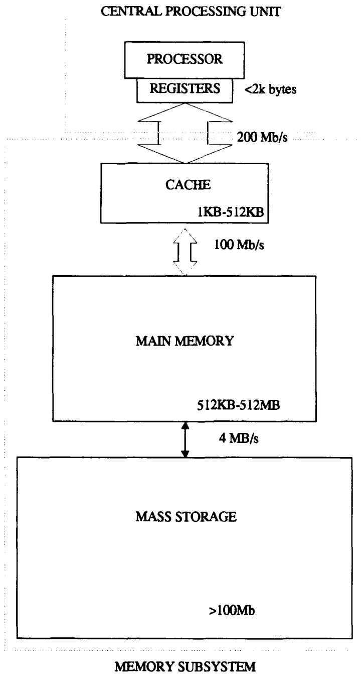
Figure 1: Memory Hierarchy
