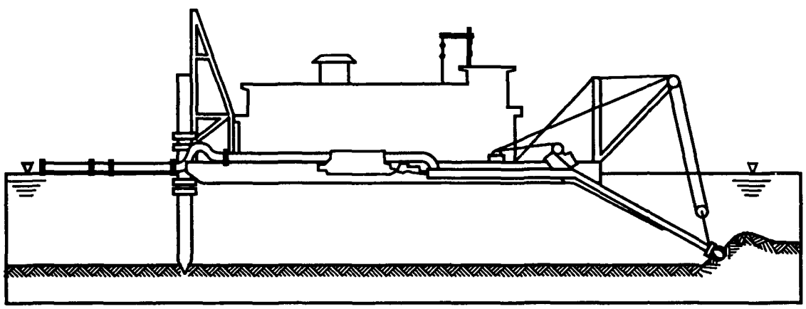
b. Cutterhead pipeline dredge
