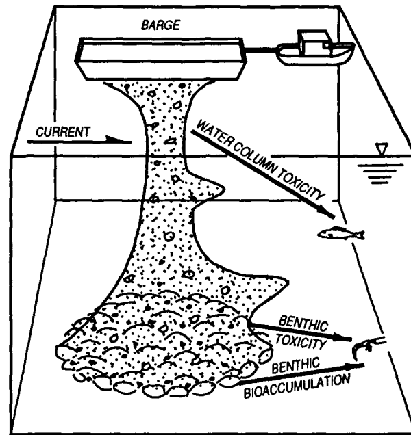
Figure 4-1. Contaminant Pathways for Open-water Disposal
