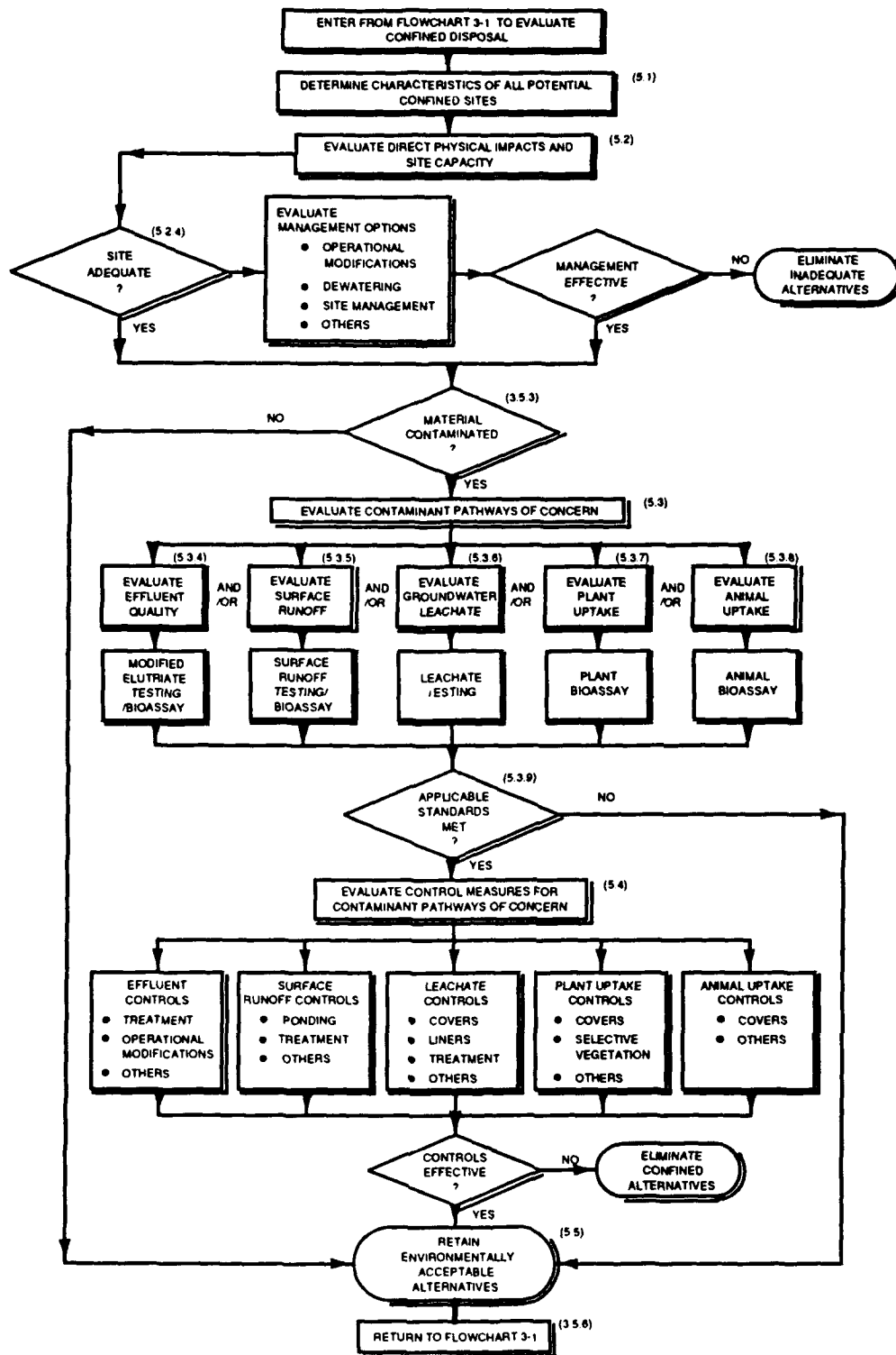
Flowchart 3-3. Framework for Testing and Evaluation for Confined (Diked) Disposal
