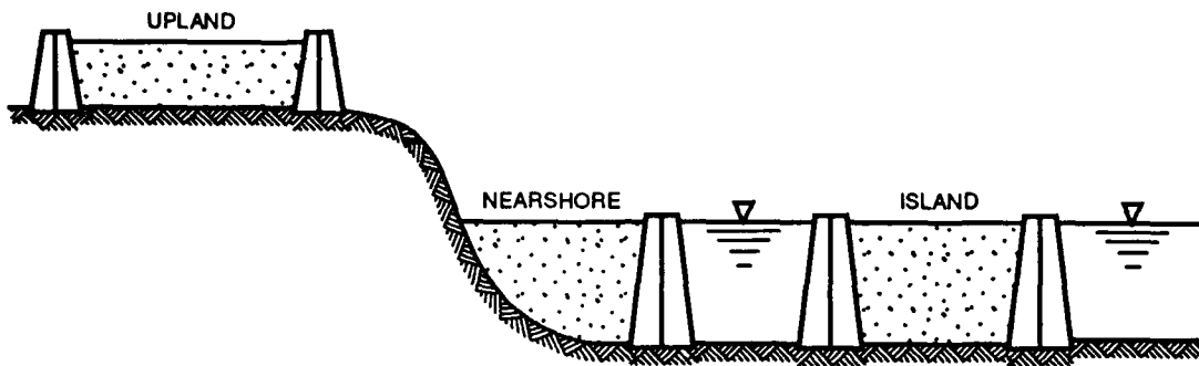
Figure 2-3. Upland, Nearshore, and Island CDFs
