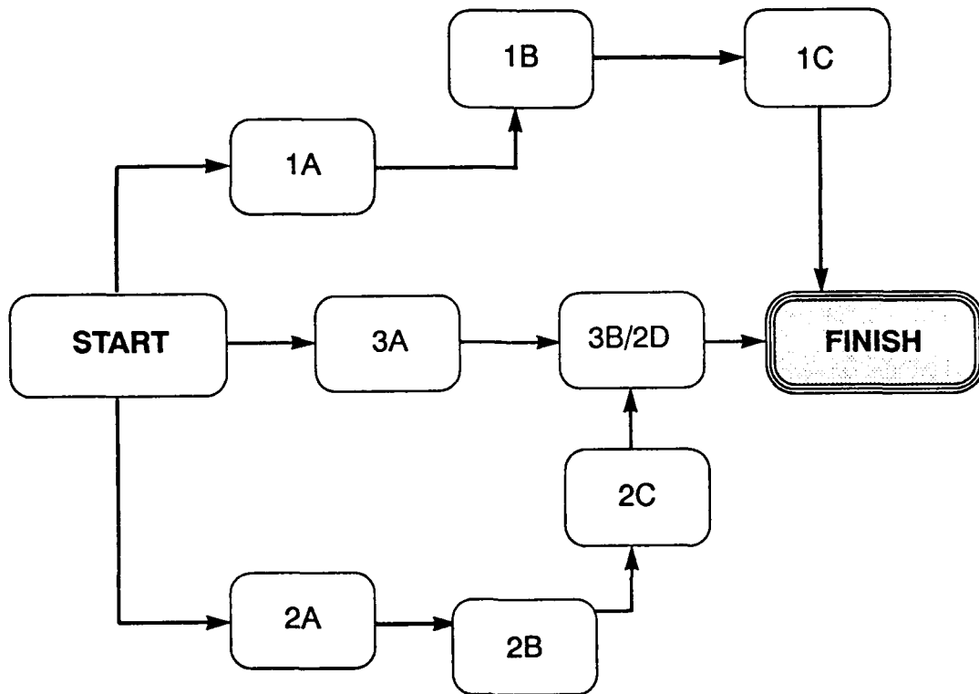
Figure 34. Arrow Diagram
