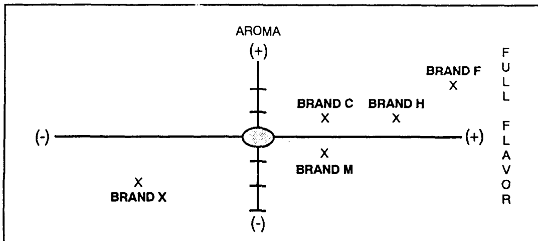
Figure 51. Perception Map
