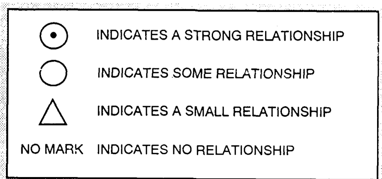
Figure 17. Quality Relationship
