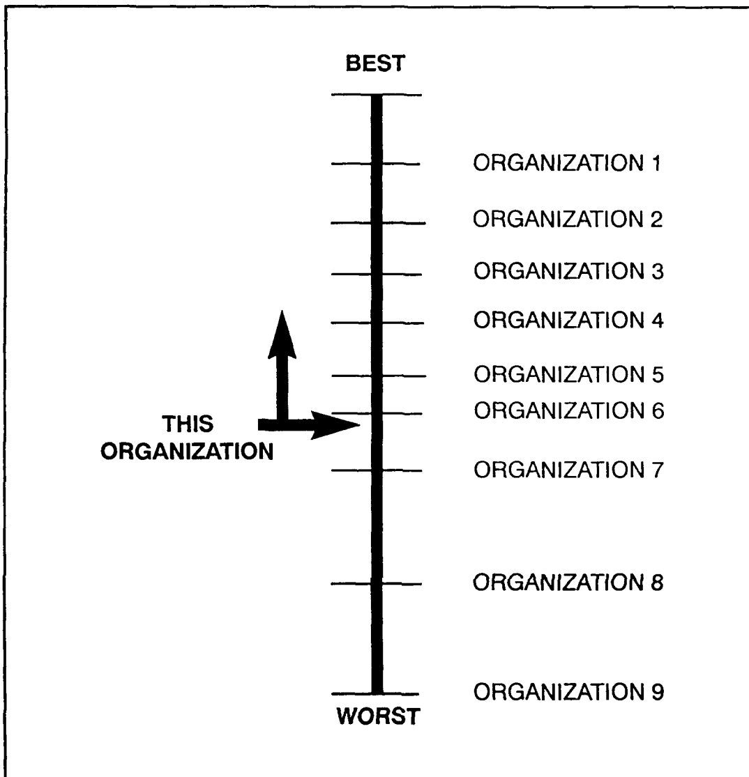
Figure 35. Benchmark
