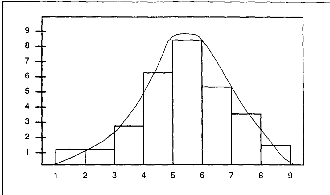
Figure 43. Histogram
