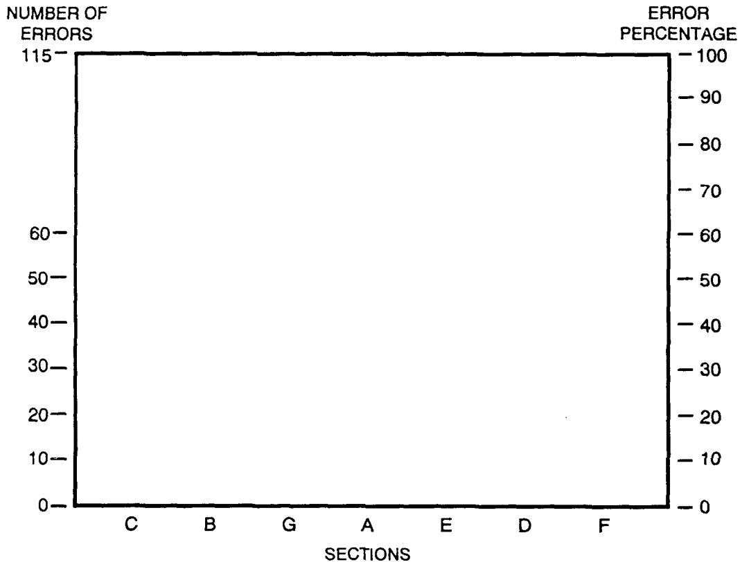
Figure 48. Pareto Frame
