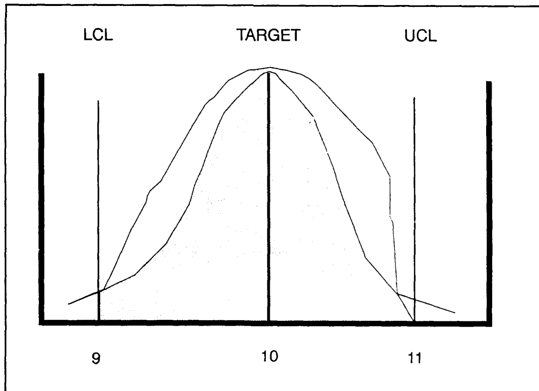
Figure 10. Loss Function
