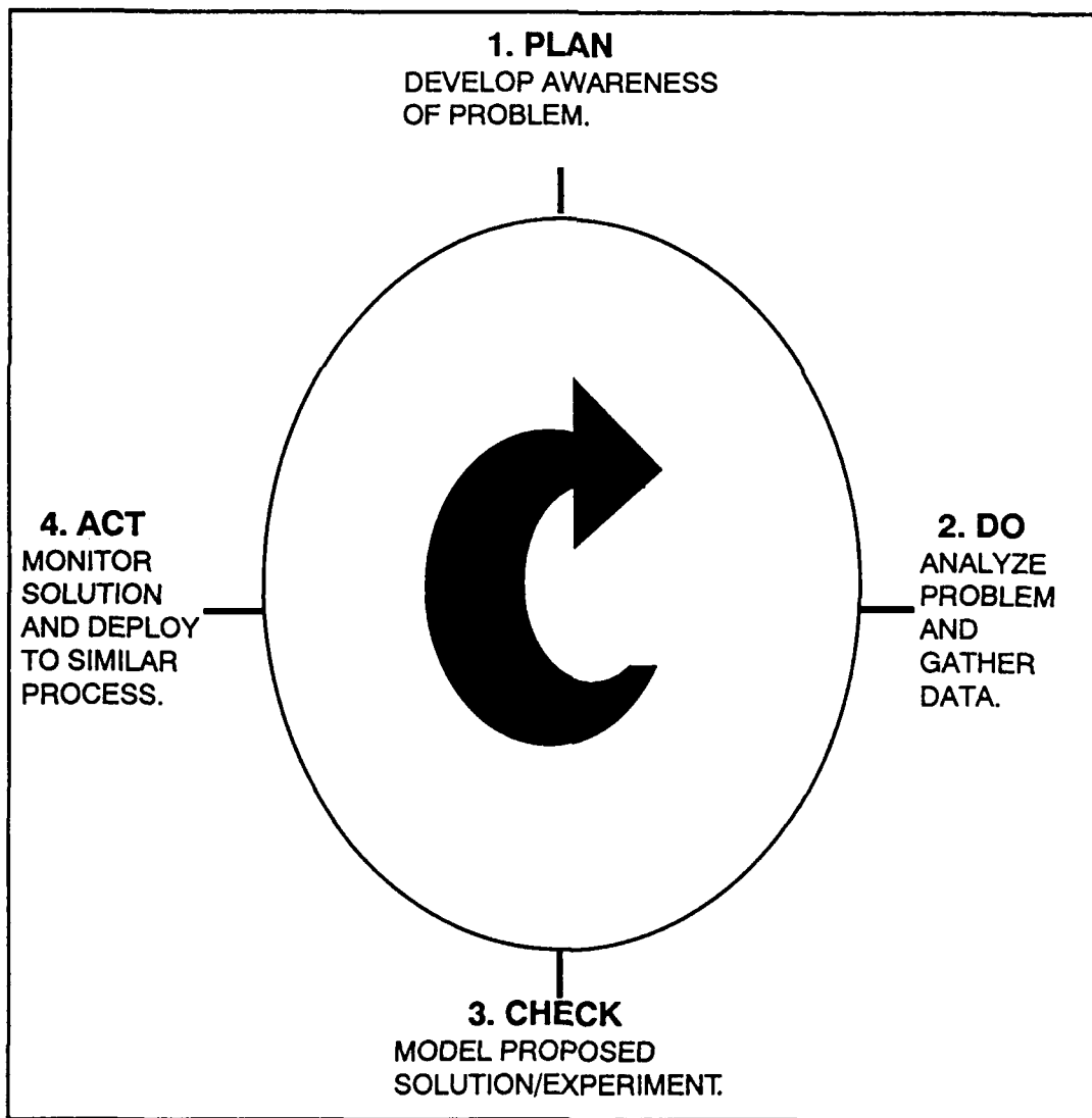
Figure 53. Plan-Do-Check-Act Cycle
