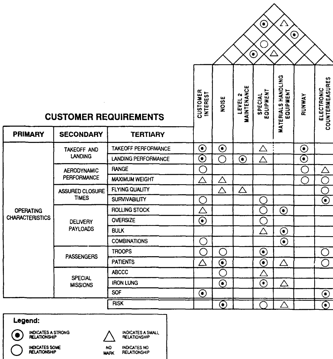
Figure 20. Correlation Matrix
