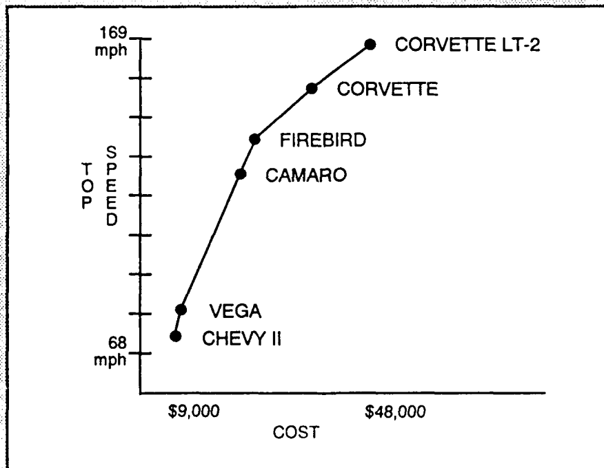
Figure 38. Correlation Chart
