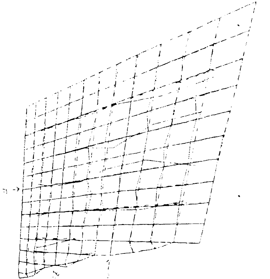
Figure 33. Combined Skin and Stiffener Mode Shape at 371.2 Hz
