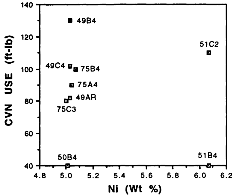
Figure 4.9 USE vs. Ni content 100KJ/in heat input
