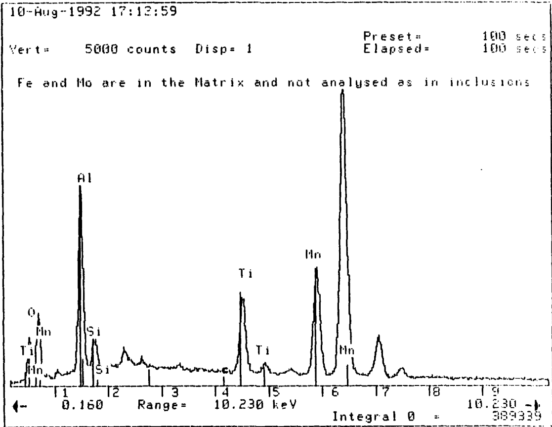
Figure 4.21 EDX Graph of 49B3-1. Typical of compositions of inclusions in ail samples
