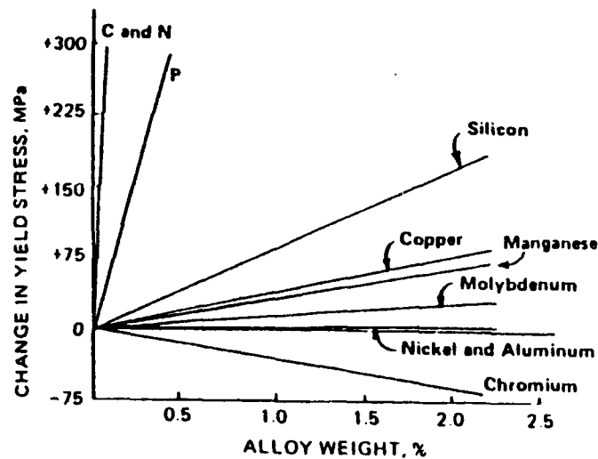
Figure 2.6 Hardening effect of elements in steel.
