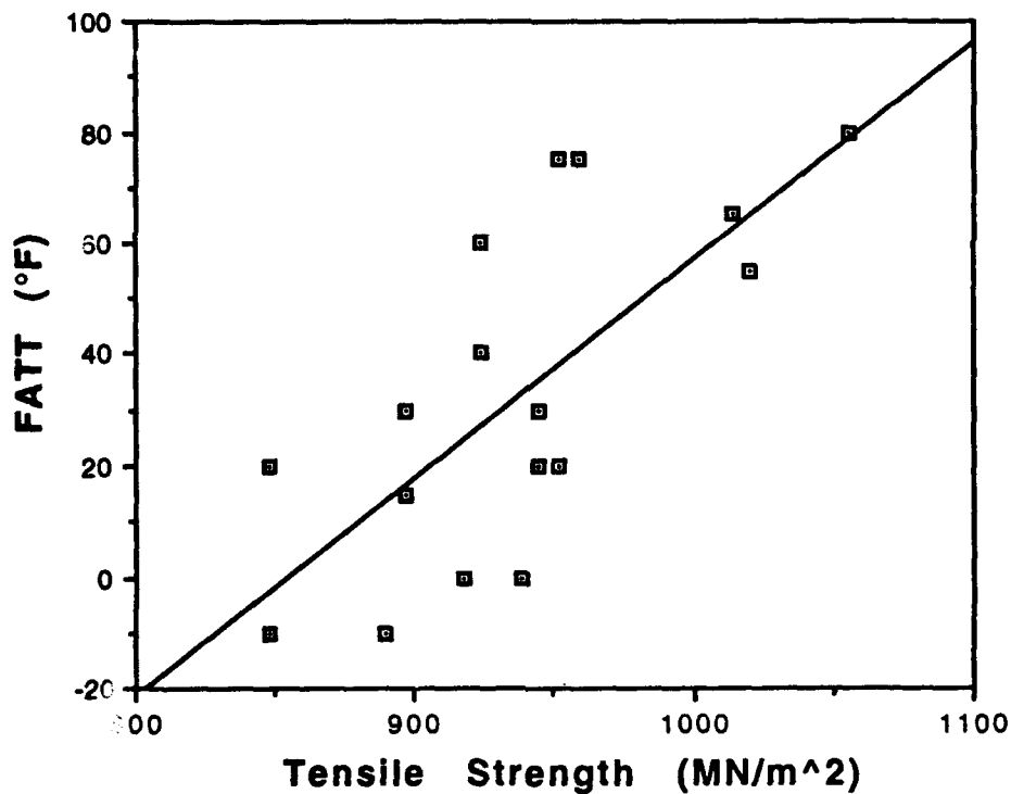
Figure 4.26 FATT vs. Tensile Strength for all data.
