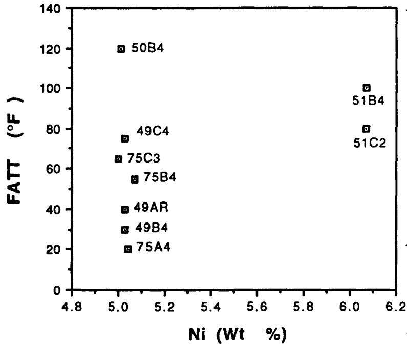
Figure 4.10 FATT vs. Ni content
