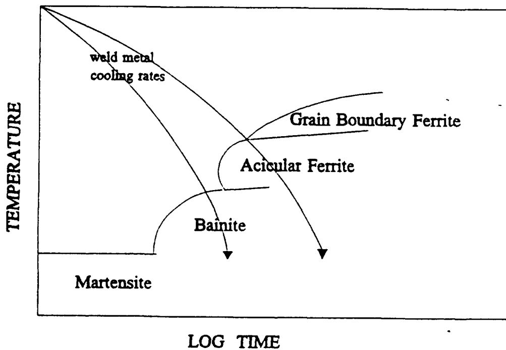
Figure 2.3 Continuous Cooling Transformation Curves. (McHale, P.F., 1991, p.12)
