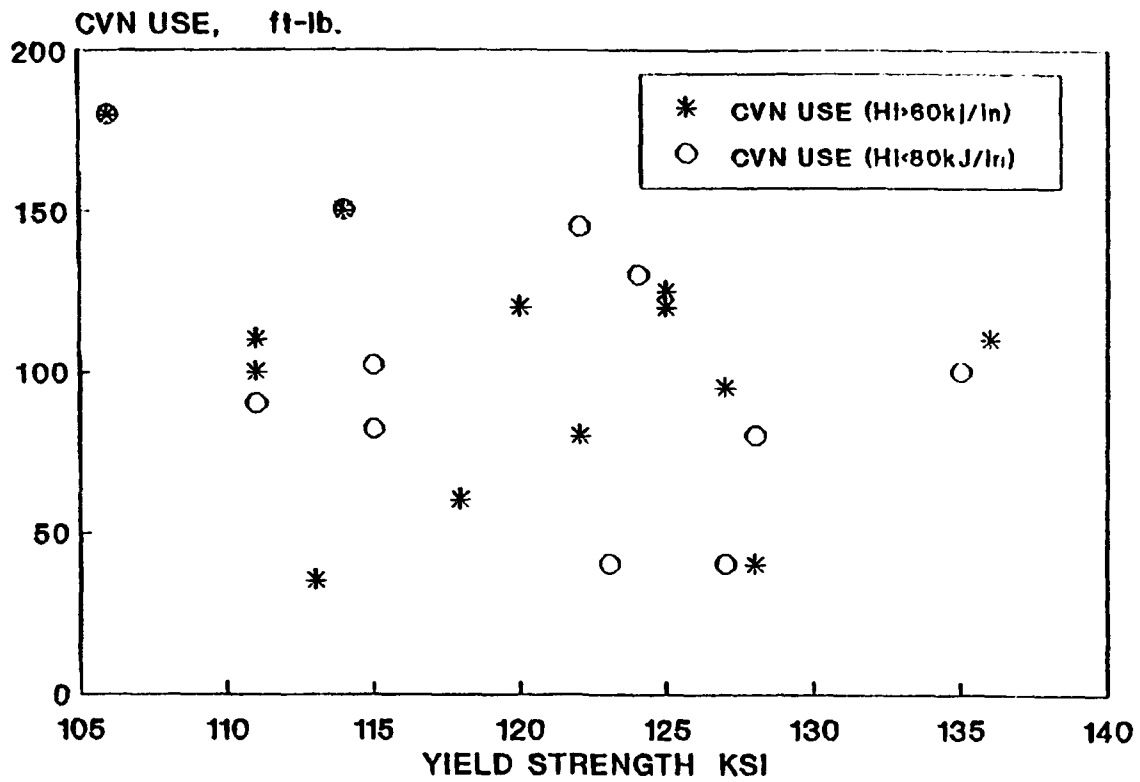
Figure 4.1 CVN USE vs. Yield Strength
