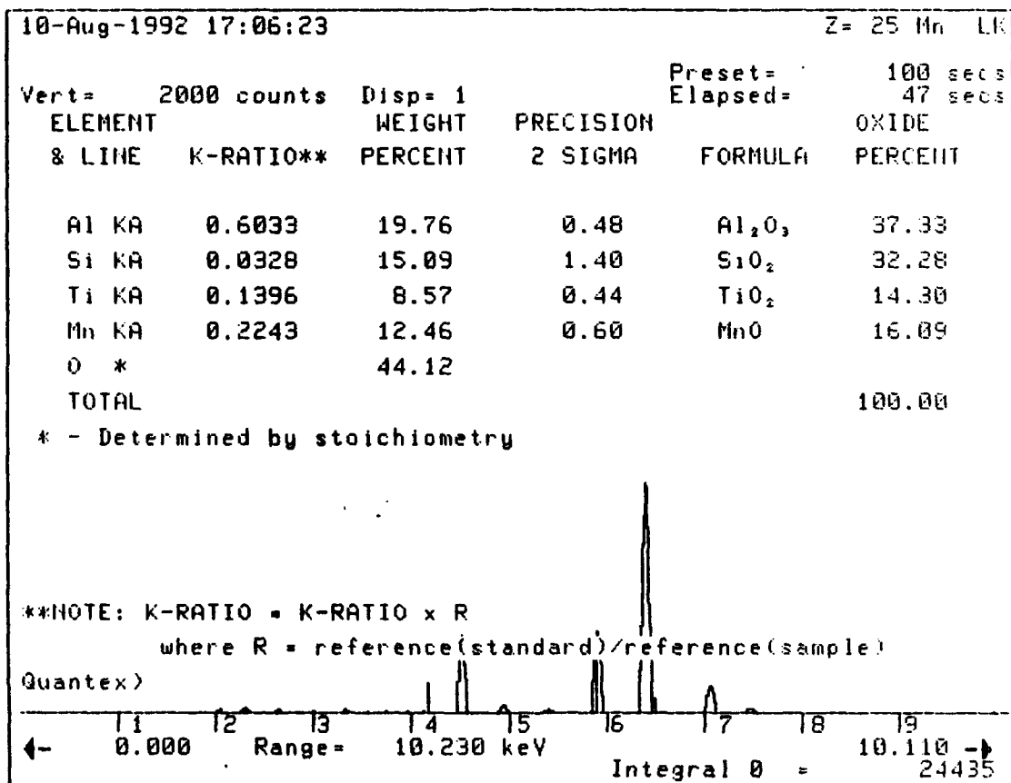
Figure 4.22 EDX Data of 49B3-1 Typical of compositions of inclusions in all samples
