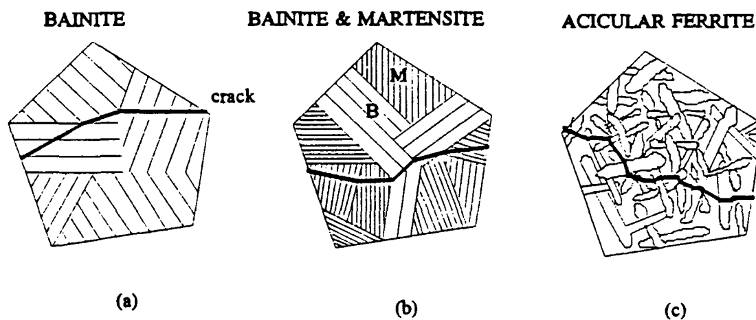
Figure 2.2 Dependence of crack propagation upon microstructure.
