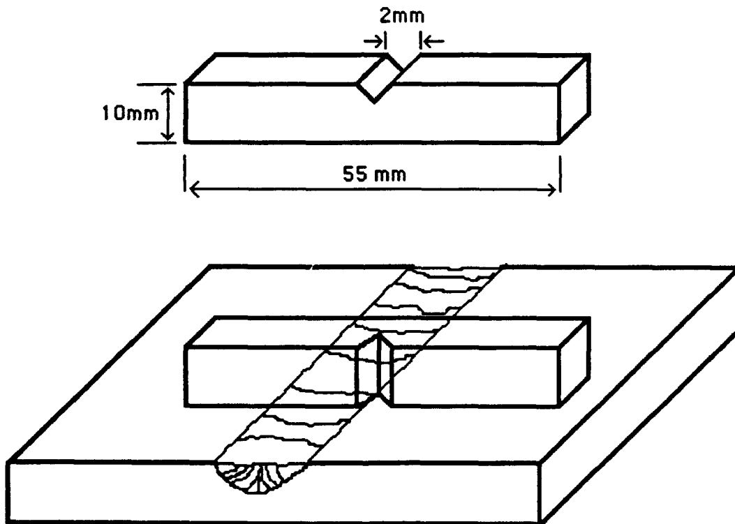
Figure 3.1 Charpy Weldment Sample Orientation
