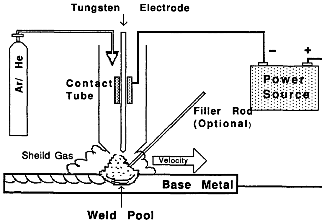
Figure 2.5 Tungsten Inert Gas (TIG) Welding Process
