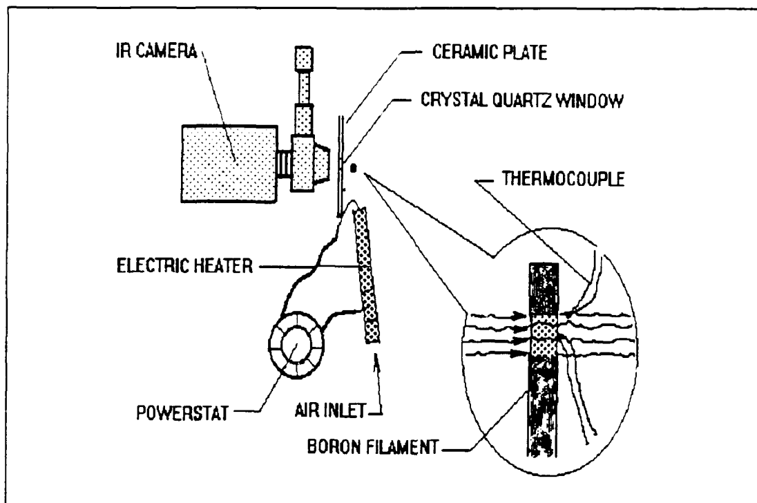
Figure 5. The initial layout of experimental apparatus
