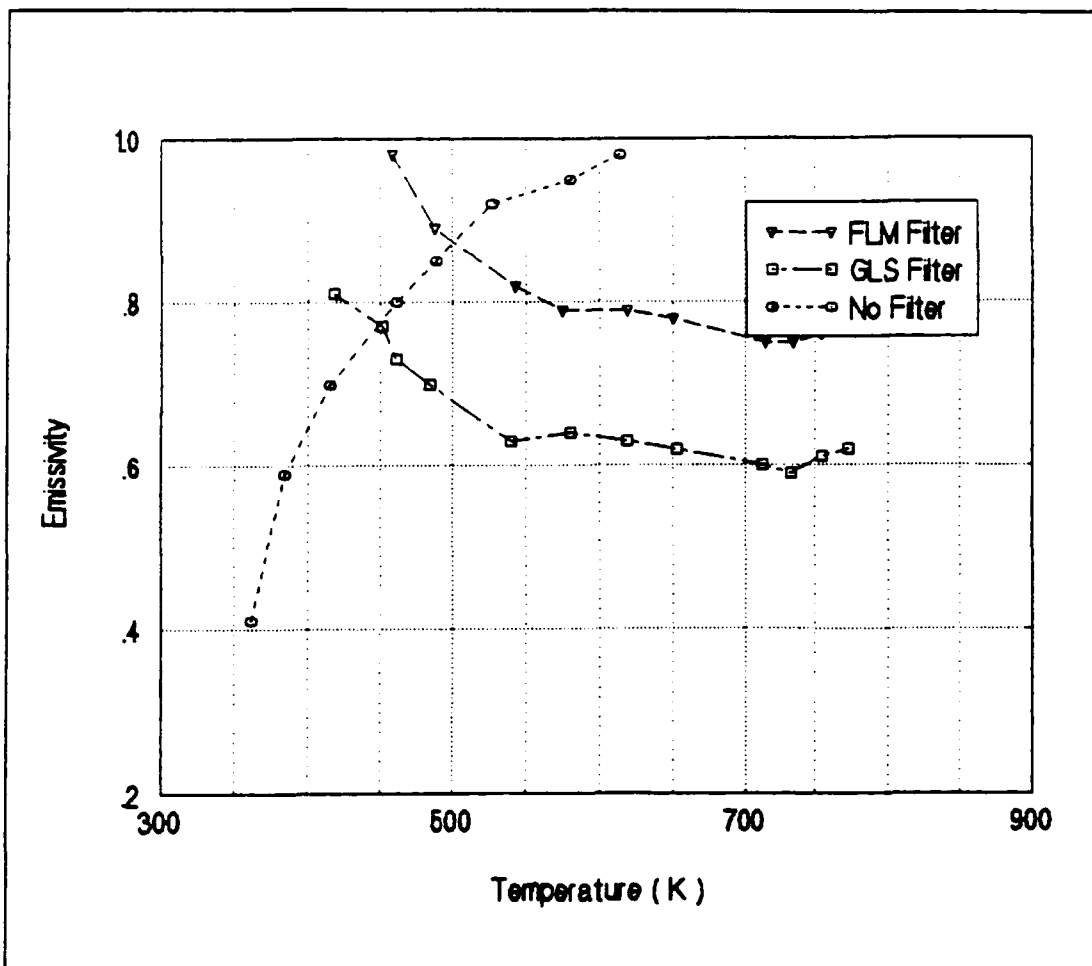
Figure 8. The averaged emissivity of boron oxide in 2 \mu\text{m} - 5 \mu\text{m} band in the longitudinal direction (rough surface)
