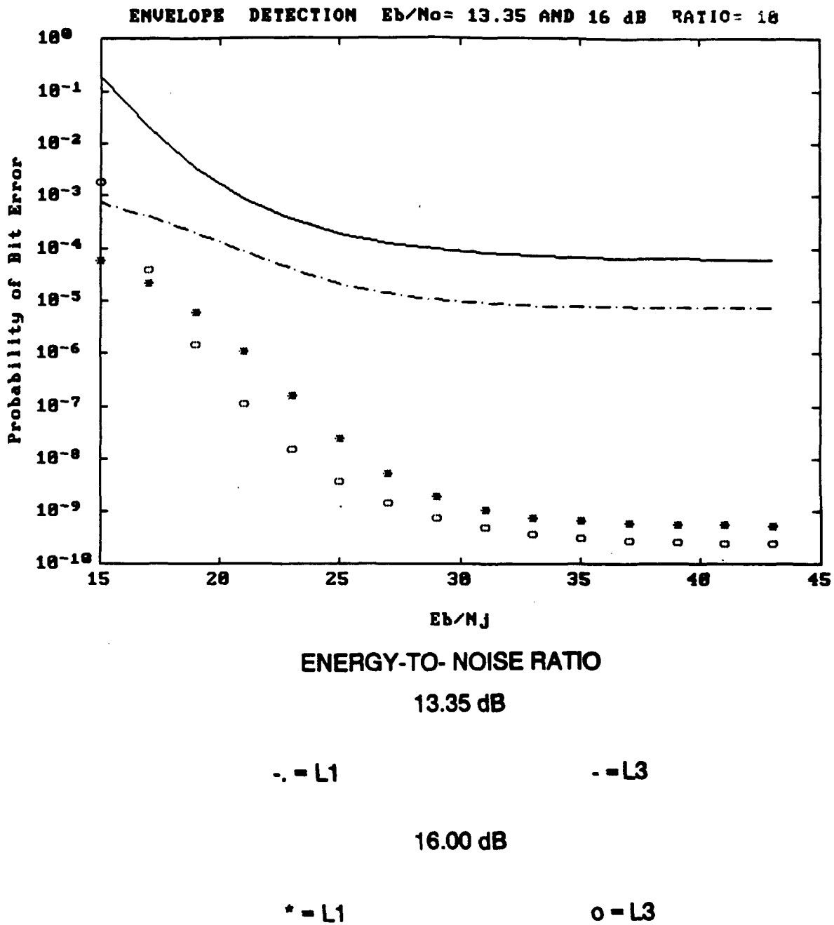
Figure 3.20. Comparison of the Performance of a FFH/NCBFSK/RS Receiver with Envelope detection, where Direct to Diffuse RATIO=10, E_b/N_o=13.35 , and 16 dB and worst L=1 and 3.
