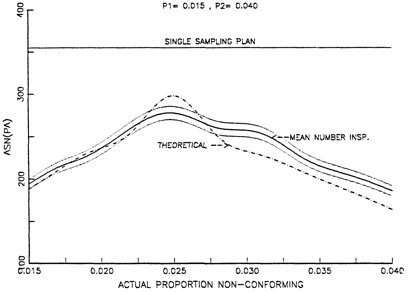
Figure 34 - ASN CURVE , PLAN SET III , CURVE B
