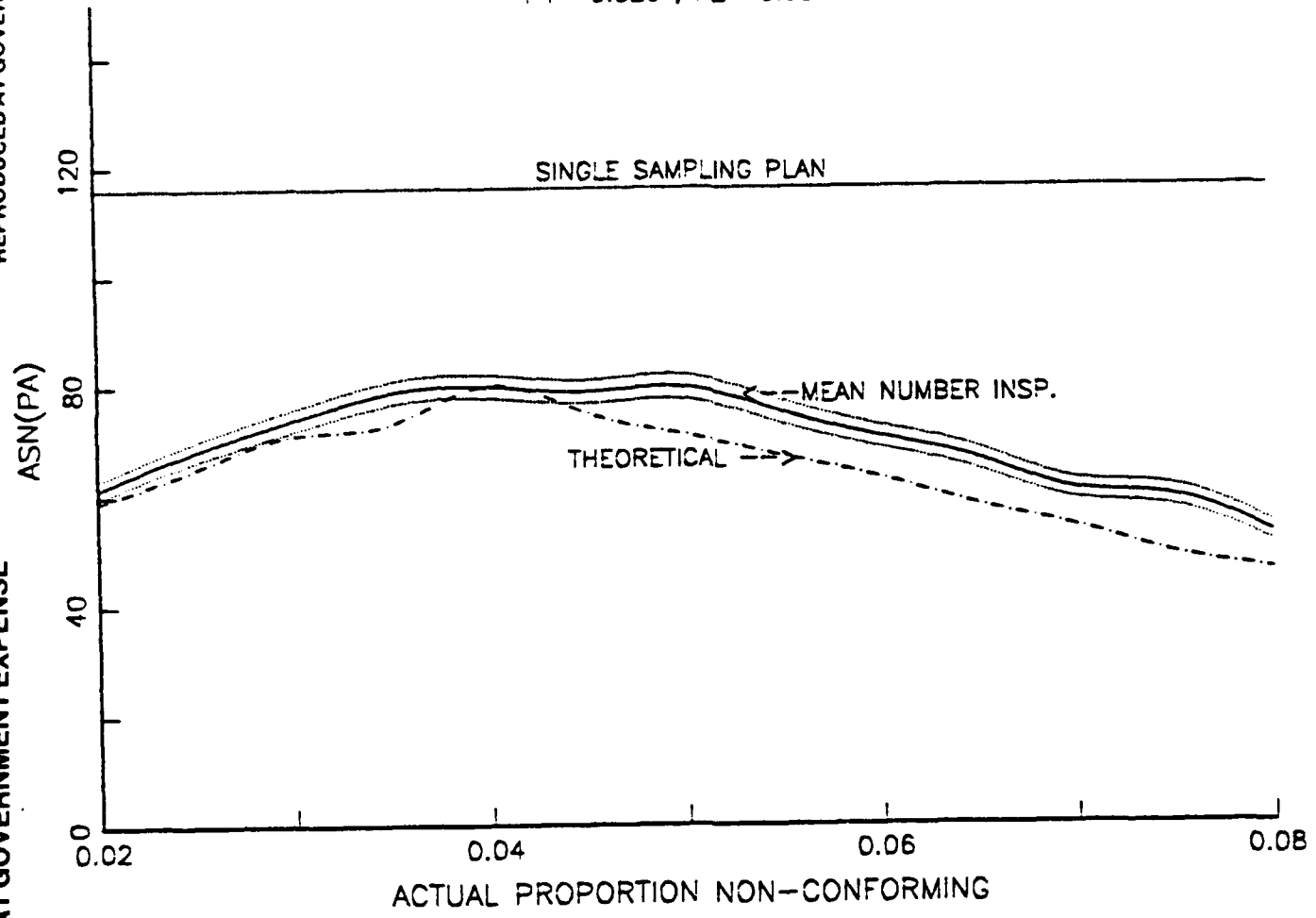
Figure 43 - ASN CURVE , PLAN SET IV , CURVE F
