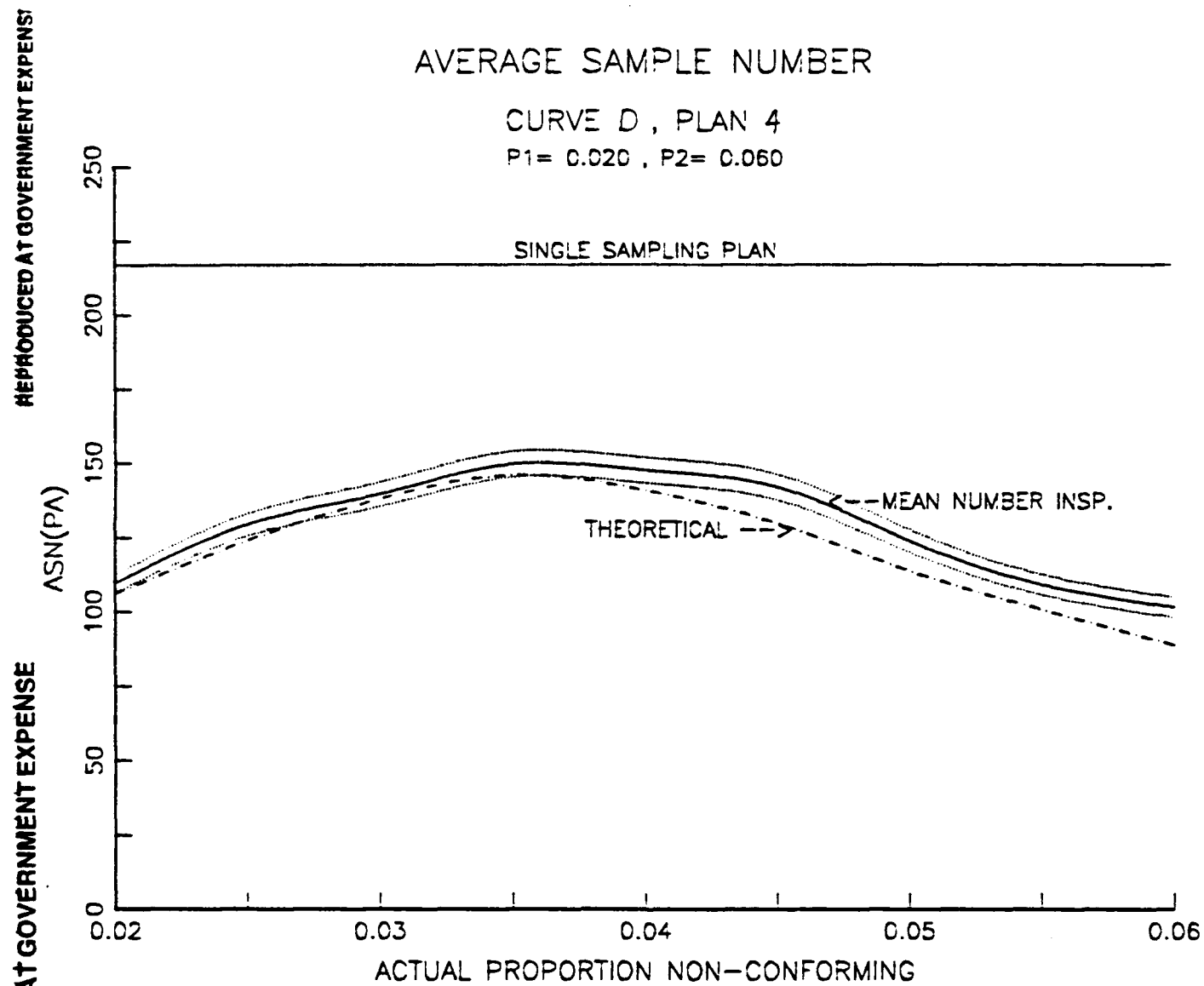
Figure 41 - ASN CURVE , PLAN SET IV , CURVE D
