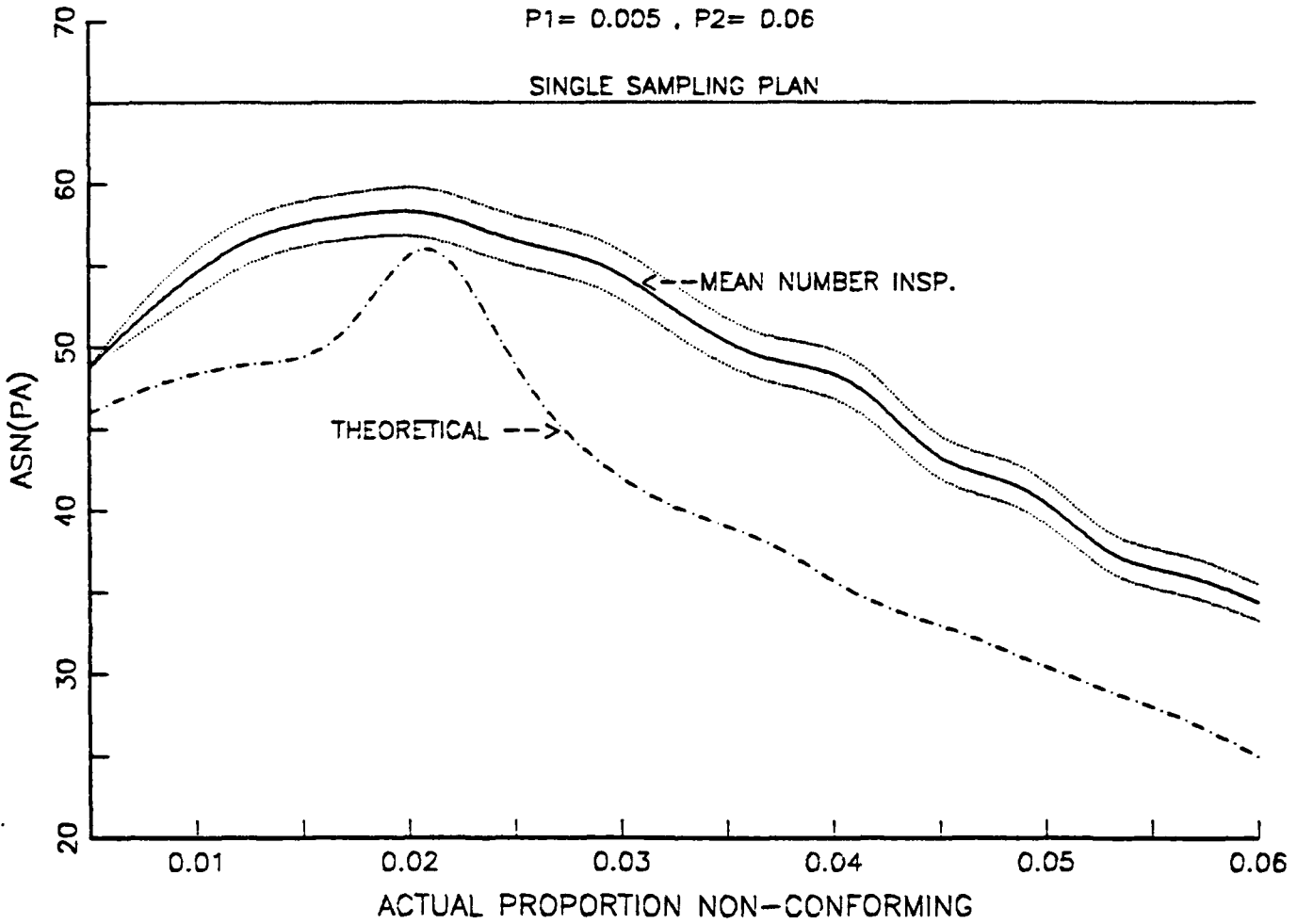
Figure 25 - ASN CURVE, PLAN SET I, CURVE F
