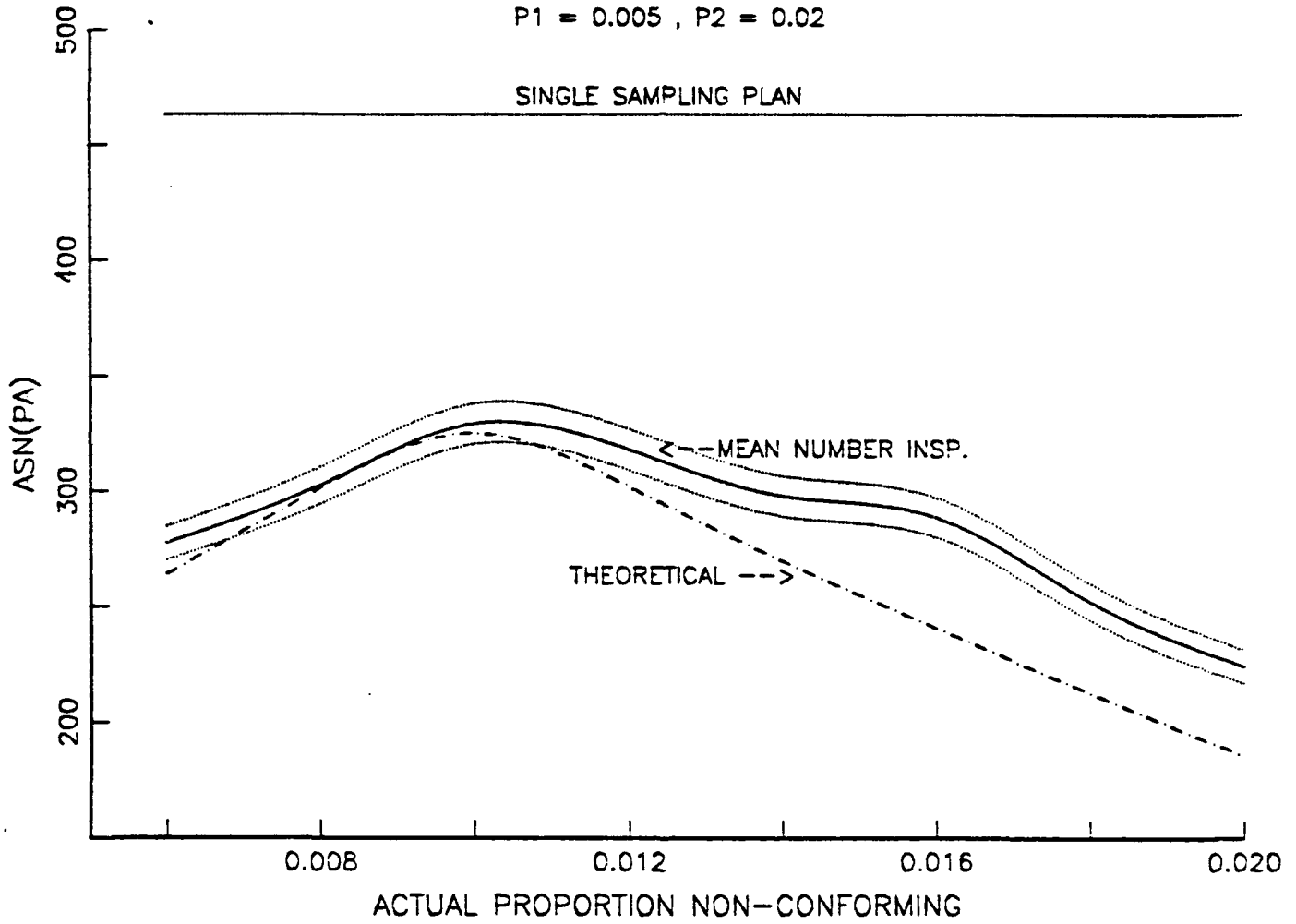
Figure 21 - ASN CURVE , PLAN SET I , CURVE B
