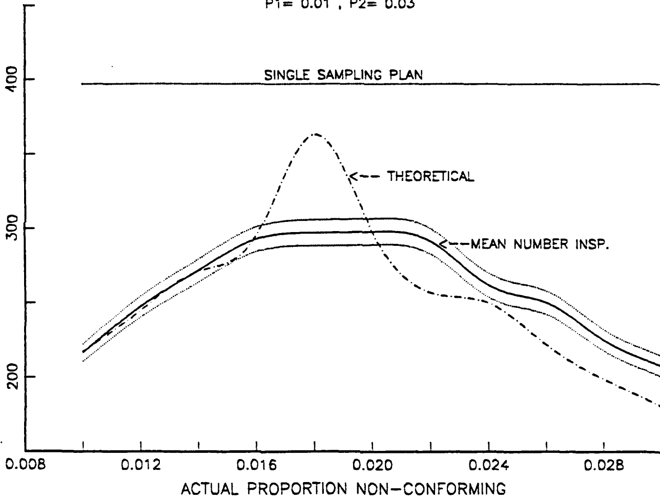
Figure 27 - ASN CURVE , PLAN SET II , CURVE A
