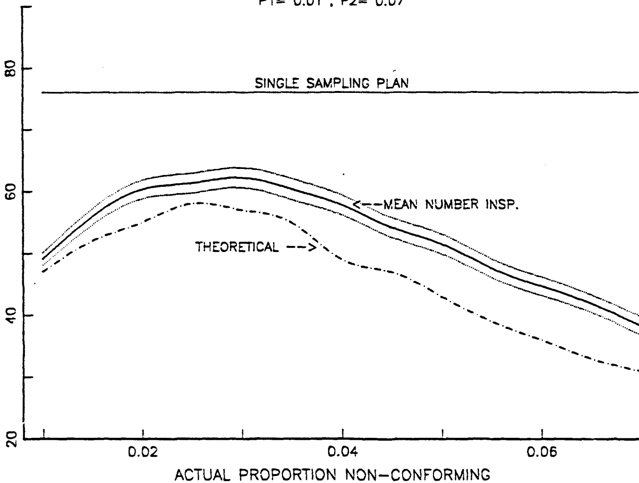
Figure 31 - ASN CURVE , PLAN SET II , CURVE E
