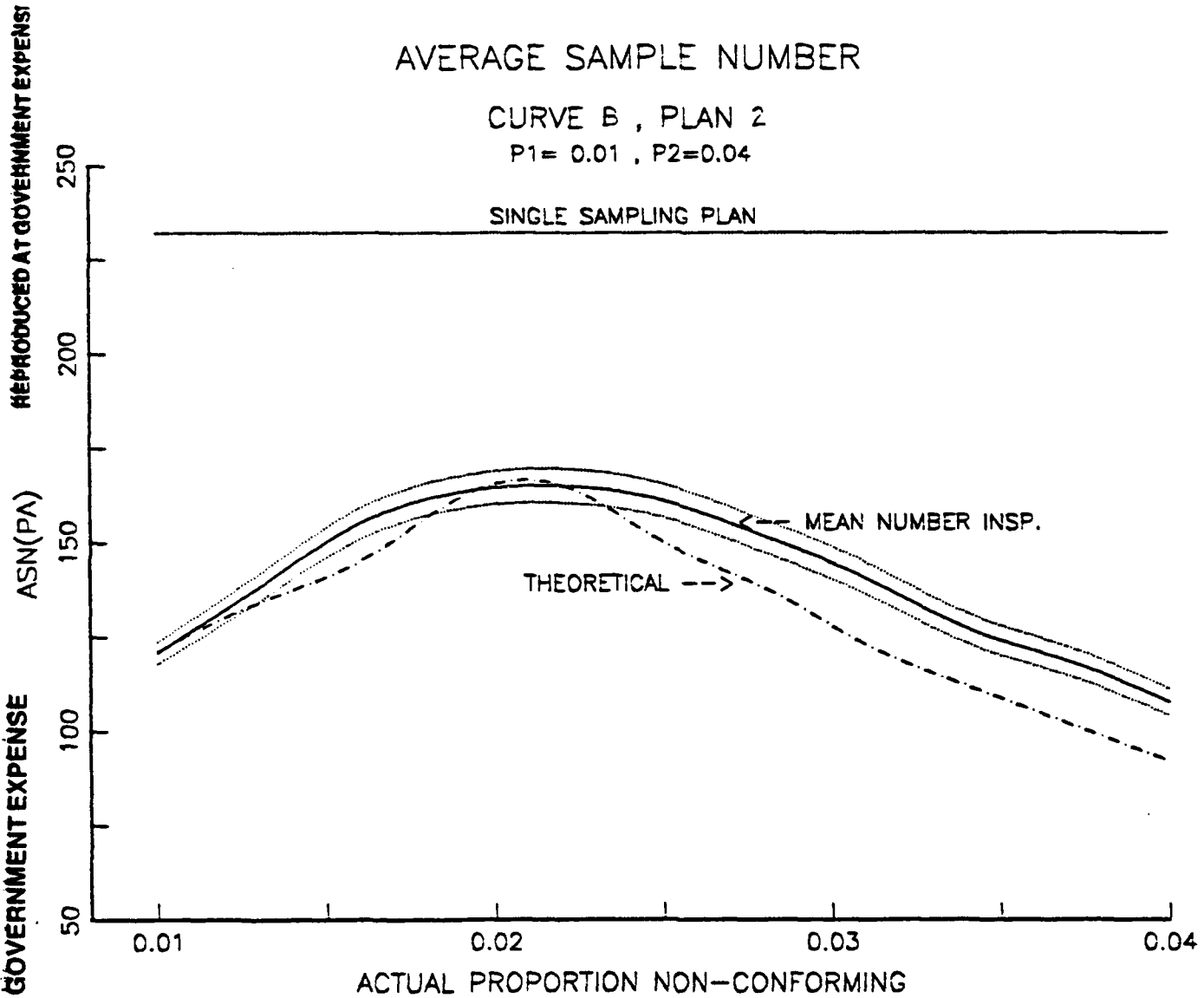
Figure 28 - ASN CURVE , PLAN SET II , CURVE B
