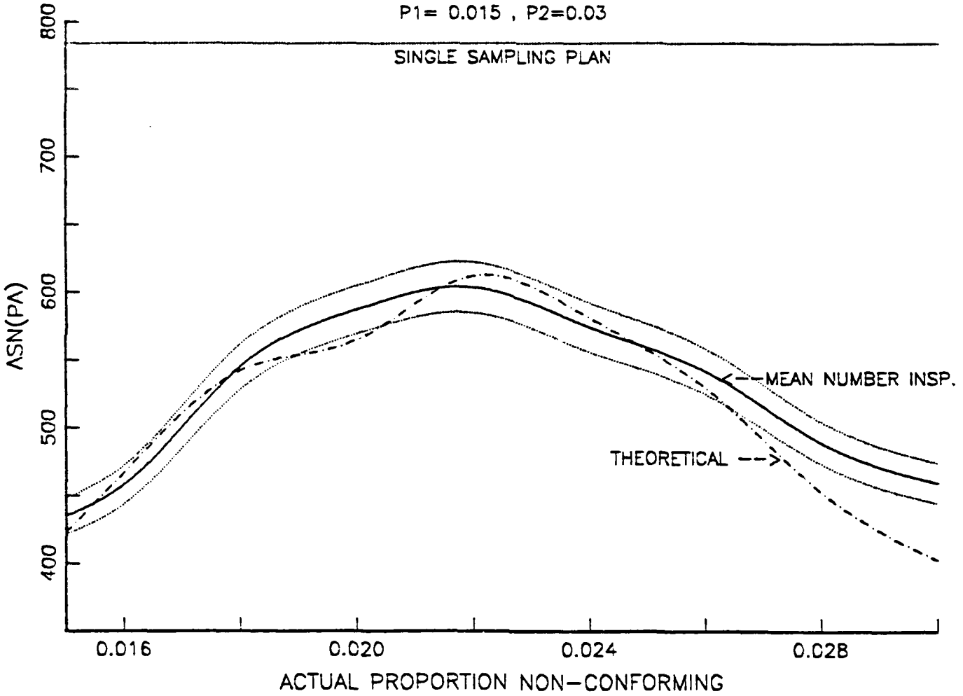
Figure 33 - ASN CURVE , PLAN SET III , CURVE A
