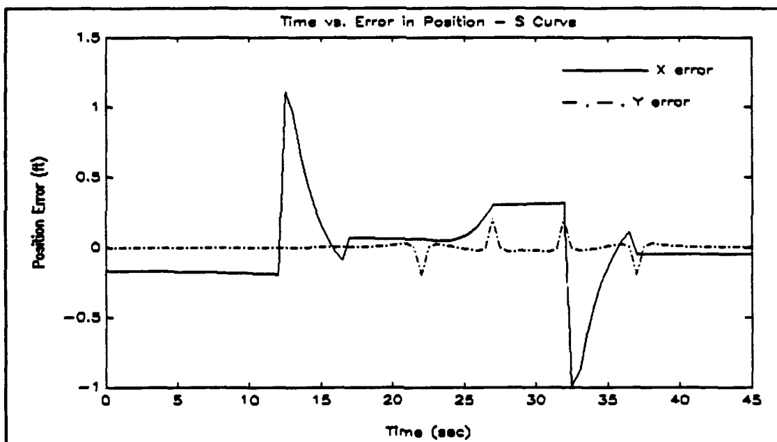
Figure 5.1: X and Y smoothed estimate error with old maneuver detection scheme
