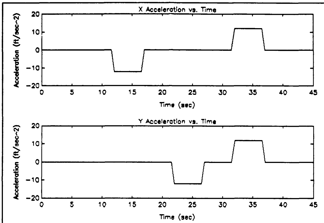
Figure 5.2: Target's acceleration
