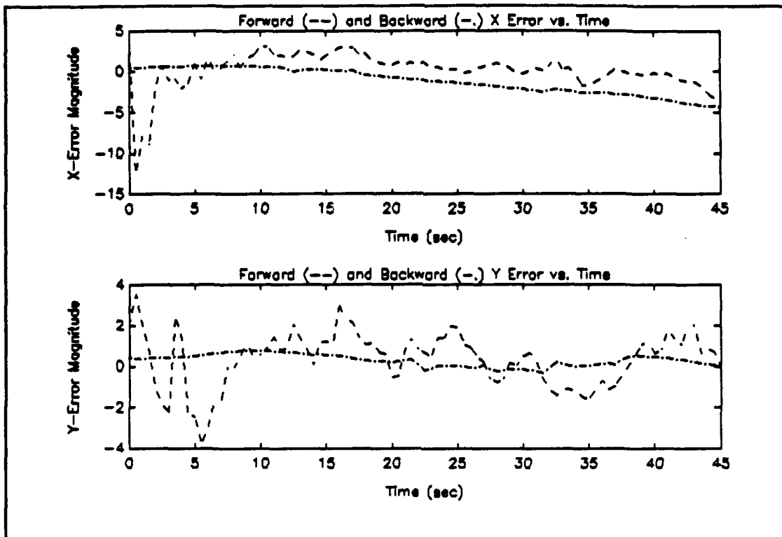
Figure 5.6: Error for noisy track
