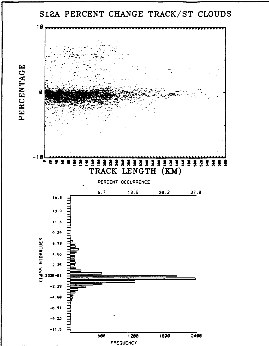
Figure A3. Scatterplot and Histogram for DPC S12A Stratus Track/Cloud.
