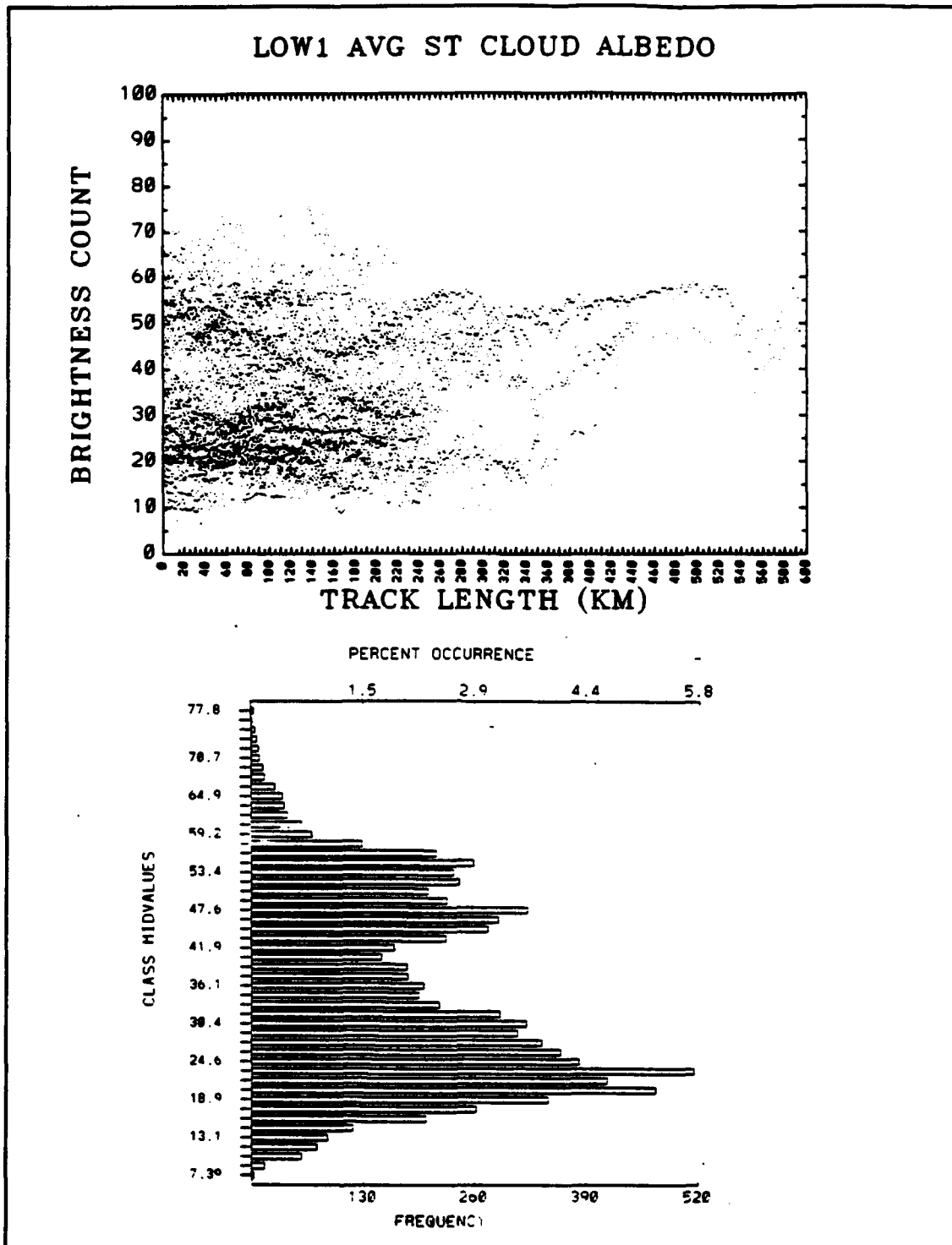
Figure 7. Scatterplot and Histogram for LOW1 Stratus Regime.
