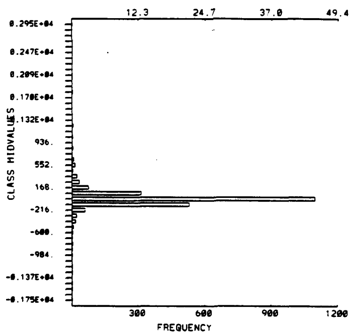
Figure A24. Scatterplot and Histogram for DPC T45 Broken Stratus Track/Cloud.
