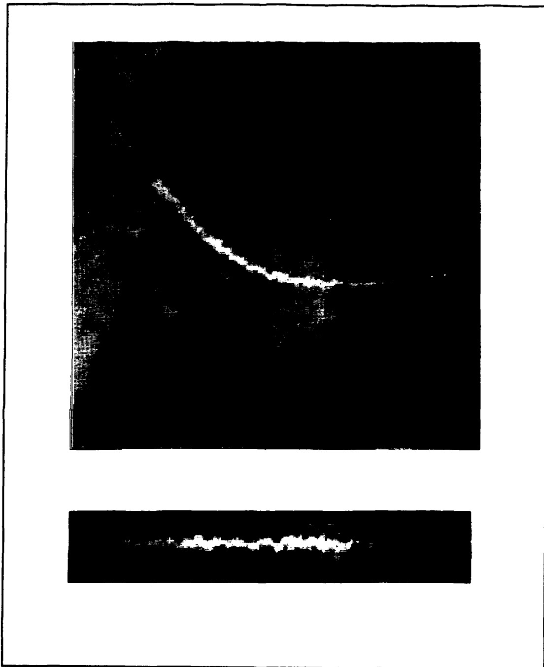
Figure 4. Raw and Linearized, Weighted Average Versions of the Same Ship Track.
