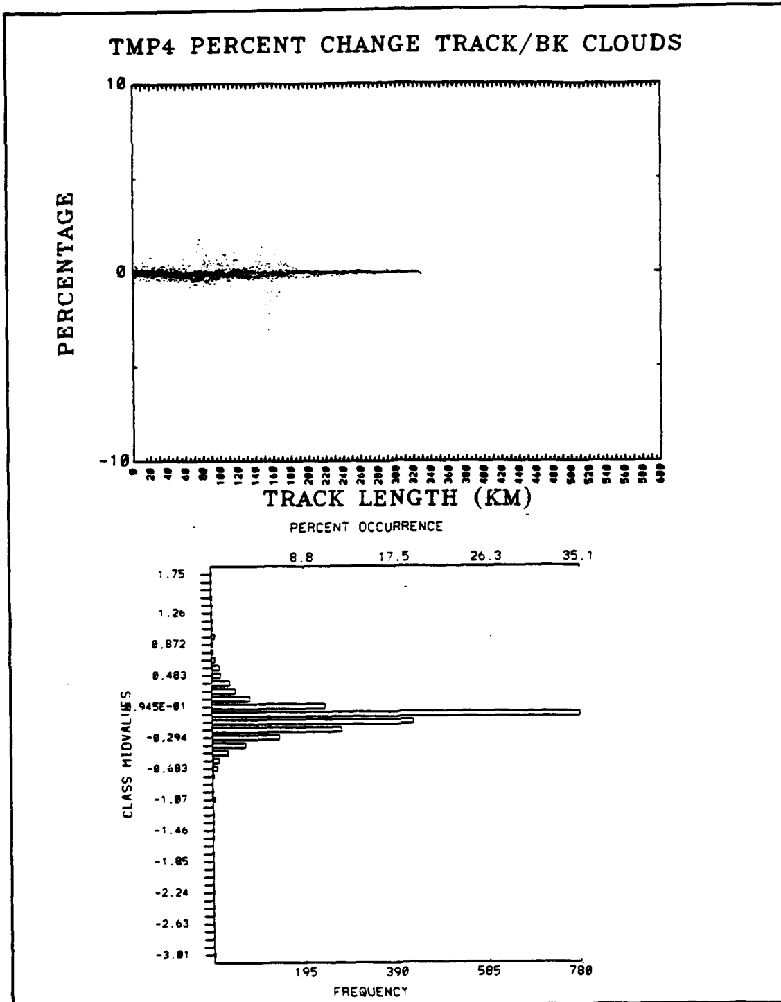
Figure A15. Scatterplot and Histogram DPC TMP4 Broken Stratus Track/Cloud.
