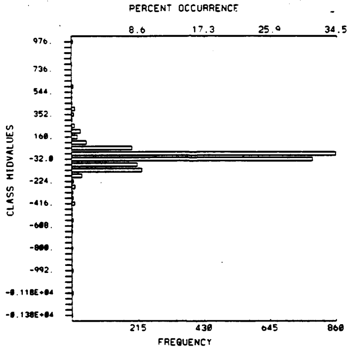
Figure A27. Scatterplot and Histogram for DPC T45 Cumulus Track/Cloud.
