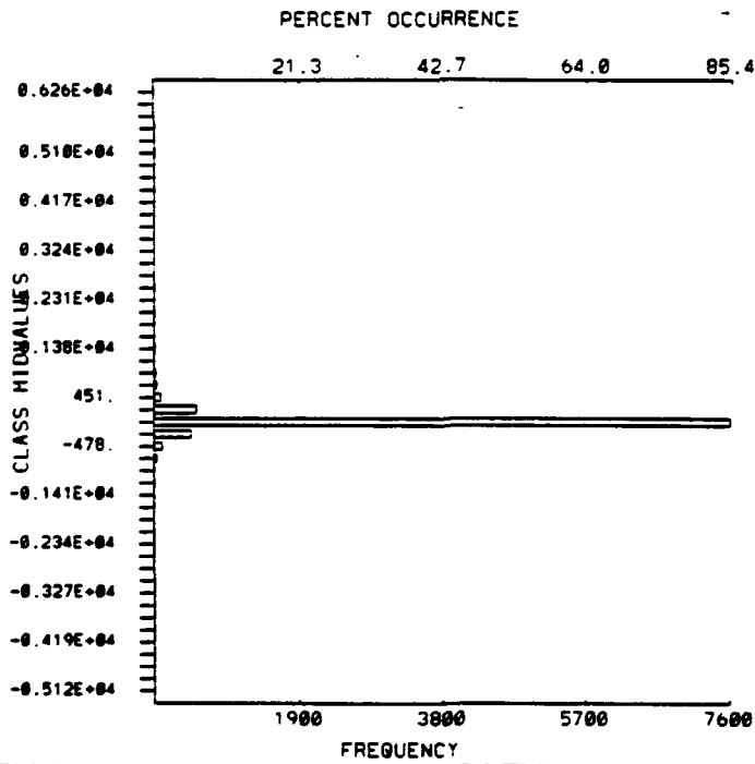
Figure A21. Scatterplot and Histogram for DPC T45 Stratus Track/Cloud.
