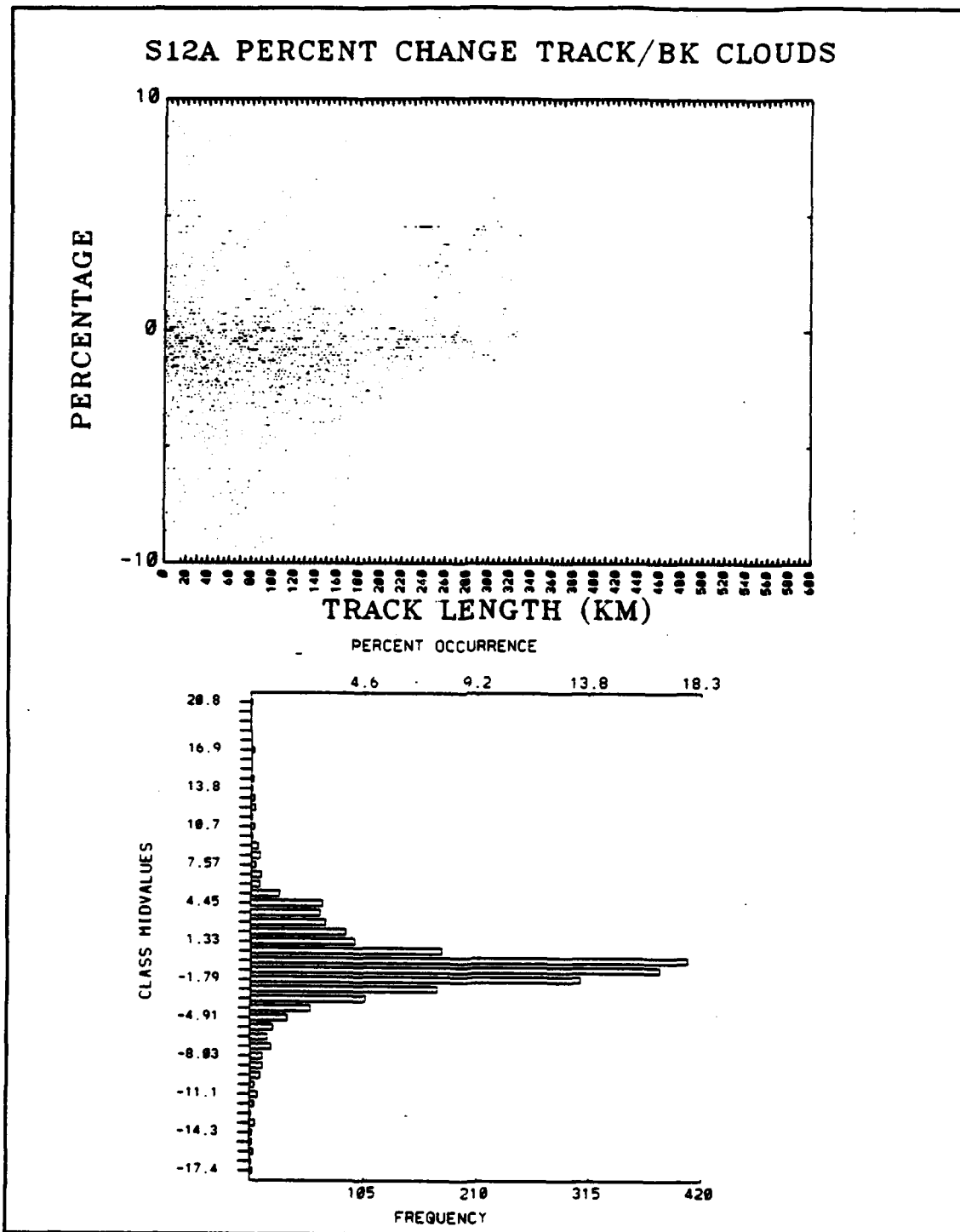
Figure A6. Scatterplot and Histogram for DPC S12A Broken Stratus Track/Cloud.
