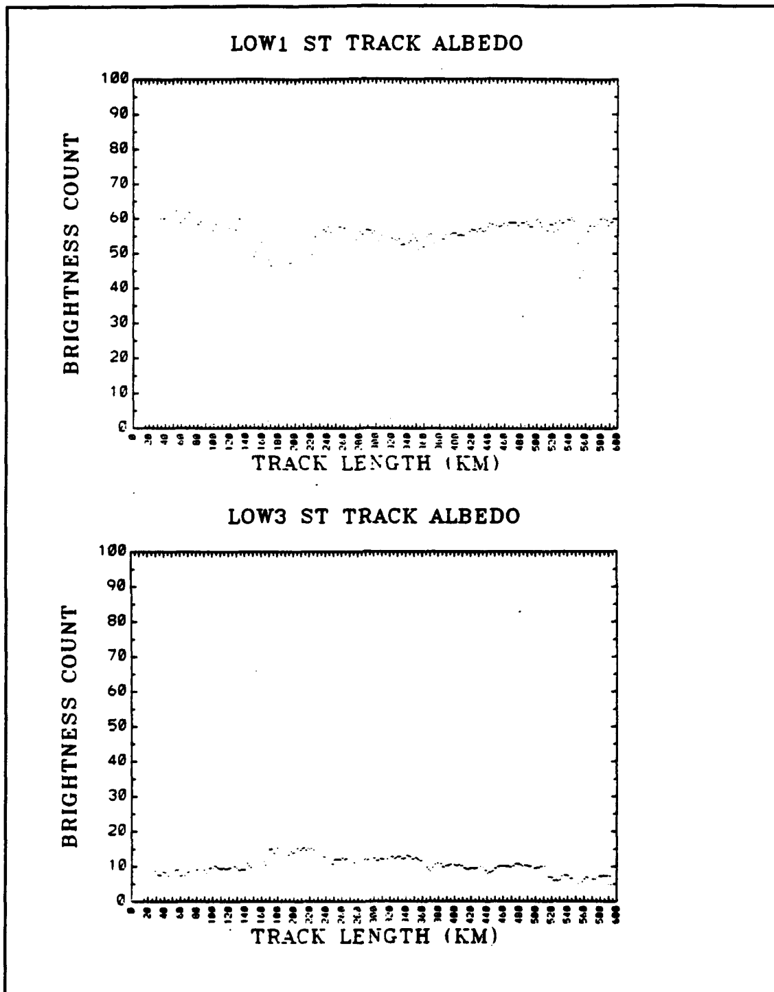
Figure 6. LOW1 and LOW3 Scatterplots Depicting a Single Ship Track.
