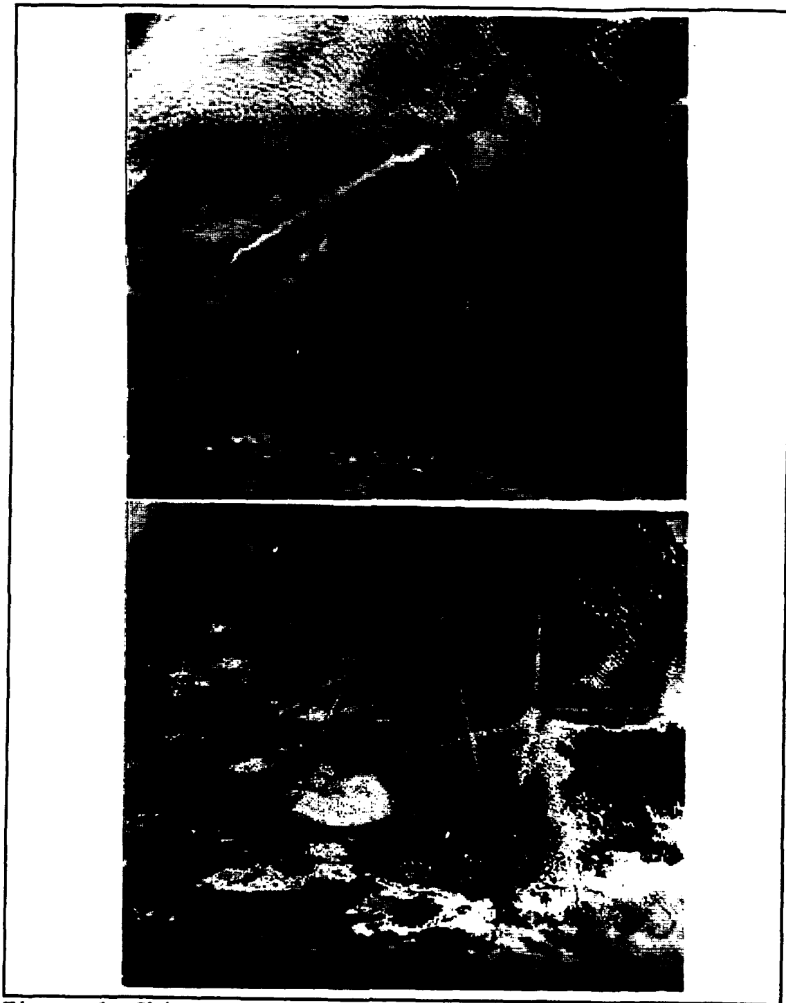
Figure 1. Ship Tracks in Satellite Imagery at .63 \mu\text{m} , (top), and 3.7 \mu\text{m} , (bottom).
