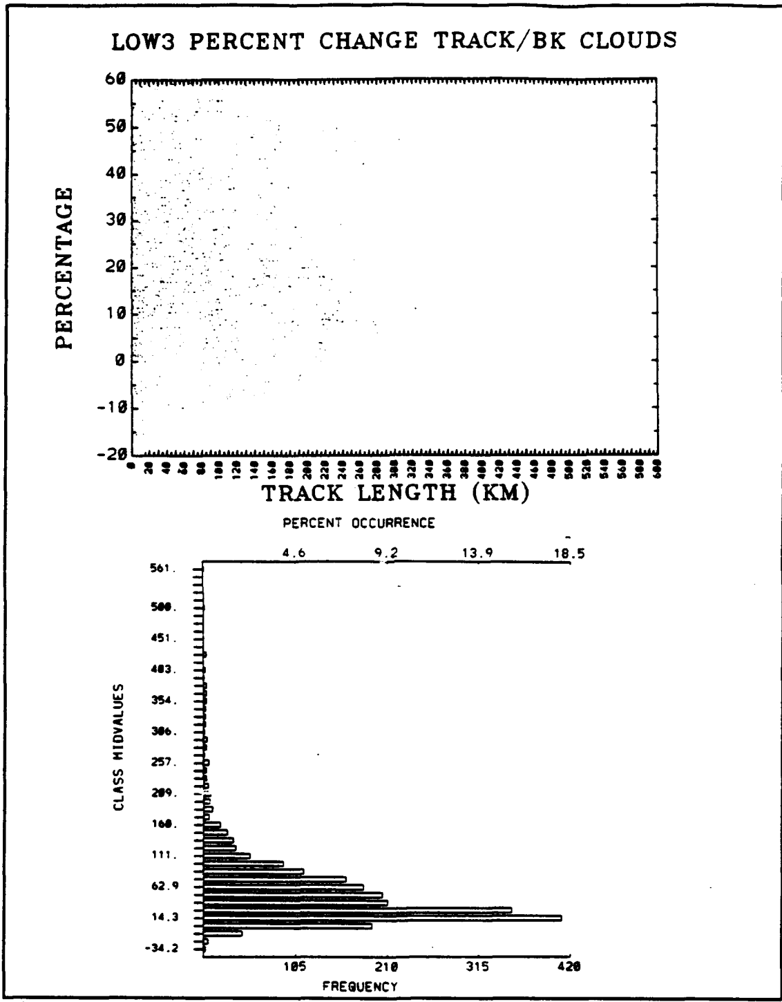
Figure 18. Scatterplot and Histogram for DPC LOW3 Track/Cloud.
