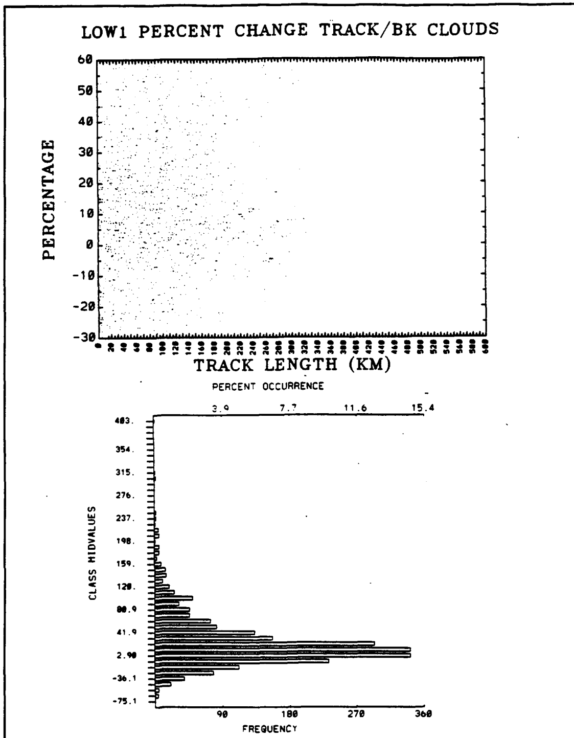
Figure 15. Scatterplot and Histogram for DPC LOW1 Track/Cloud.
