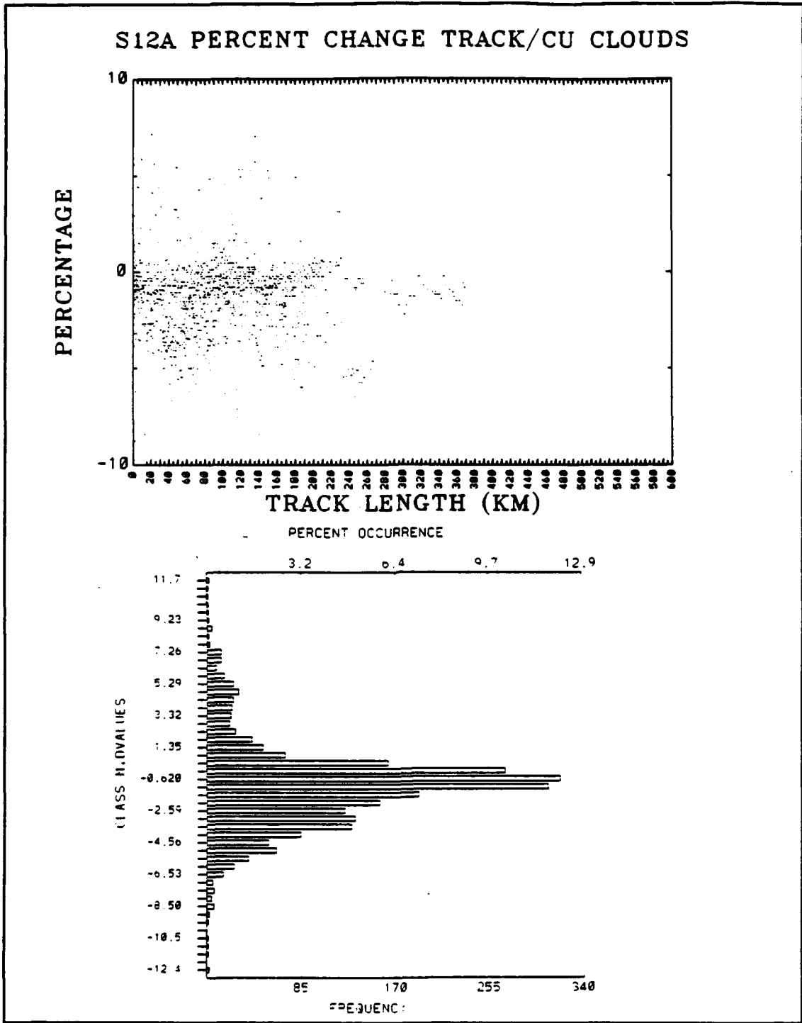
Figure A9. Scatterplot and Histogram for DPC S12A Cumulus Track/Cloud.
