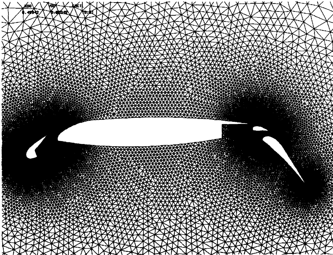
Figure 12 a) Unstructured Triangular Mesh Generated About a Four Element Airfoil Configuration by the Present Algorithm before the Application of Mesh Smoothing. (Number of Vertices = 21232, Number of Triangles = 41781) (Global View )
