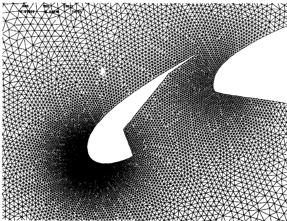
Figure 12 c) Unstructured Triangular Mesh Generated About a Four Element Airfoil Configuration by the Present Algorithm before the Application of Mesh Smoothing. (Number of Vertices = 21232, Number of Triangles = 41781) (Close Up of Leading Edge Slat)
