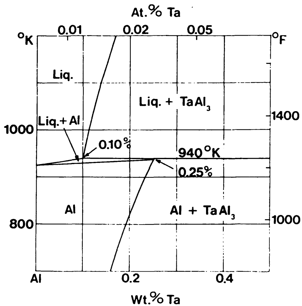
FIGURE 10: The phase diagram of Al-Ta. Note
