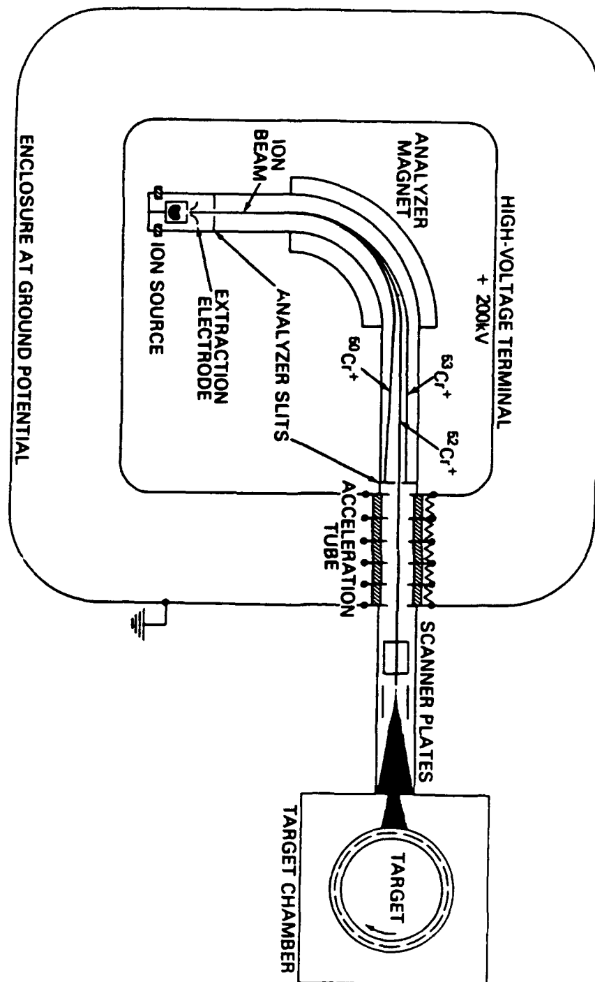
FIGURE 9: A schematic of the Ion Implantation process.
