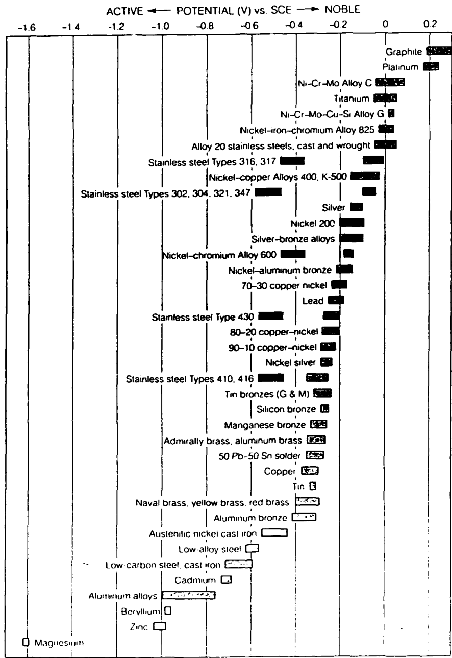
FIGURE 7: Galvanic Series showing the range of E_{corr} for various metals and alloys in seawater.
