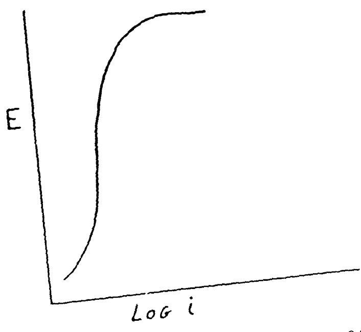
FIGURE 2: The location of the hydrogen evolution line is shown above the active region which causes the metal to spontaneously passivate
