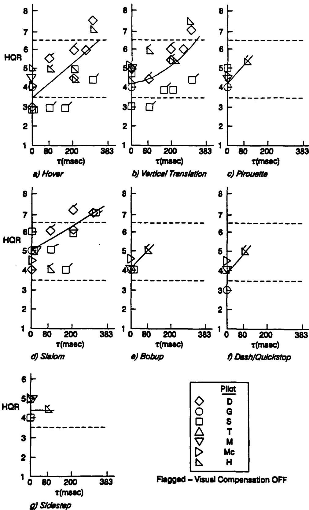
Figure 19. Time Delay Variations — Fixed Base
