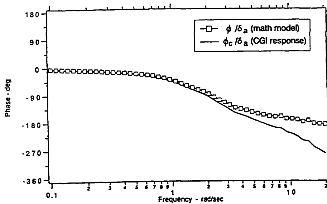
Figure B-5. Effect on CGI Response of Removing Visual Compensation Filter (Compare Fig. B-2b)
