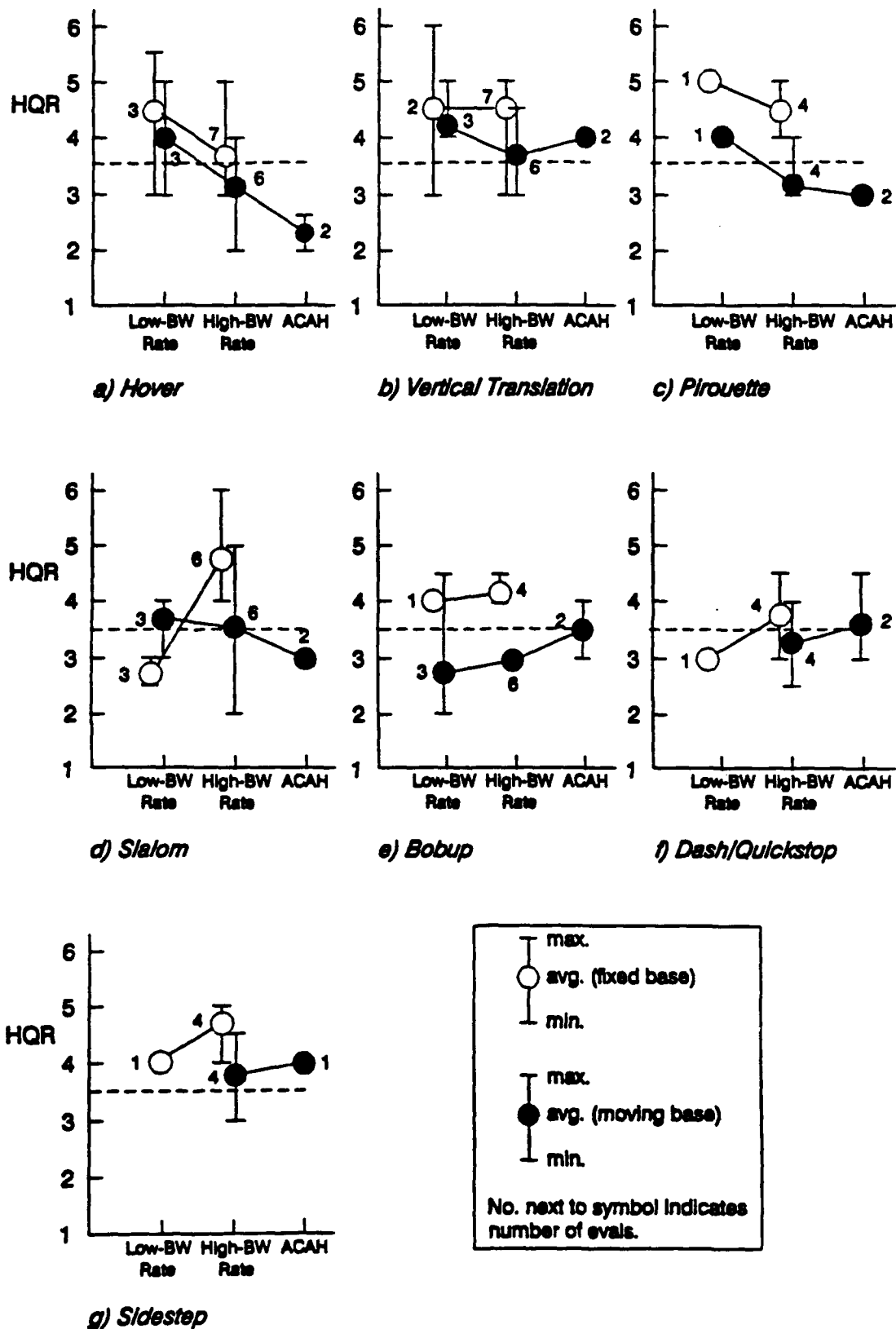
Figure 21. Effects of Bandwidth and Response-Type on HQRs (No Added Time Delay, Visual Compensation On, Baseline Motion)
