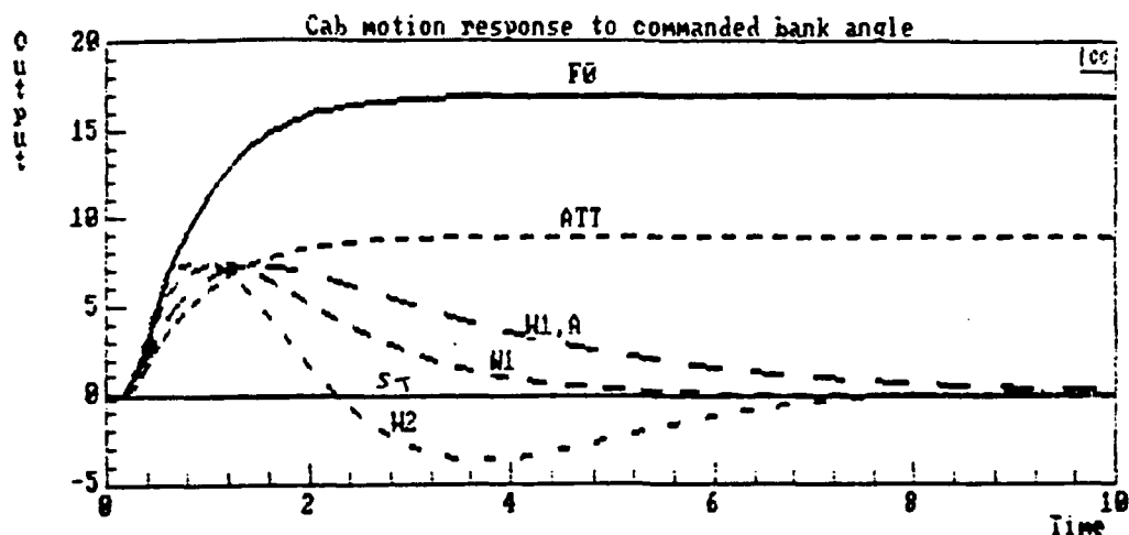
a) Bank Angle Responses to a Unit Control Input
