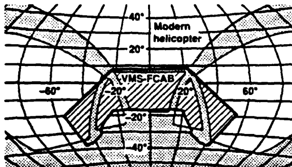
Figure 14. FCAB Display Field-of-View Plot (From Ref. 13)
