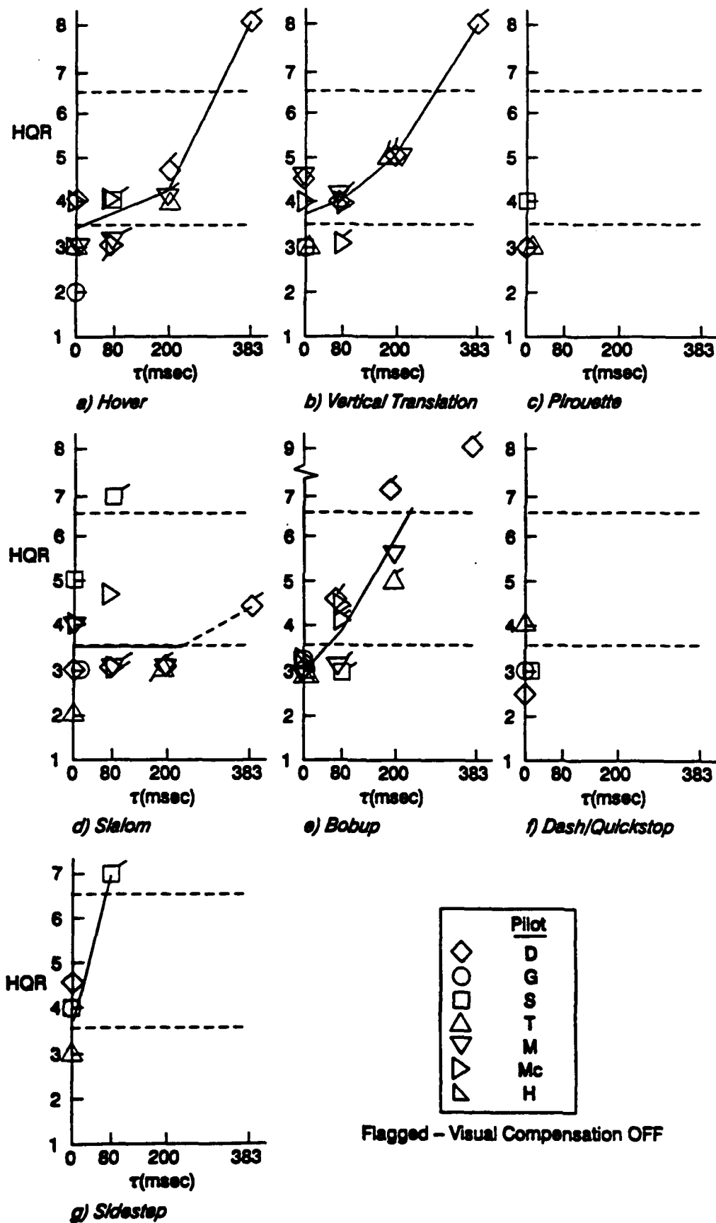
Figure 20. Time Delay Variations — Moving Base
