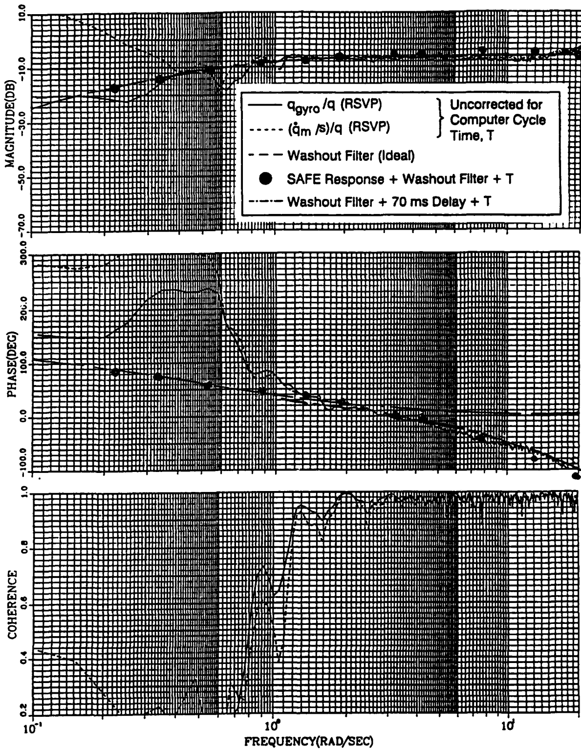
c) Pitch Rate (Motion System Acceleration Response, \dot{q}_m , Resolved to Rate by Dividing by s)
