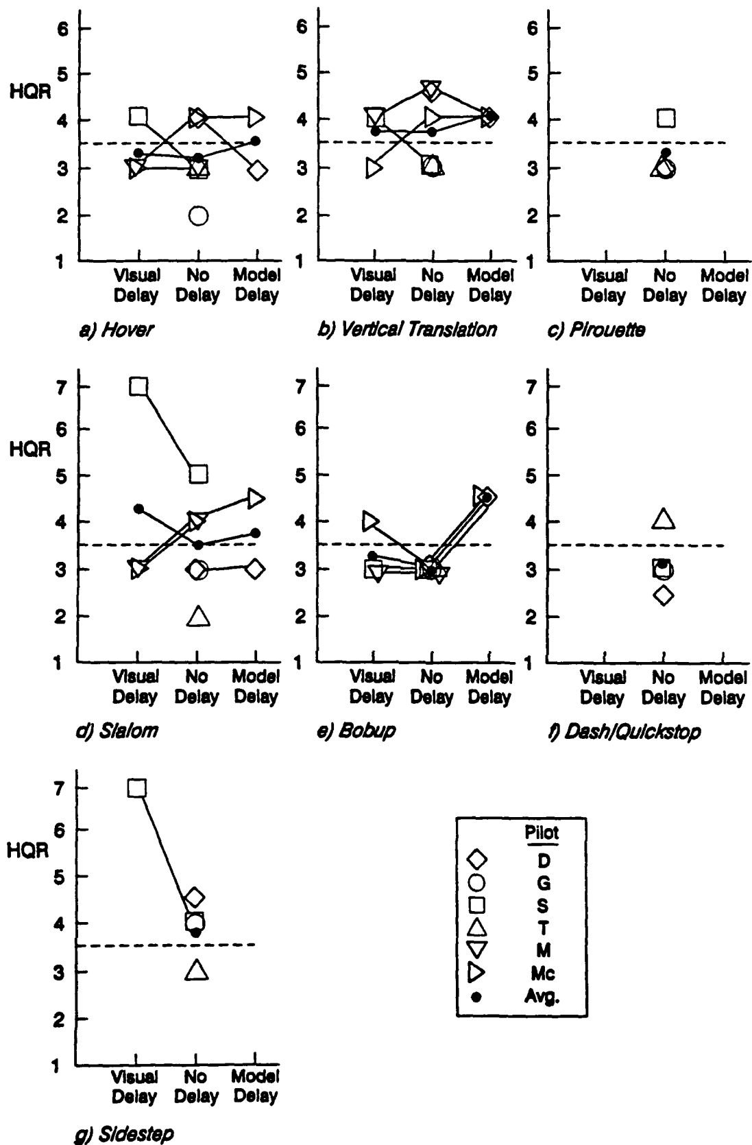
Figure 17. Effects on HQR of Introducing Approximately 80 msec of Time Delay in the Visual Scene Alone (Visual Delay), and in the Total Simulation Model (Model Delay). Baseline Motions, High-Bandwidth Rate Response-Type
