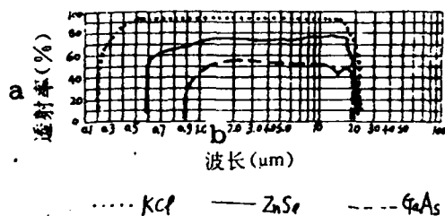
Fig. 2. Comparison of transmissibility of several materials KEY: a - transmissibility (%) b - wavelength (micrometers)
