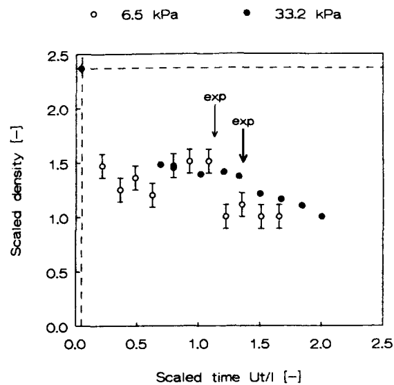
Figure 5 The scaled density as a function of the scaled time, determined on the wedge face at a height y=0.08 H . Open and full dots indicate the results at shock strengths of respectively 6.5 kPa and 33.2 kPa. The vertical and horizontal dashed lines are respectively the time of arrival of the shock and the density calculated for regular reflection. The arrows indicate the arrival of E_1 (920538)
