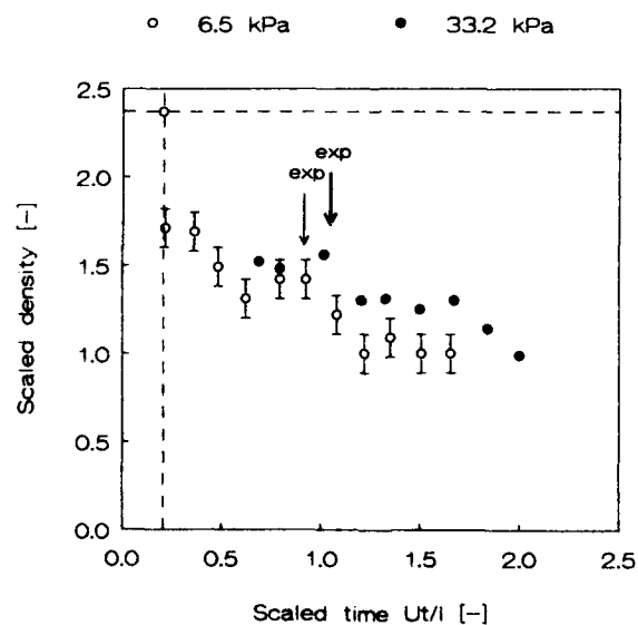
Figure 6 The scaled density as a function of the scaled time, determined on the wedge face at a height y=0.40 H . Open and full dots indicate the results at shock strengths of respectively 6.5 kPa and 33.2 kPa. The vertical and horizontal dashed lines are respectively the time of arrival of the shock and the density calculated for regular reflection. The arrows indicate the arrival of E_1 (920539)
