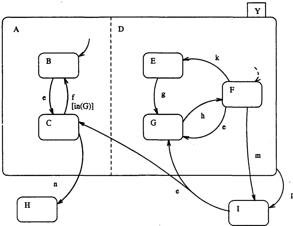
Figure 15: A Statechart
