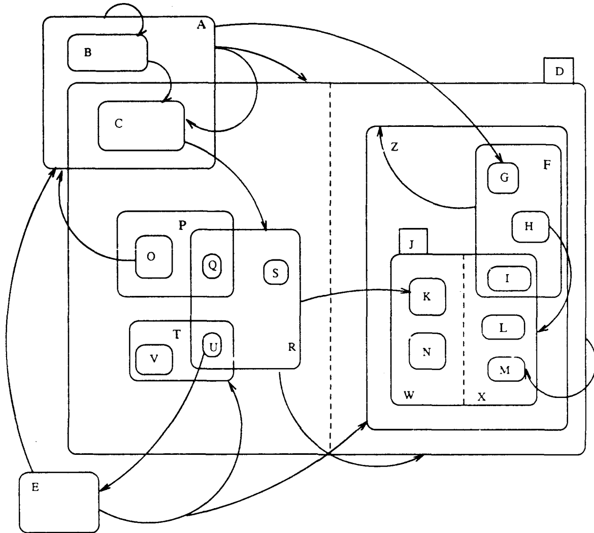
Figure 8: A higraph example
