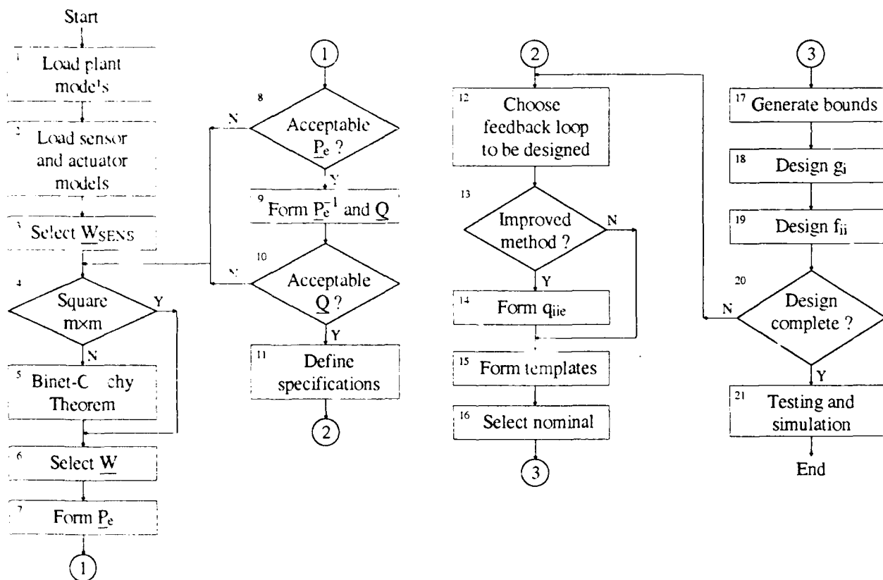
Fig. 3-29 Flowchart for MIMO QFT CAD Package
