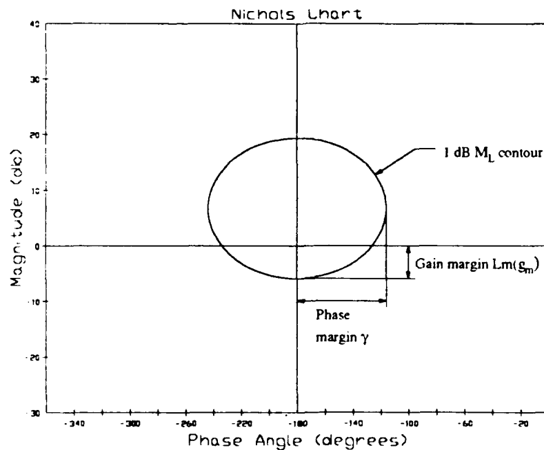
Fig. 2-10 Stability Specifications
