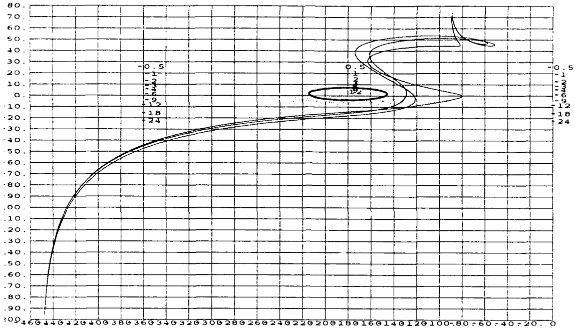
Fig. 4-52 Open loop transmissions for channel 2
