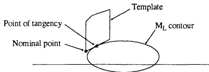
Fig. 3-11 Upper point of tangency with stability bound
