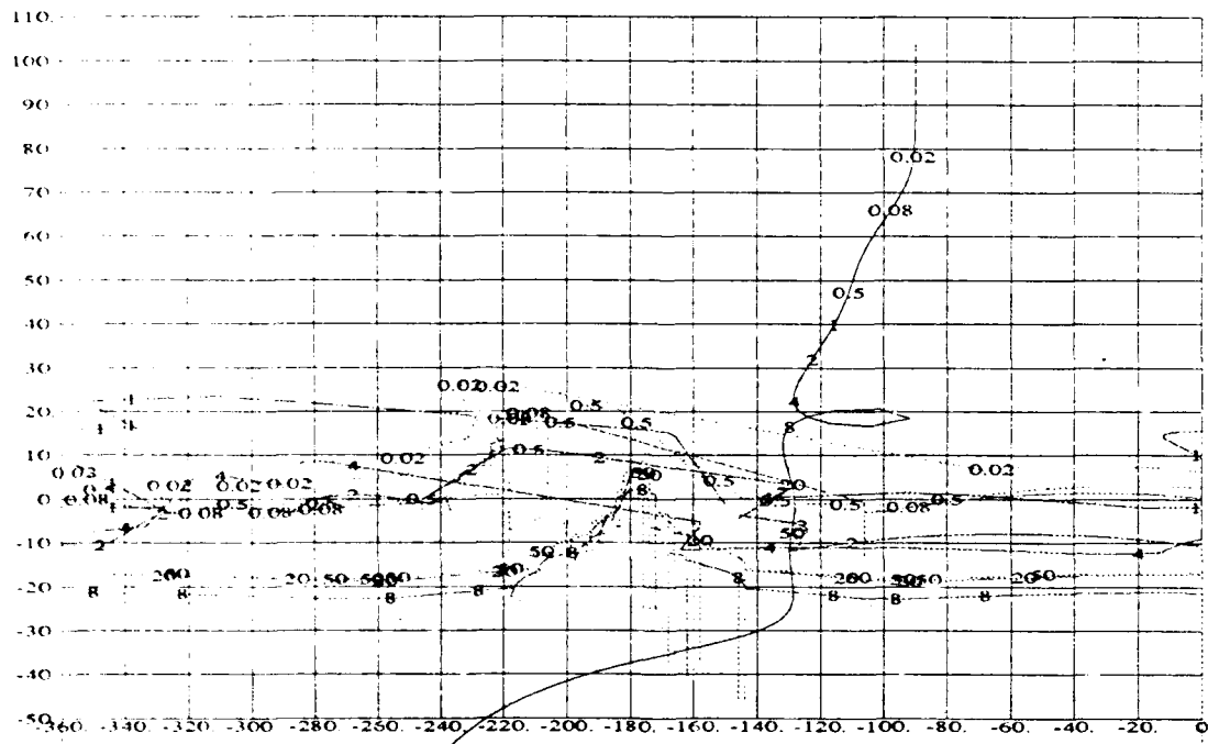
Fig. 4-18 Gamma bounds with OLTF for channel 2
