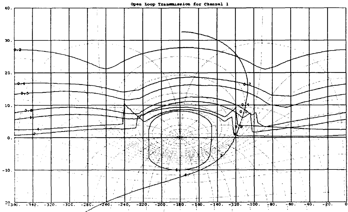
Fig. 4-42 Channel 1 OLTF with composite bounds
