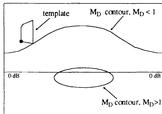
Fig. 3-18 Inverse Nichols chart
