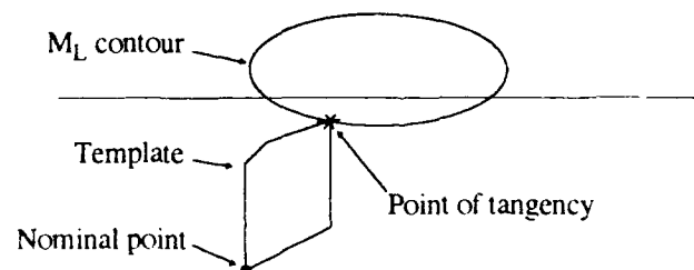
Fig. 3-16 Lower point of tangency with stability bound
