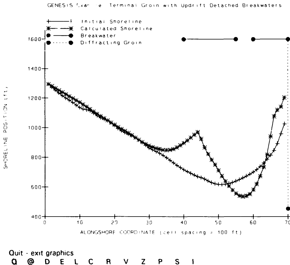
Figure 11. Example shoreline position plot
