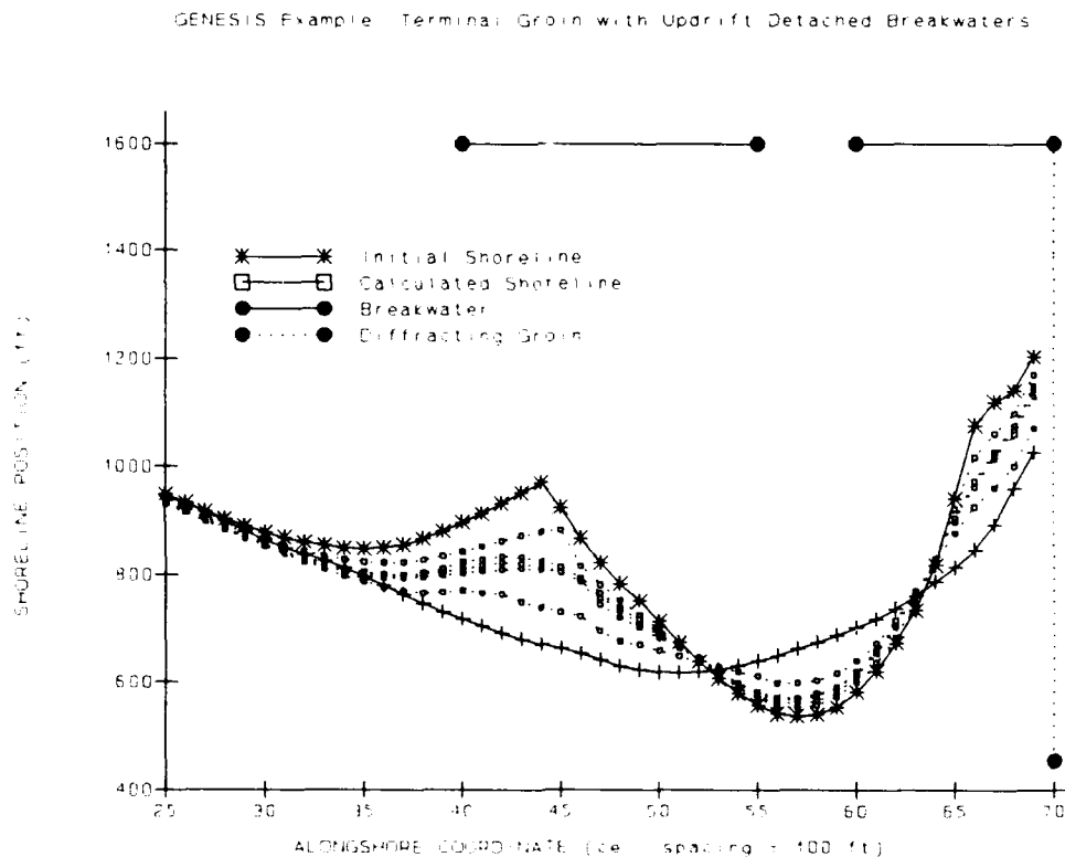
Figure 12. Shoreline plot with intermediate shoreline positions and zoom option
