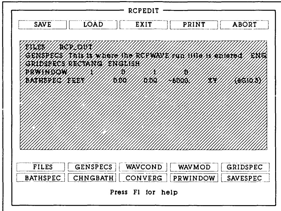
Figure 4. Schematic illustration of the RCPEDIT screen
