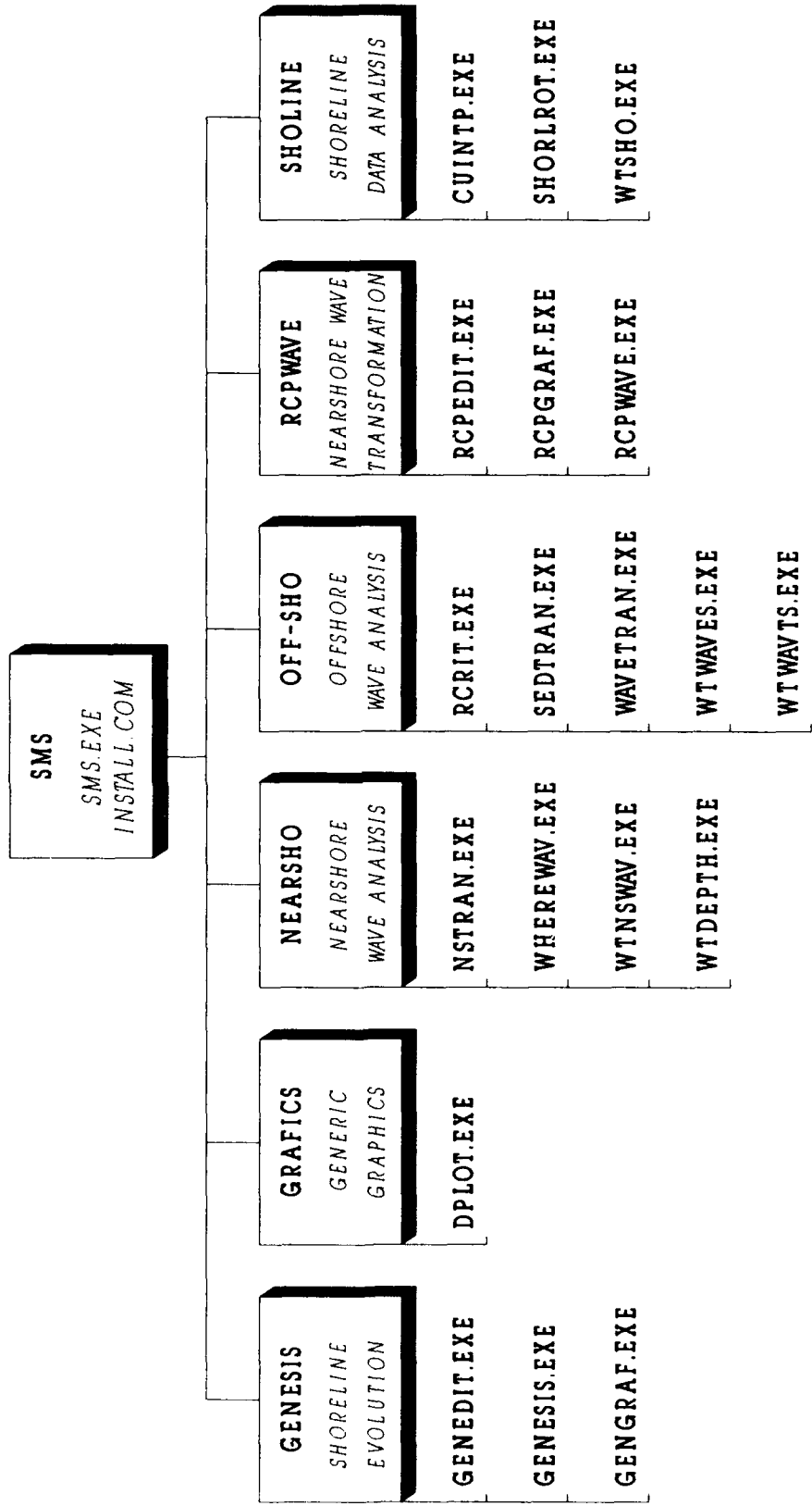
Figure 1. Directory structure and programs in the SMS
