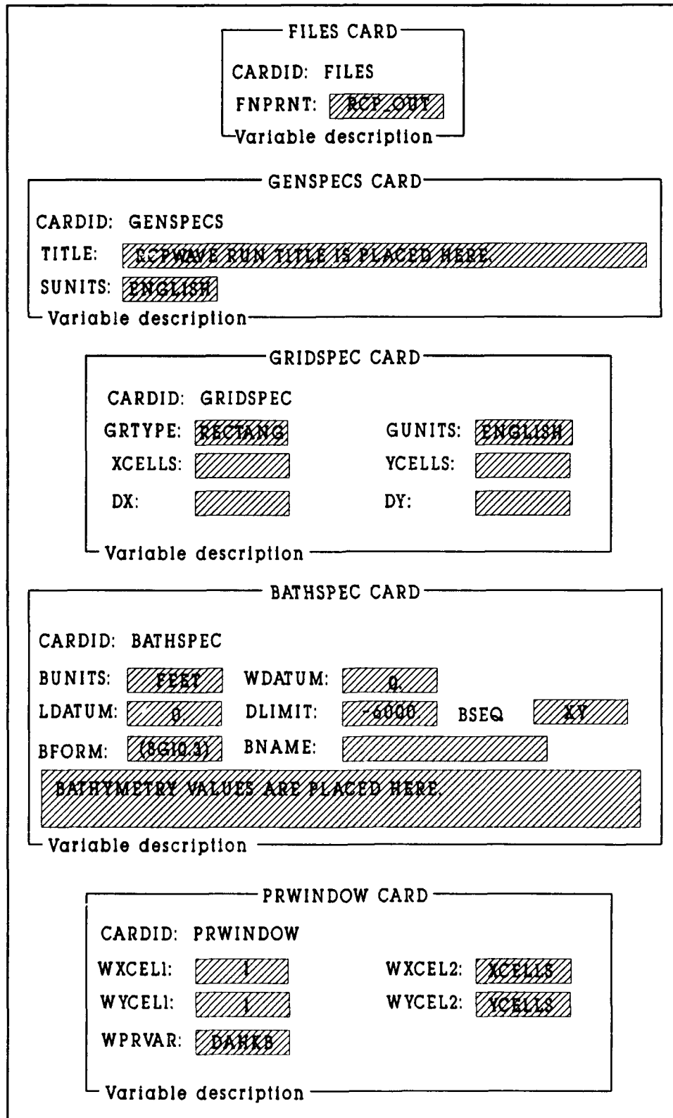
Figure 5. Required RCPWAVE input data cards
