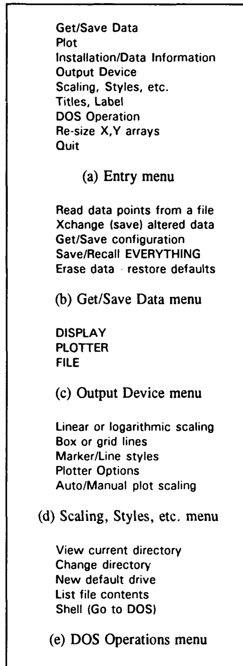
Figure 22. Selected DPLLOT menus
