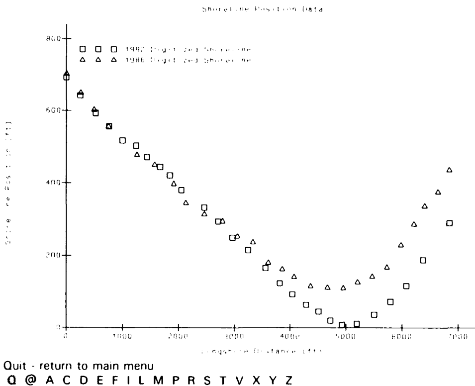
Figure 23. Digitized shoreline data
