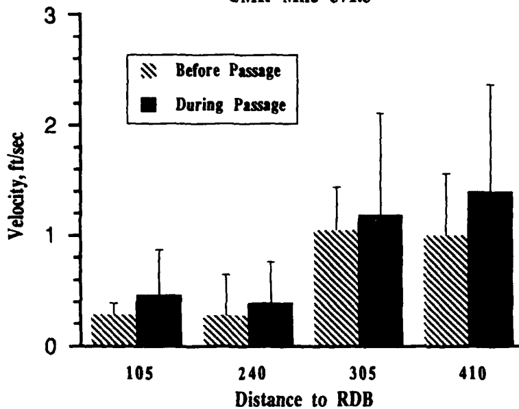
Figure 22. Mean and range in velocity (ft/sec) immediately before and during tests 14 and 20, UMR, July 1990. Velocity readings were taken parallel to flow. See tests 14 and 20 in Appendix E
