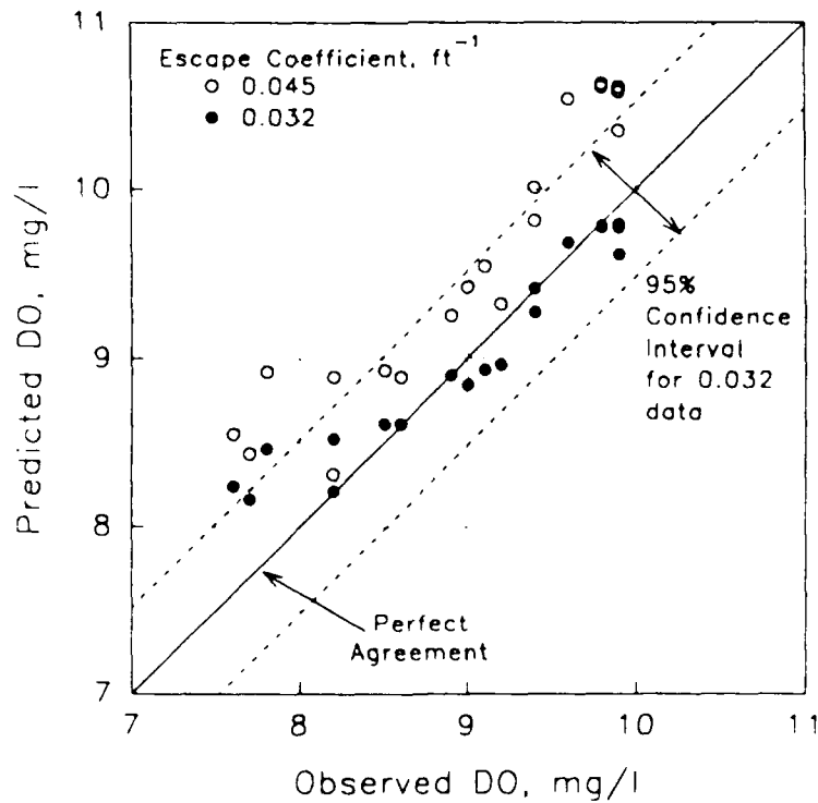
Figure 9. Selective withdrawal evaluation; dissolved oxygen
