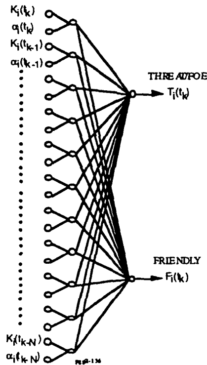
Figure 4.8: Maneuver Parameter Generator and Maneuver Classifier
