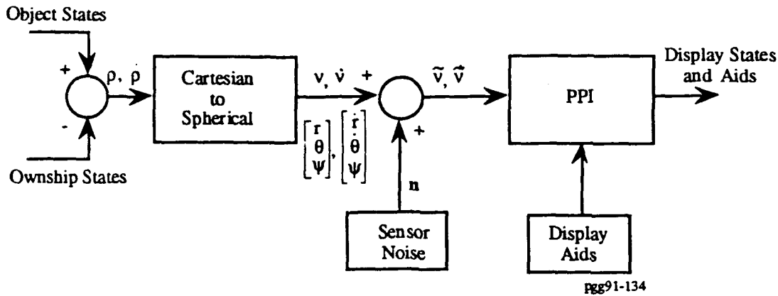
Figure 4.2: CSIM Implementation — Radar/TSD Modules
