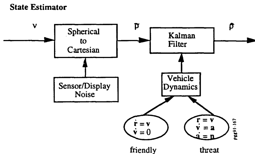
Figure 4.6: State Estimator Block Diagram
