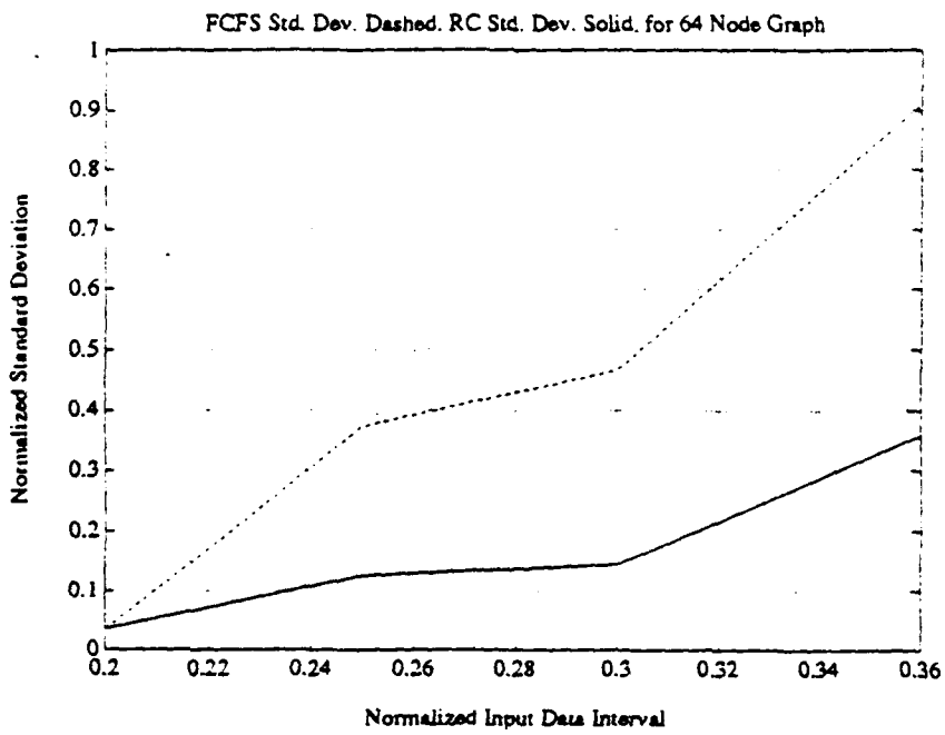
Figure 17: FFT Graph - Blow-up of Standard Deviation
