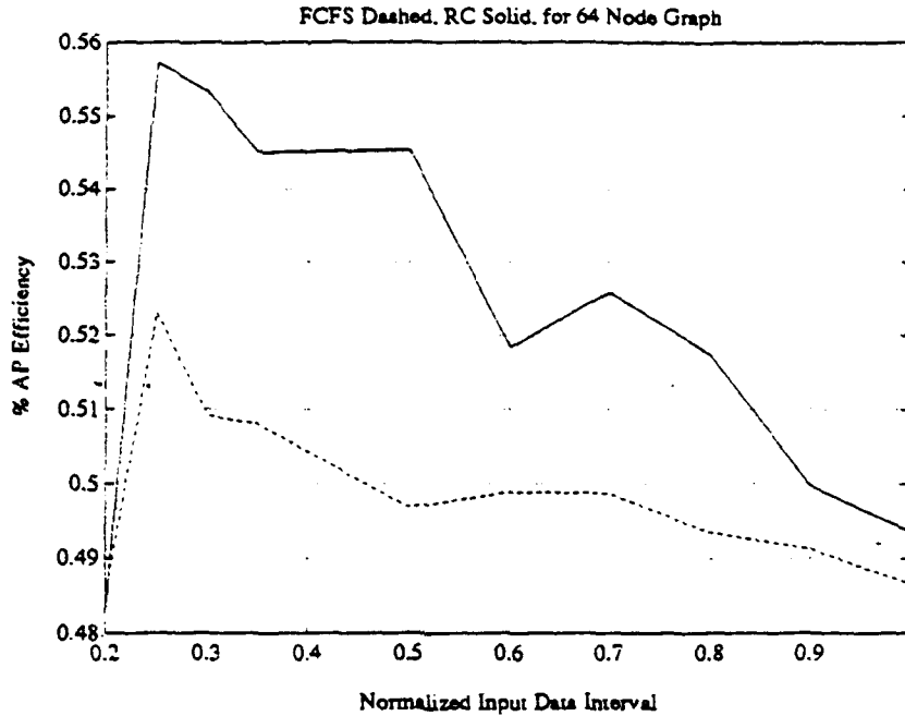
Figure 18: FFT Graph - Processor Efficiency
