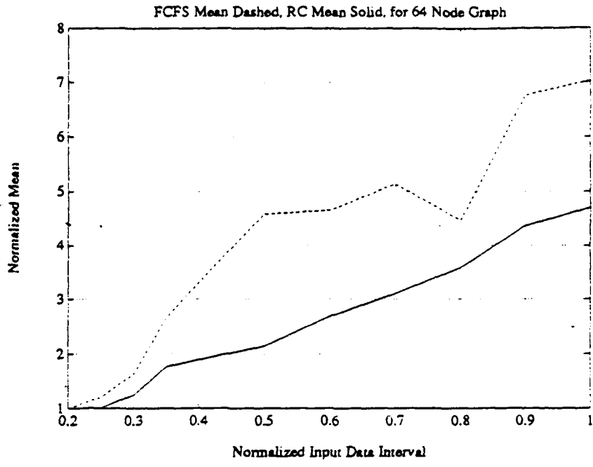
Figure 14: FFT Graph - Mean Instance Completion Times
