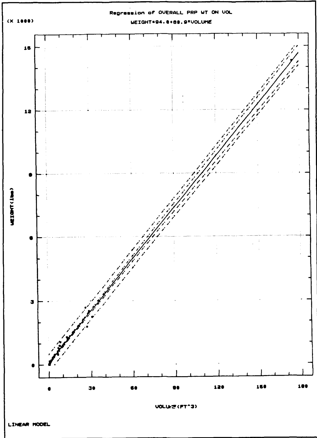
Figure B-19: Overall Propulsion Weight vs Propulsion Volume
