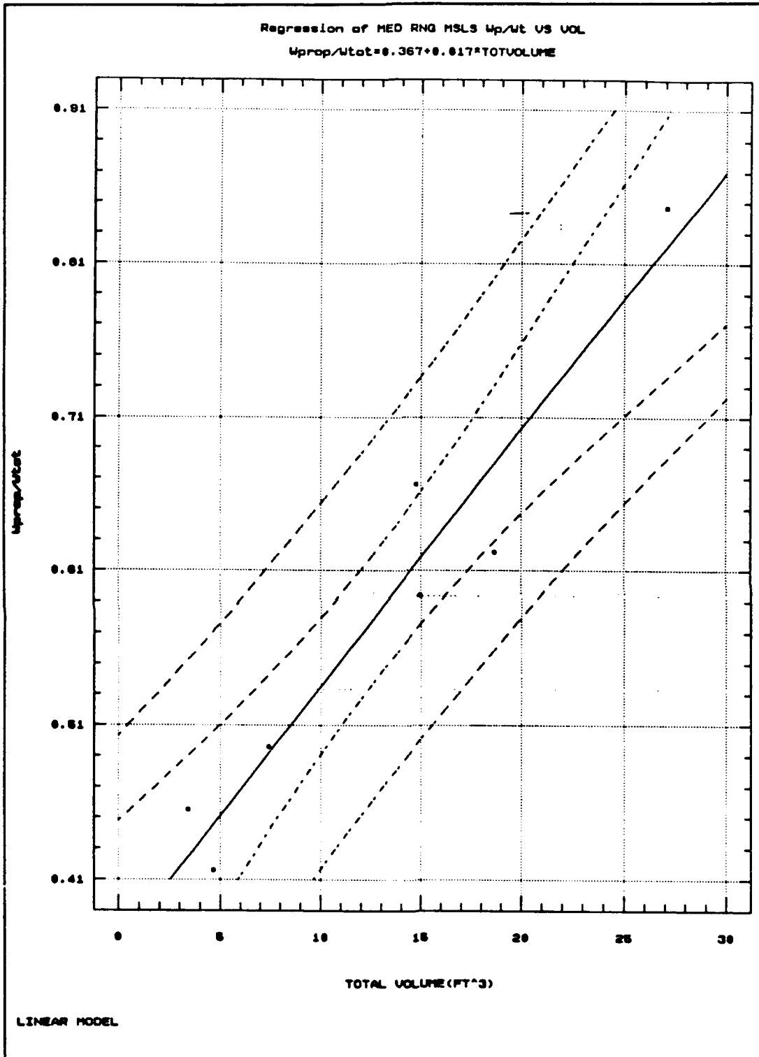
Figure B-40: Medium Range Missile W prop /W t vs Volume
