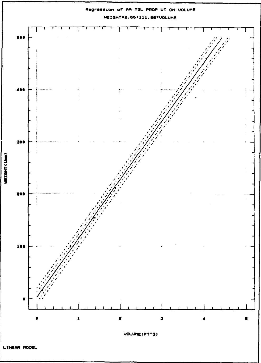
Figure B-22: AAM Propulsion Weight vs Volume
