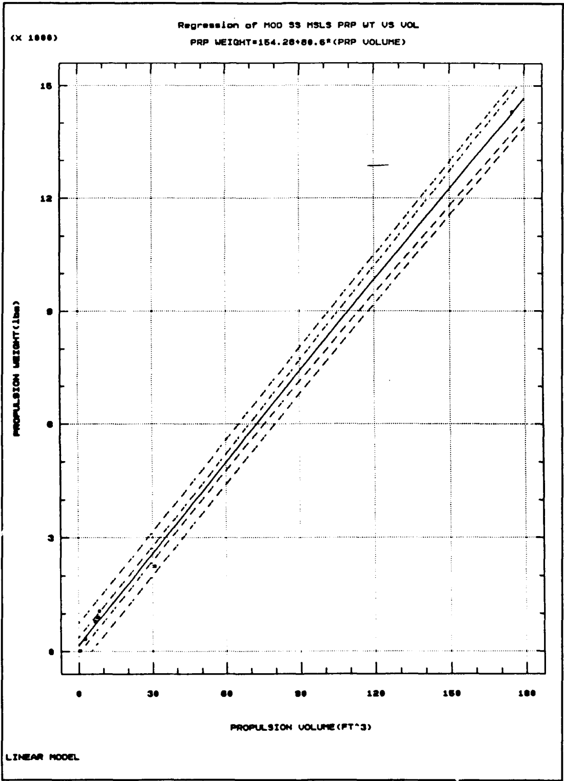
Figure B-48: SSM Rocket Prop Only Prop Wt vs Prop Vol
