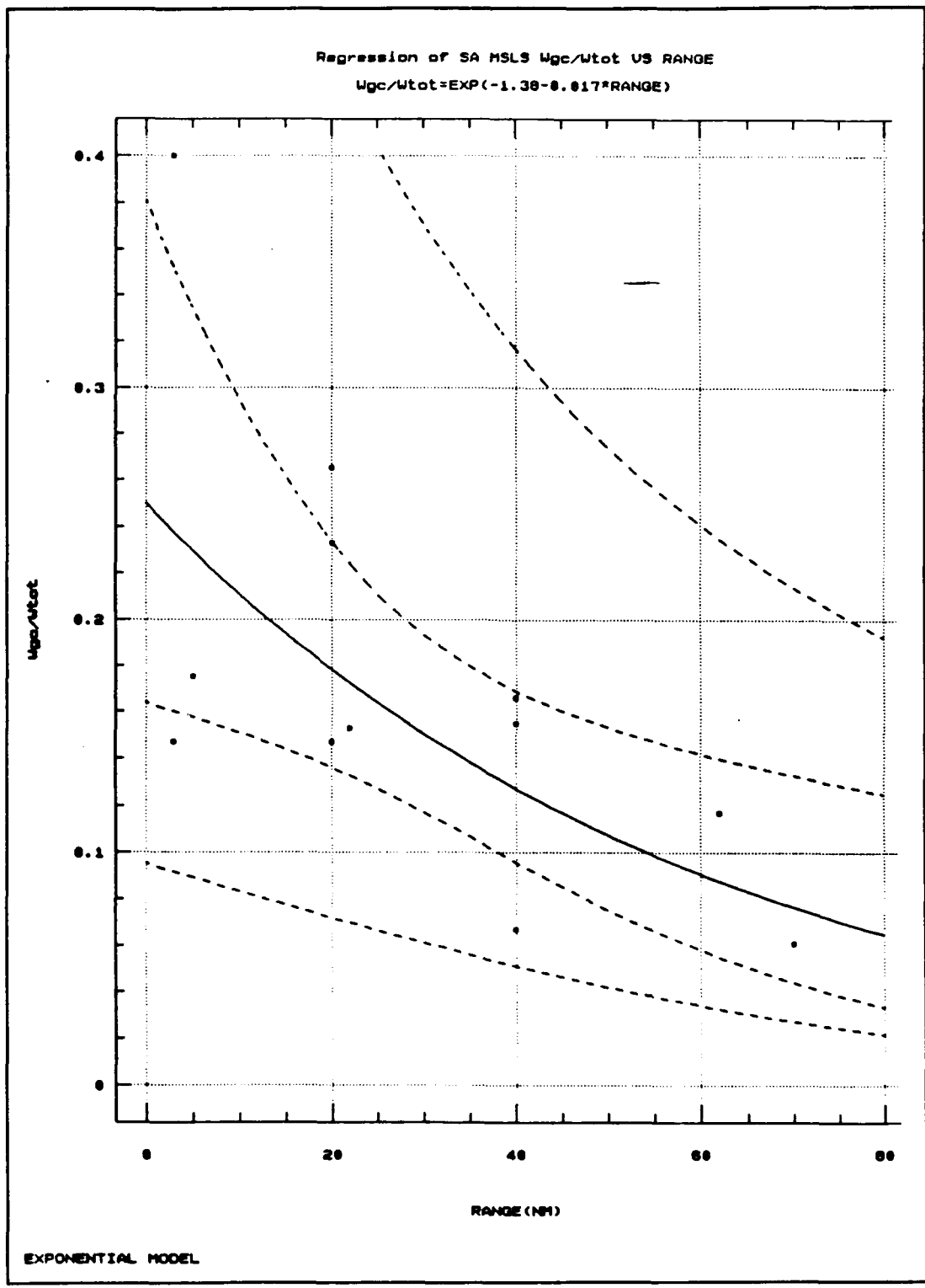
Figure B-62: SAM Wgc/Wt vs Range
