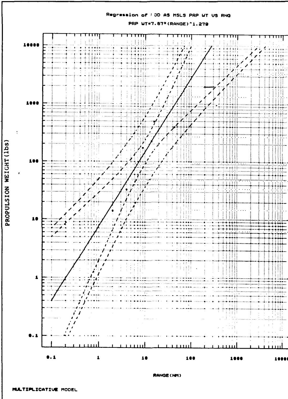
Figure B-46: ASM Rocket Prop Only Prop Wt vs Range
