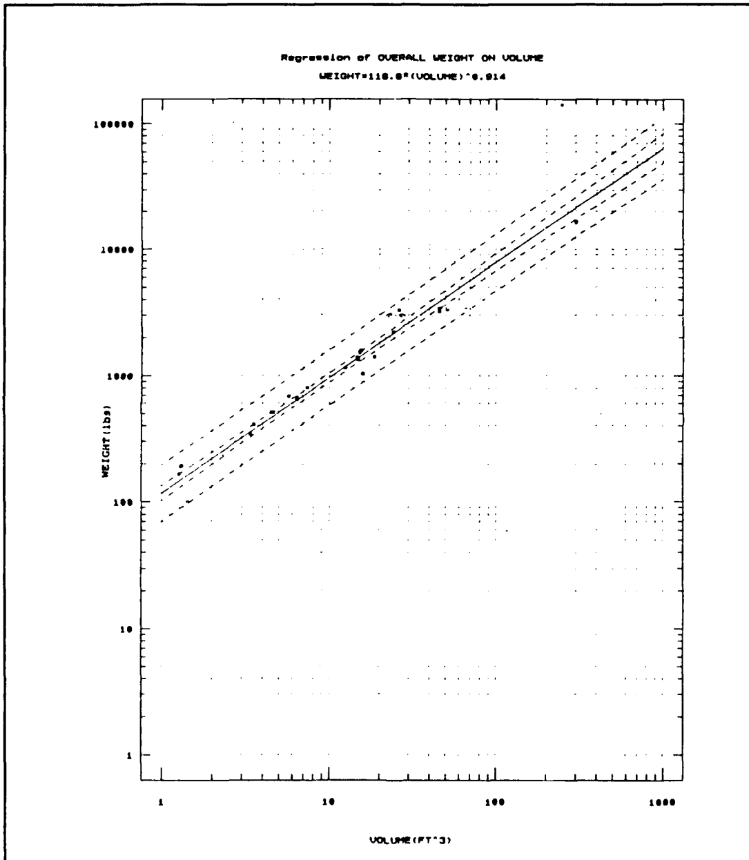
Figure 6: Sample Plot
