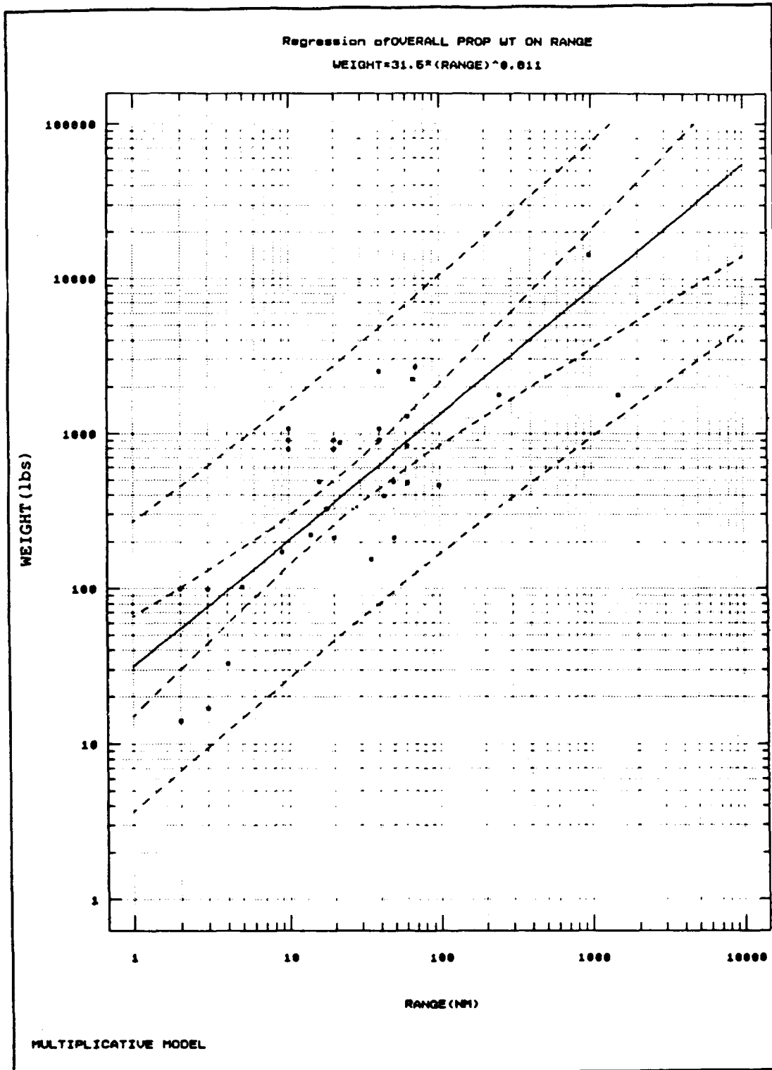
Figure B-20: Overall Propulsion Weight vs Range
