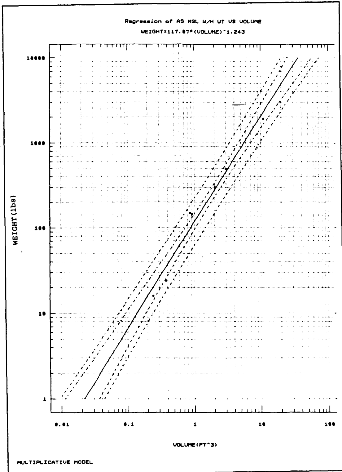
Figure B-71: ASM W/H Weight vs W/H Volume
