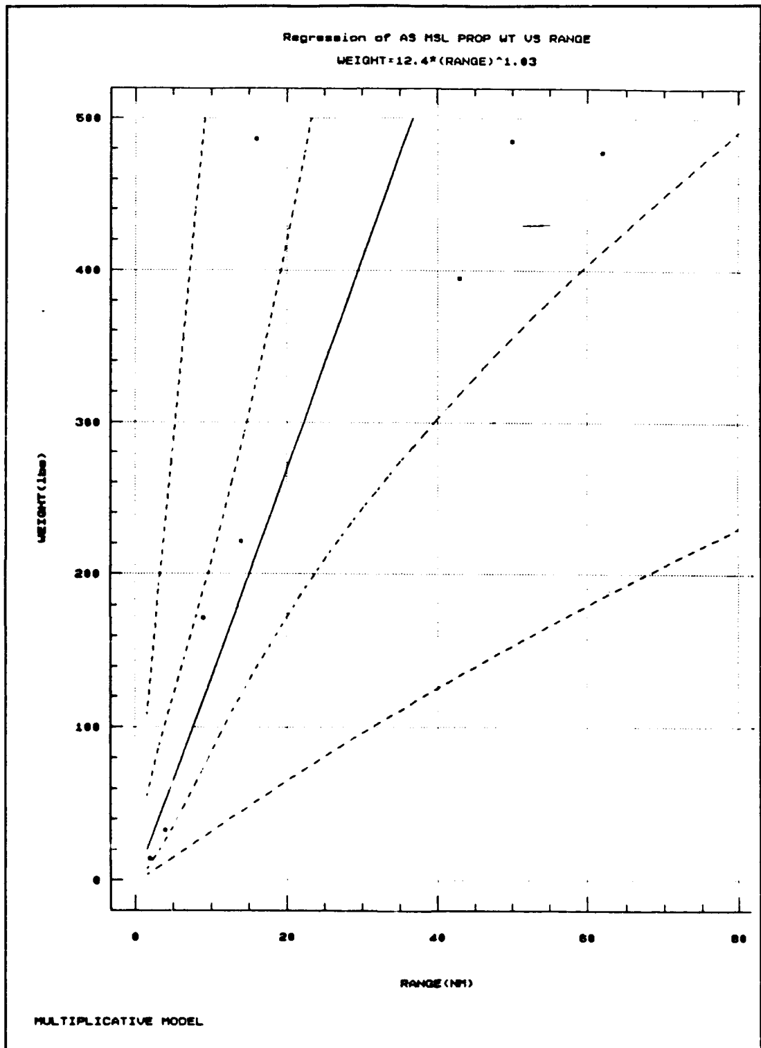
Figure B-28: ASM Propulsion Weight vs Range
