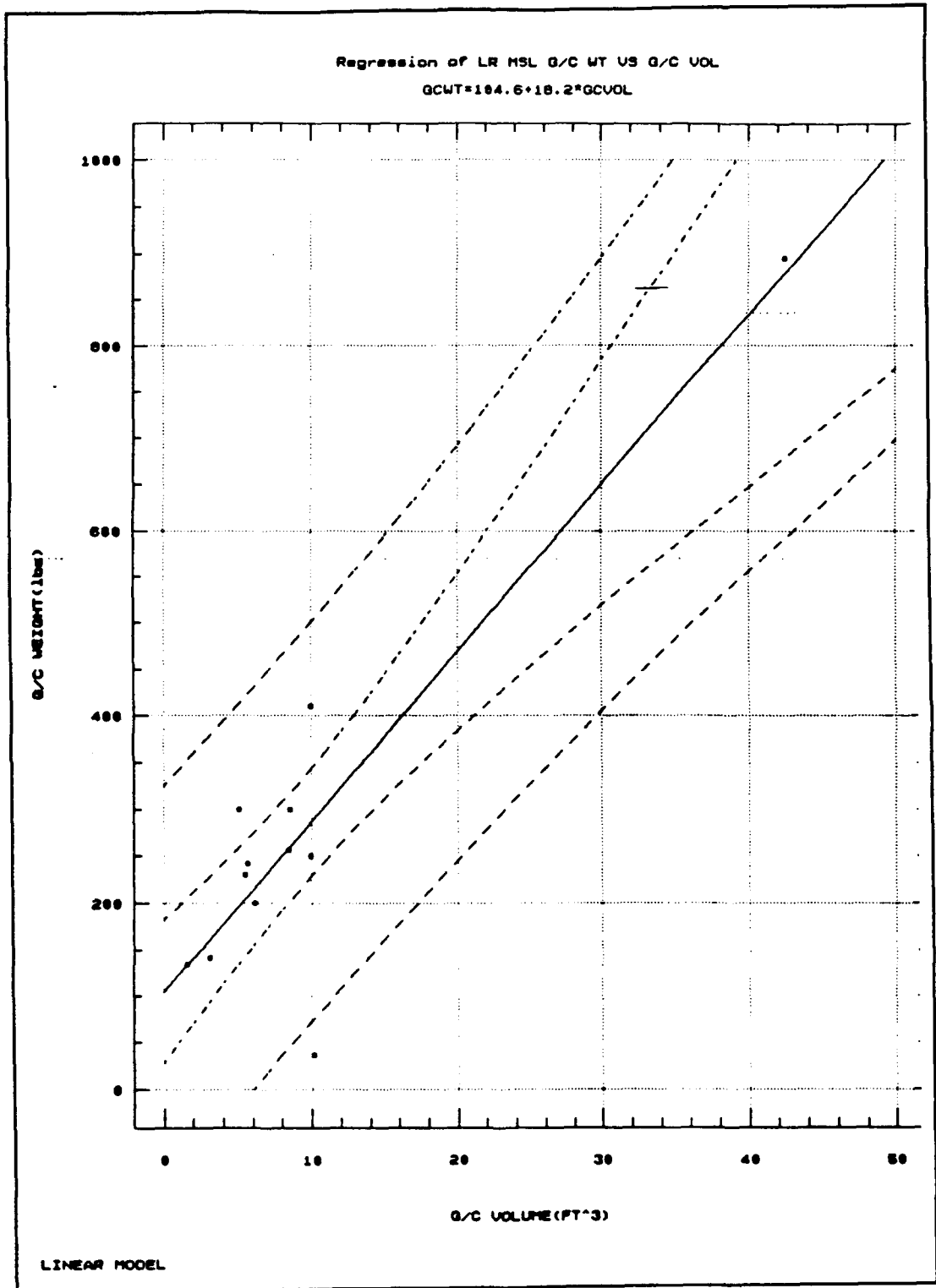
Figure B-67: Long Range Missile G/C Weight vs G/C Volume
