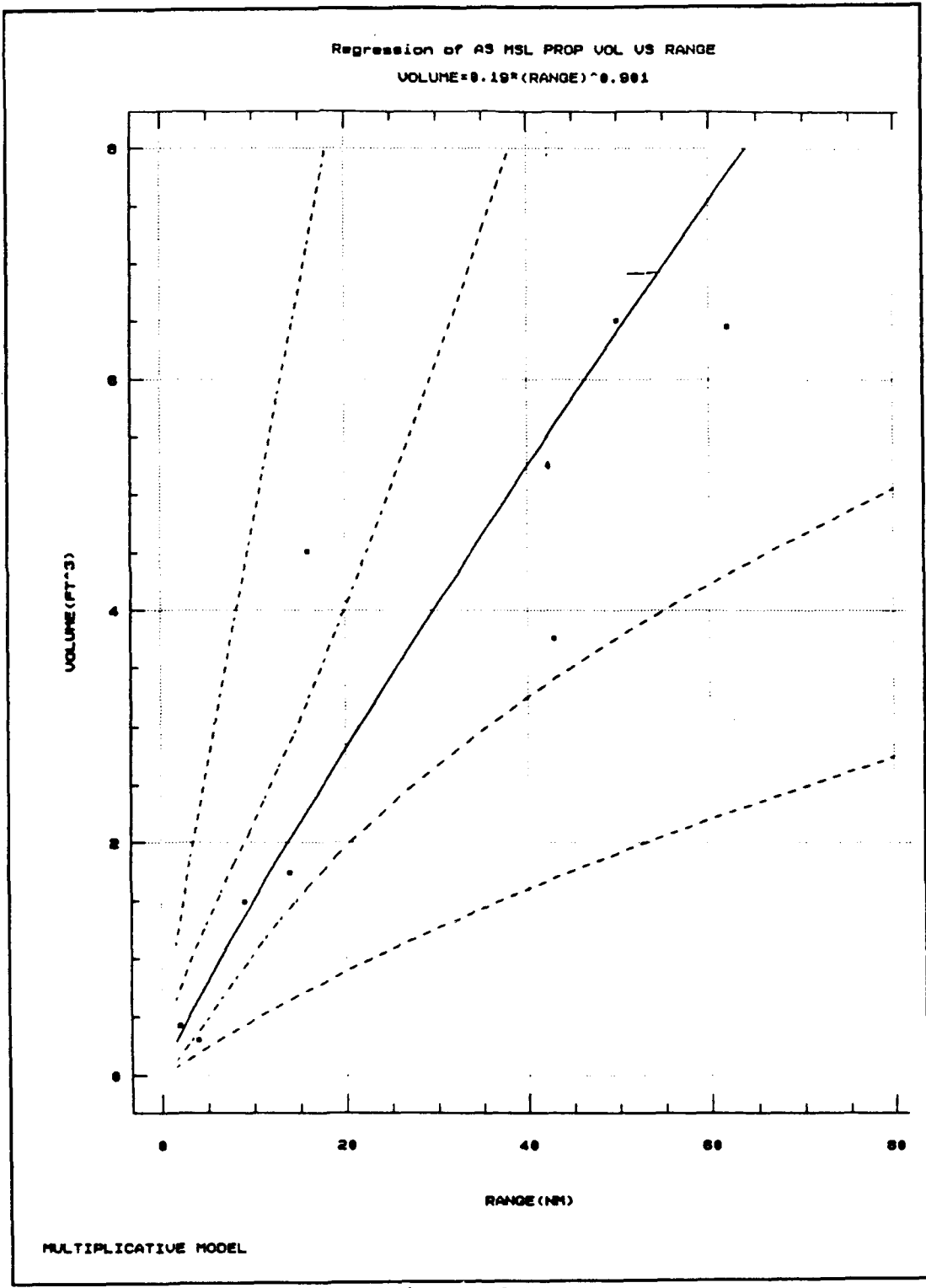
Figure B-29: ASM Propulsion Volume vs Range
