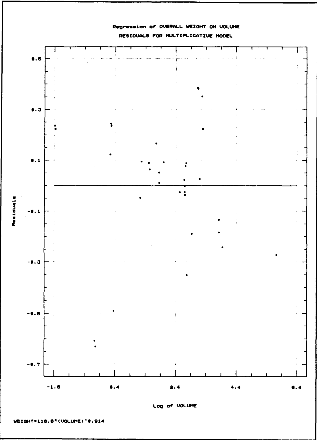
Figure 5: Residuals Plot
