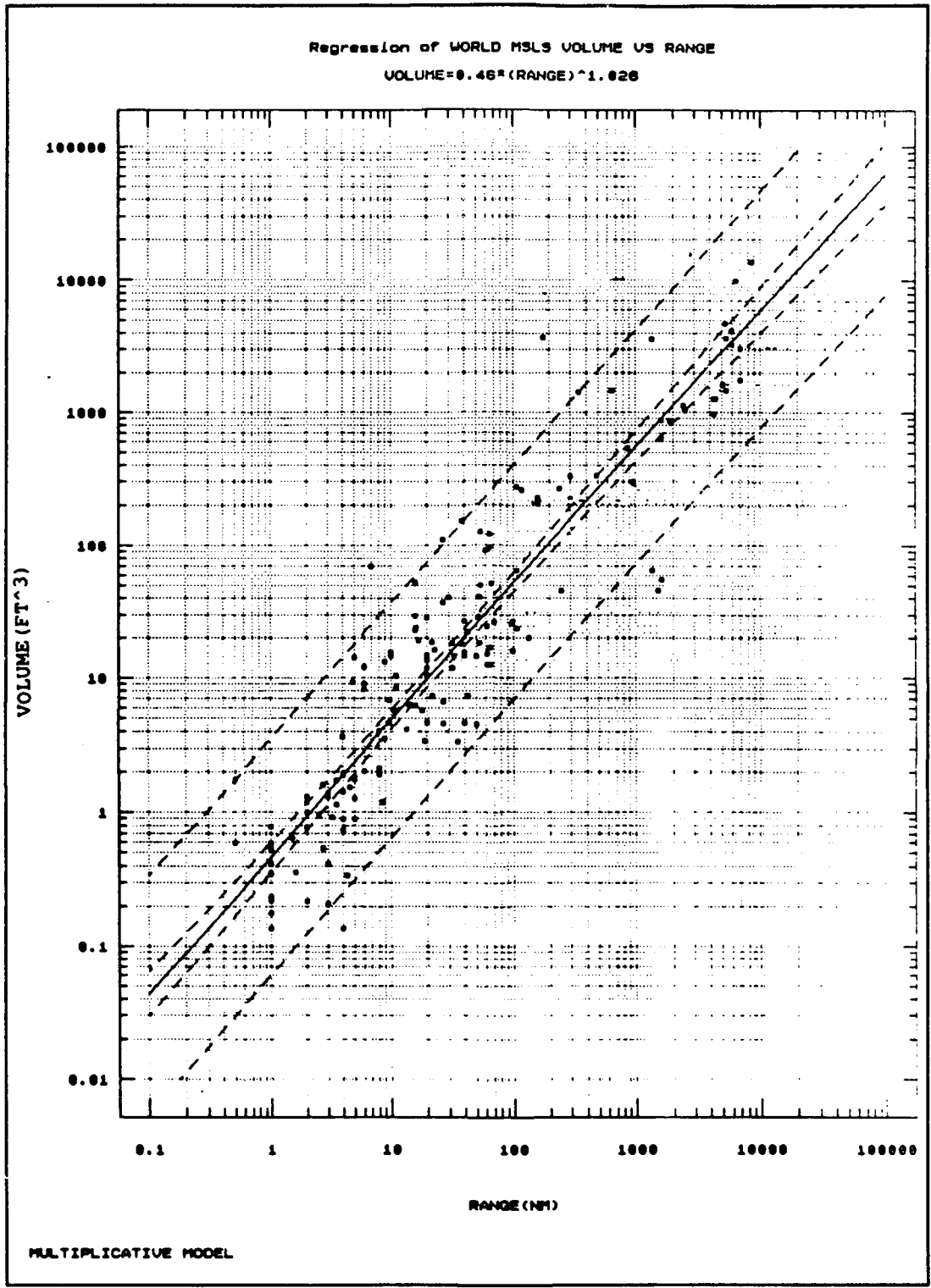
Figure B-3: Overall Volume vs Range
