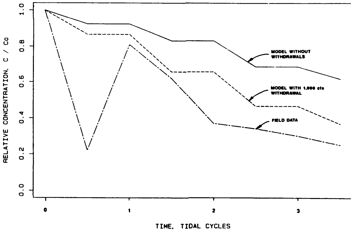
Figure 5. Model dye washout with and without withdrawals, and averaged field data for sites 9-15 starting at the 10:00-16:00-EST ebb tide of 30 August 1989
