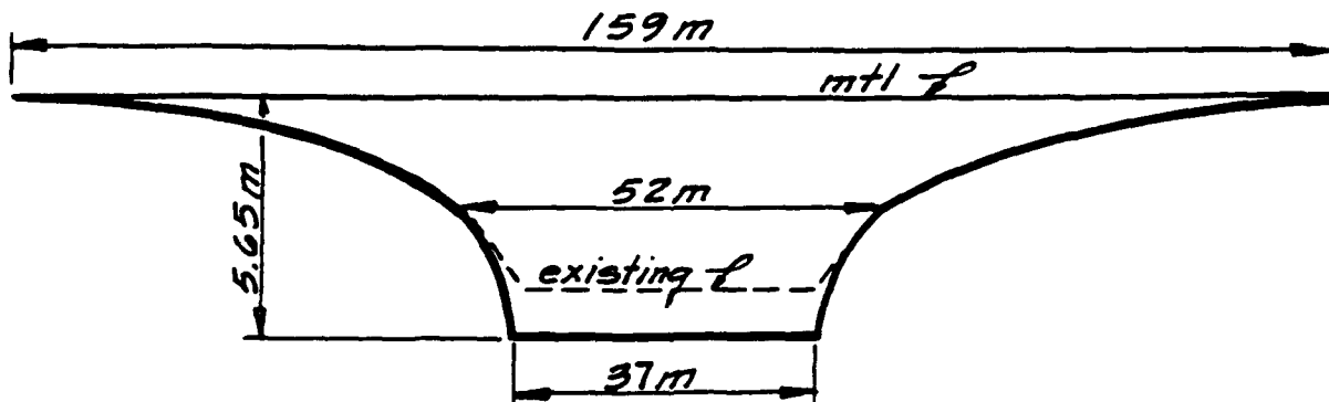
b. Deepened existing canal
