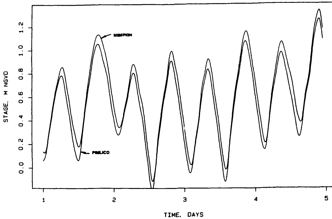
Figure 7. Comparison between Mempkin and Pimlico stages, May 1989
