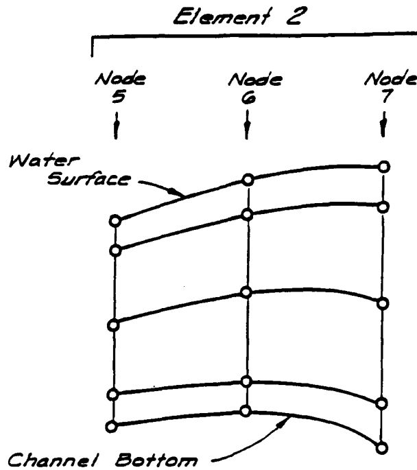
Figure A2. Example computational element from schematic mesh showing stretching coordinates and nodes
