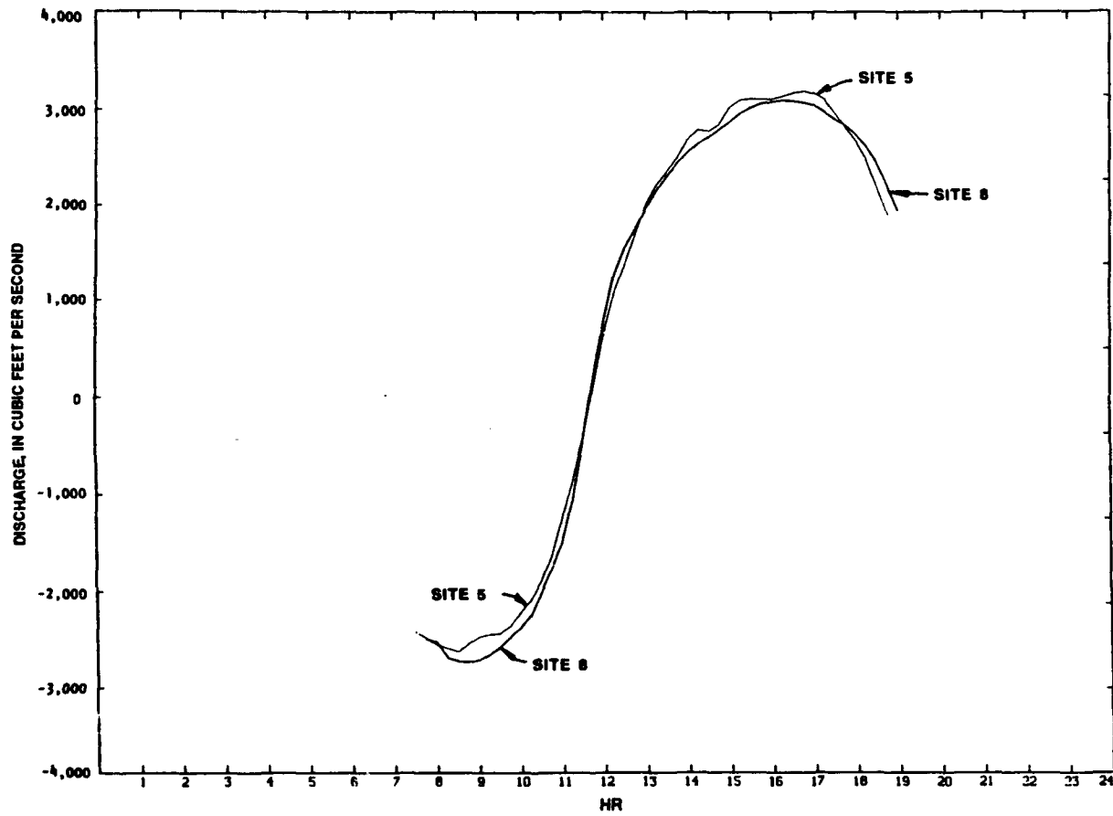
Figure 9. Flows at sites 5 and 8 for 9 August 1989
