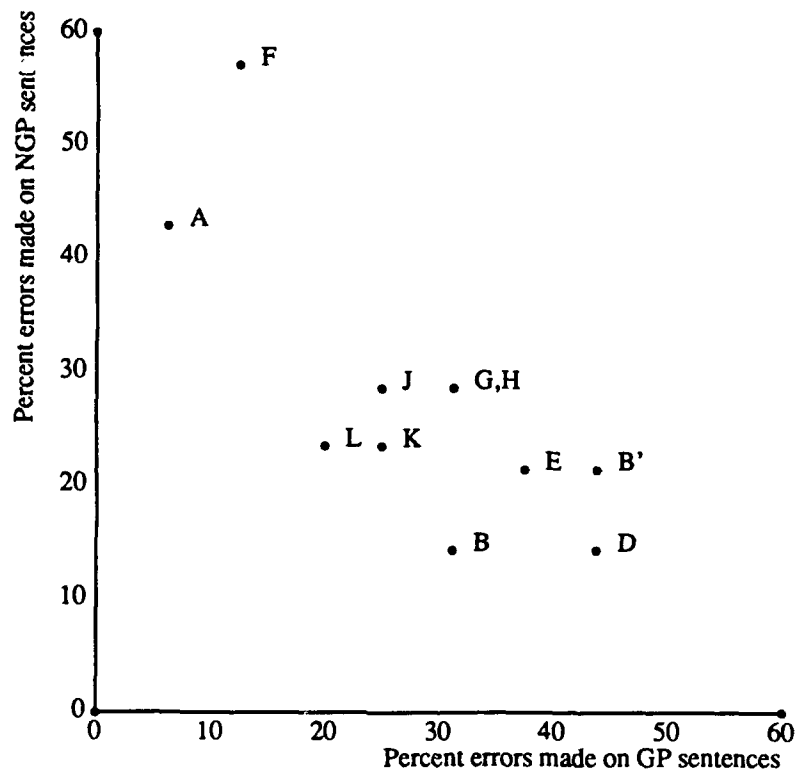
Figure 1: The tradeoff between predicting GP and NGP sentences.
