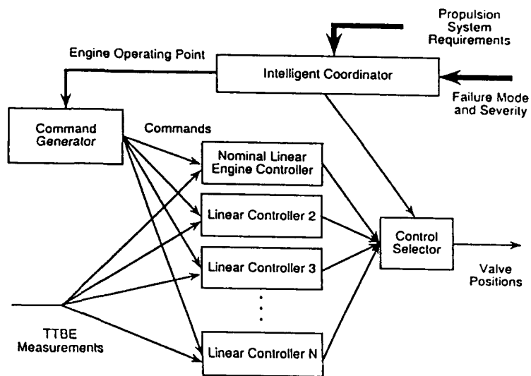
Figure 5 Multivariable Reconfigurable Control Scheme
