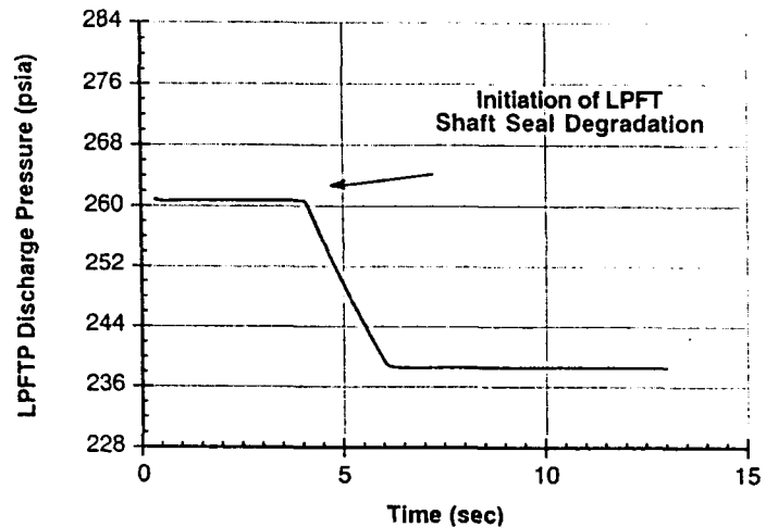
Figure 2a Open Loop Response of LPFTP Discharge Pressure to LPFTP Shaft Seal Degradation
