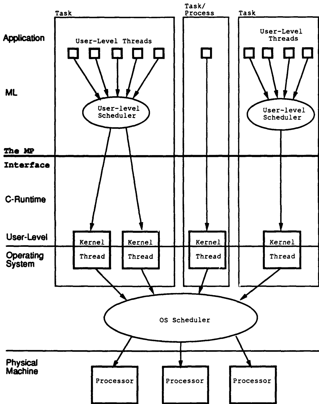
Figure 1: Relationship of Tasks, Kernel Threads, and User-Level Threads
