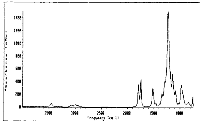
HFAA Derivative
