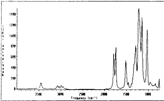
PFPA Derivative
