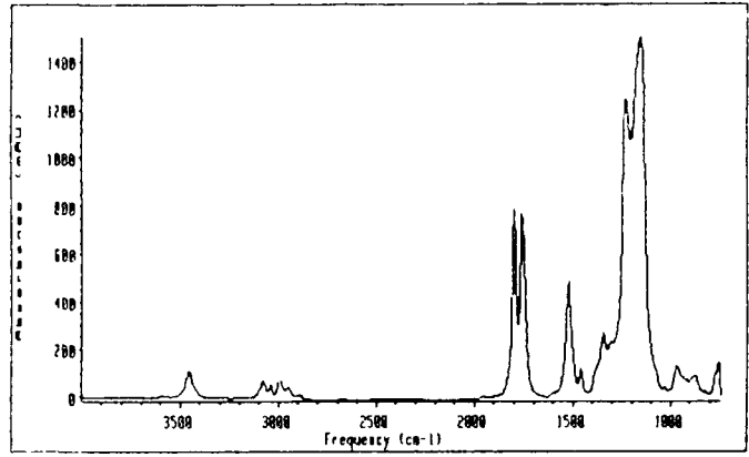
TFAA Derivative
