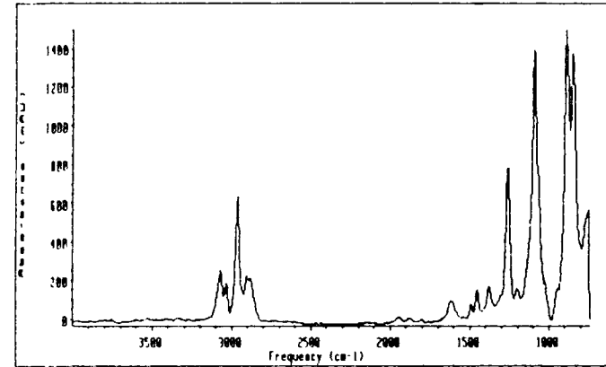
BSFTA Derivative
