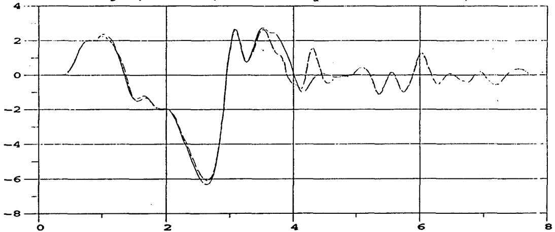
M35A2 Roll Angle; 40 MPH; M105A2 Payload = 3000 lbs, even dist.
