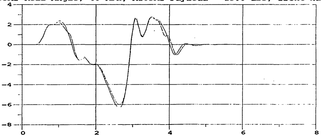
M35A2 Roll Angle; 40 MPH; M105A2 Payload = 1500 lbs, front half
