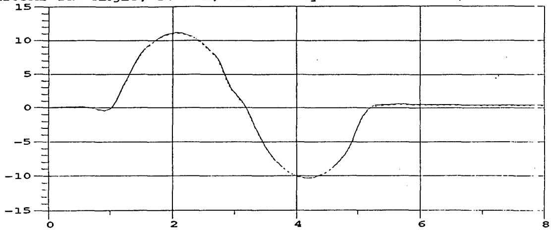
M105A2 Yaw Angle; 30 MPH; M105a2 Payload = 1500 lbs, left center
