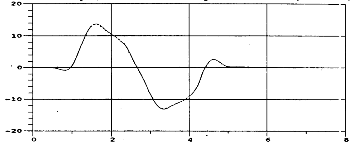
M105A2 Yaw Angle; 35 MPH; M105A2 Payload = 3000 lbs, rear half
