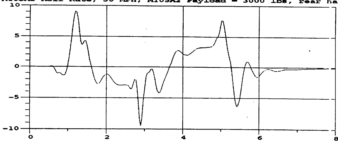
M105A2 Roll Rate; 30 MPH; M105A2 Payload = 3000 lbs, rear half
