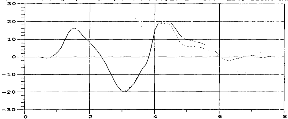
M105A2 Yaw Angle; 40 MPH; M105A2 Payload = 3000 lbs, front half
