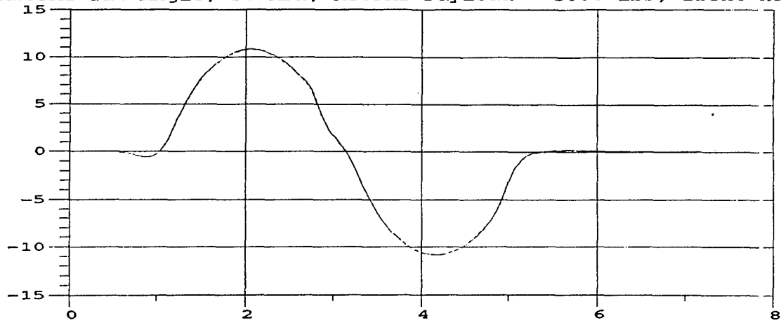
M105A2 Yaw Angle; 30 MPH; M105A2 Payload = 3000 lbs, front half
