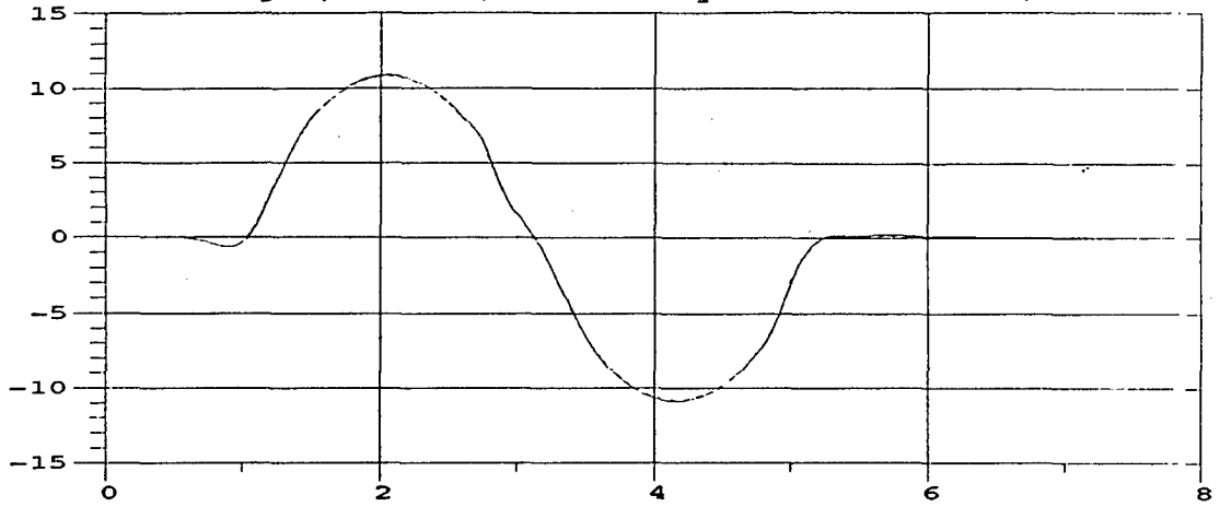
M105A2 Yaw Angle; 30 MPH; M105A2 Payload = 3000 lbs, even dist.
