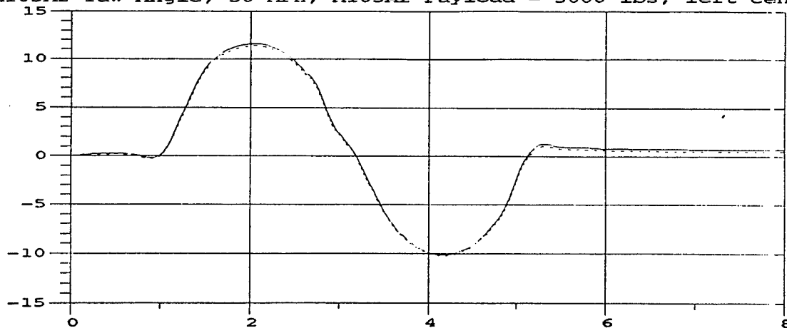
M105A2 Yaw Angle; 30 MPH; M105A2 Payload = 3000 lbs, left center
