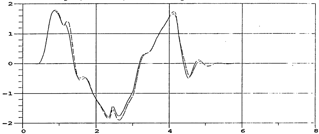
M35A2 Roll Angle; 35 MPH; M105A2 Payload = 3000 lbs, front half
