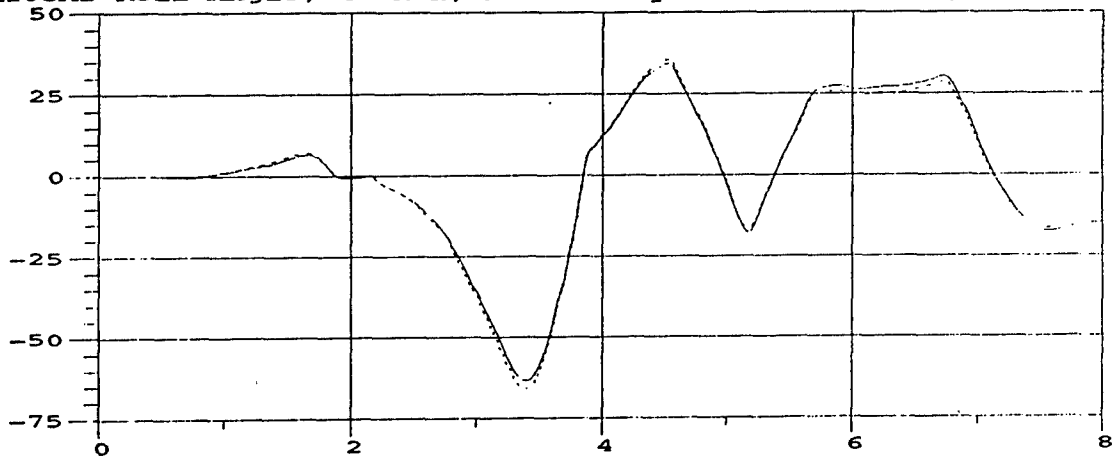
M105A2 Roll Angle; 40 MPH; M105A2 Payload = 3000 lbs, even dist.
