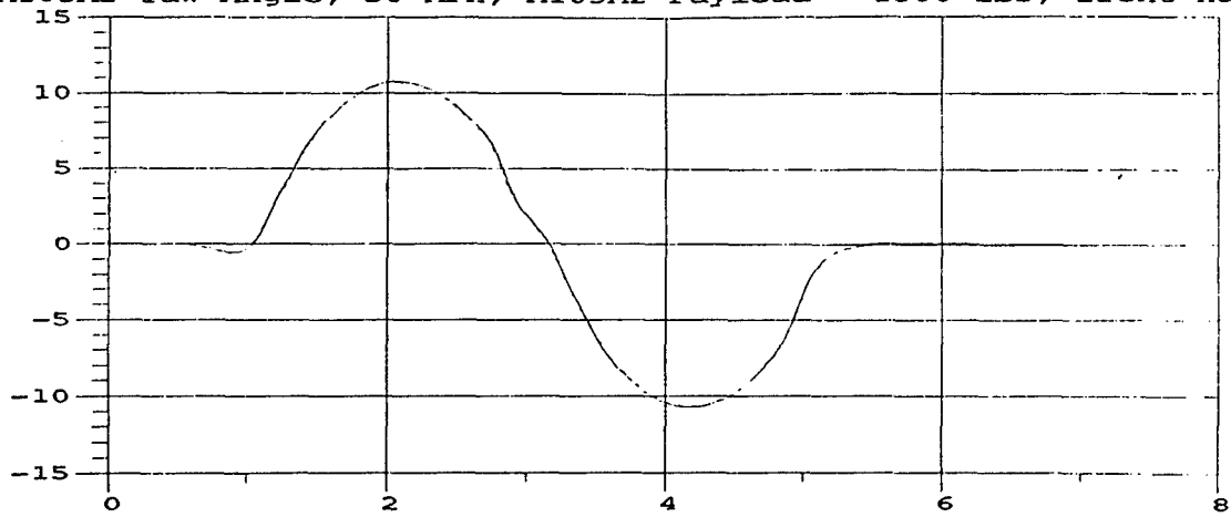
M105A2 Yaw Angle; 30 MPH; M105A2 Payload = 1500 lbs, front half
