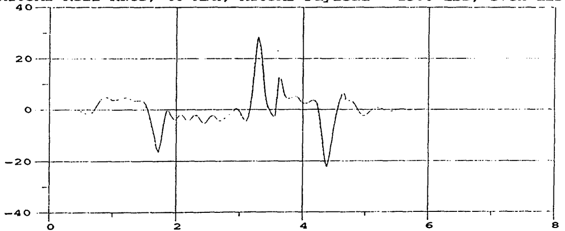
M105A2 Roll Rate; 40 MPH; M105A2 Payload = 1500 lbs, even dist.
