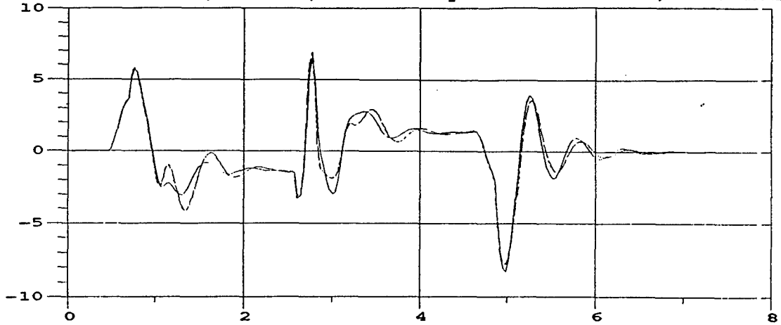
M35A2 Roll Rate; 30 MPH; M105A2 Payload = 1500 lbs, rear half
