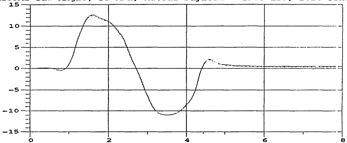
M105A2 Yaw Angle; 35 MPH; M105a2 Payload = 1500 lbs, left center
