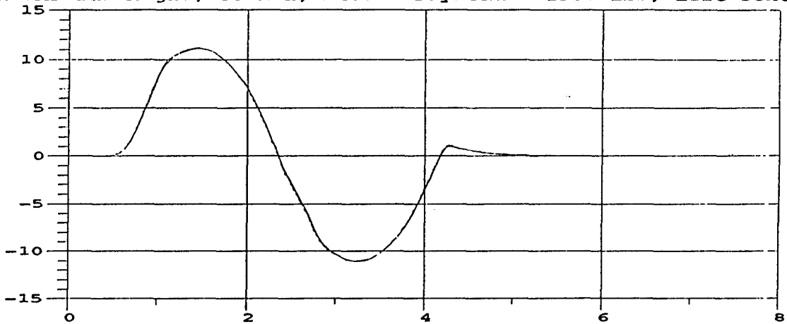
M35A2 Yaw Angle; 35 MPH; M105a2 Payload = 1500 lbs, left center
