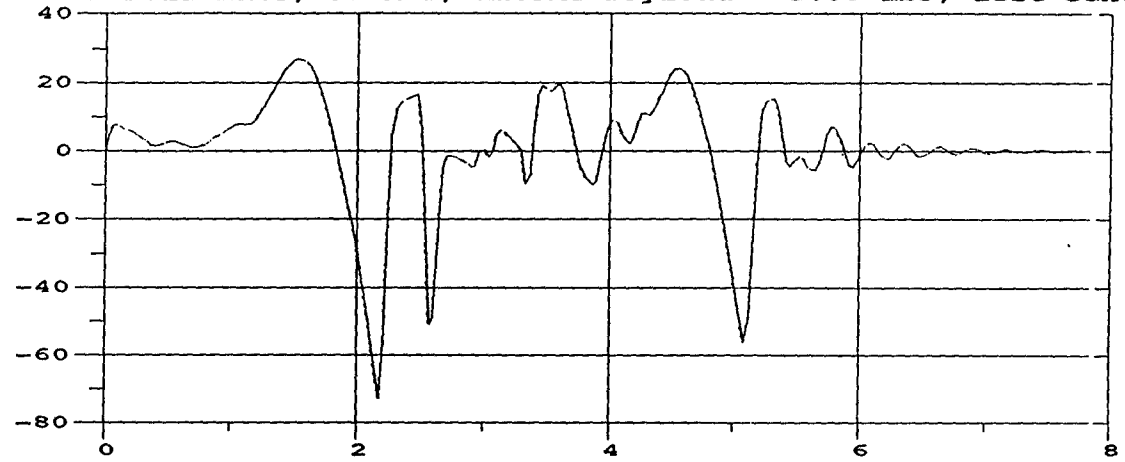
M105A2 Roll Rate; 35 MPH; M105A2 Payload = 3000 lbs, left center
