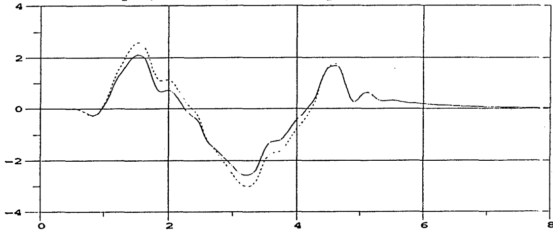
M105A2 Roll Angle; 35 MPH; M105A2 Payload = 1500 lbs, rear half
