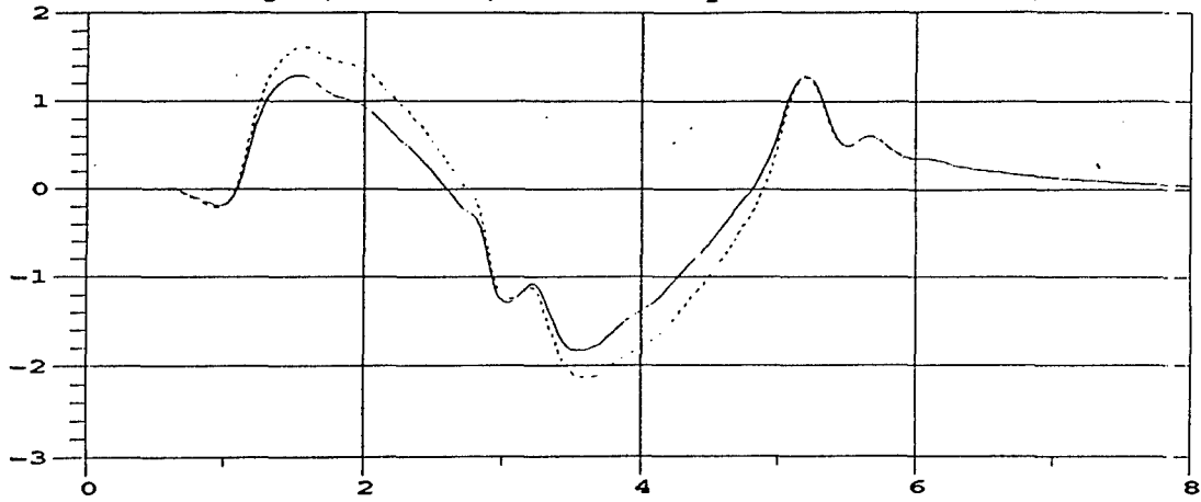
M105A2 Roll Angle; 30 MPH; M105A2 Payload = 1500 lbs, rear half
