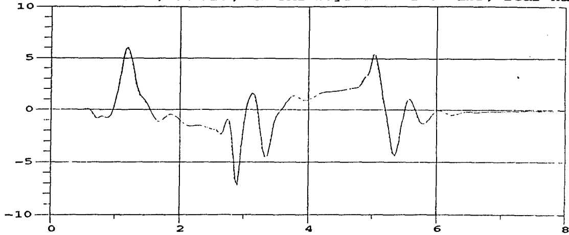
M105A2 Roll Rate; 30 MPH; M105A2 Payload = 1500 lbs, rear half
