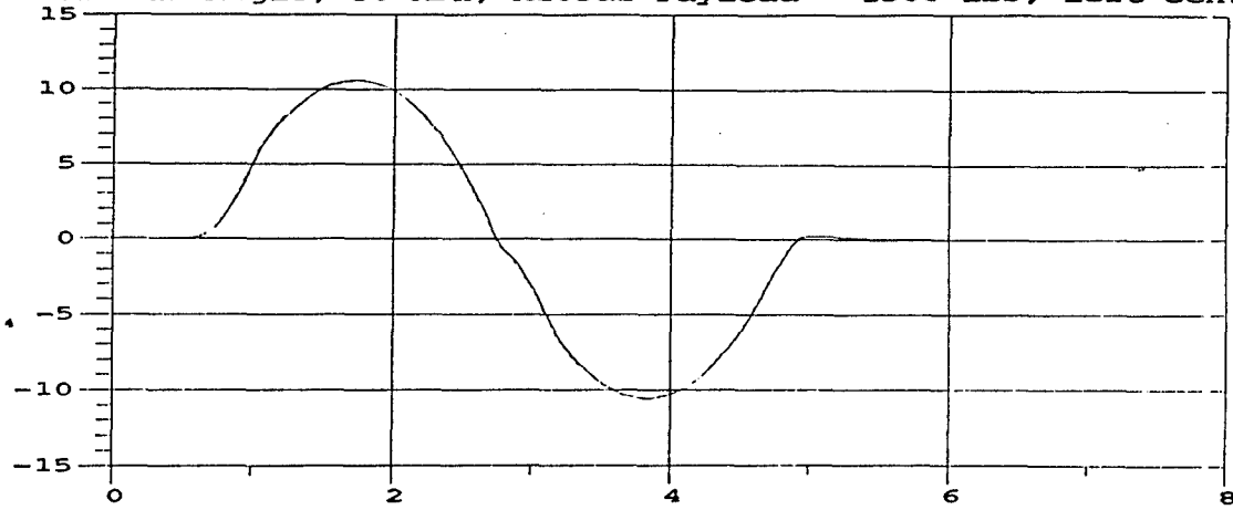
M35A2 Yaw Angle; 30 MPH; M105a2 Payload = 1500 lbs, left center
