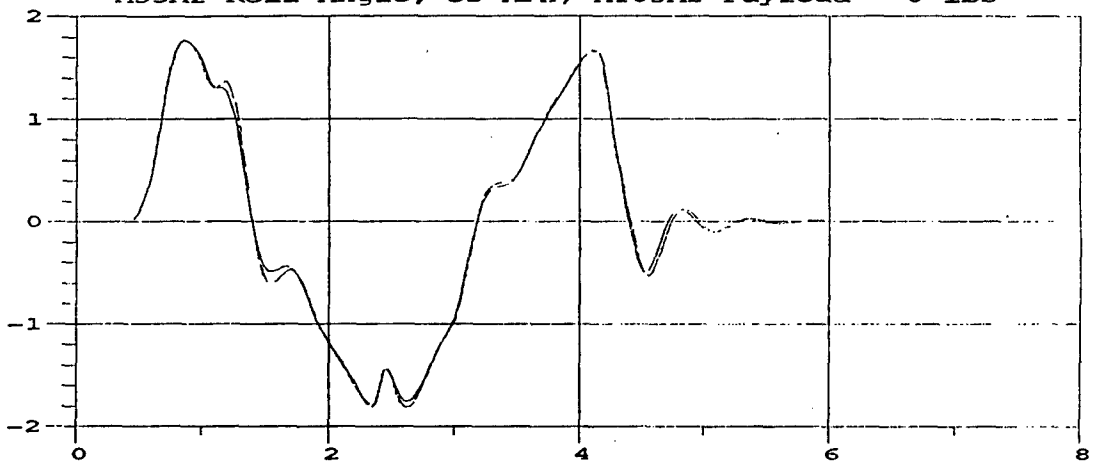
M35A2 Roll Angle; 35 MPH; M105A2 Payload = 0 lbs
