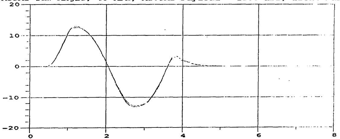
M35A2 Yaw Angle; 40 MPH; M105A2 Payload = 1500 lbs, front half
