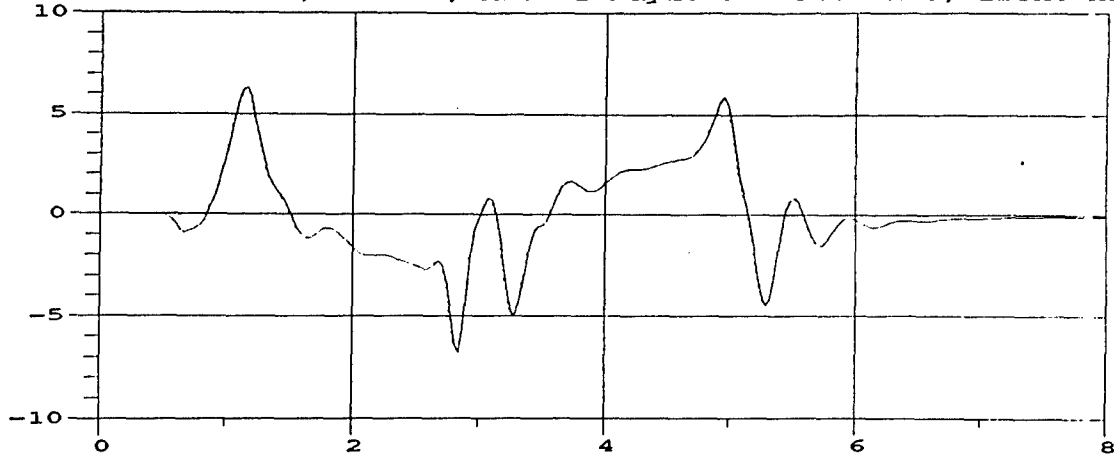
M105A2 Roll Rate; 30 MPH; M105A2 Payload = 3000 lbs, front half
