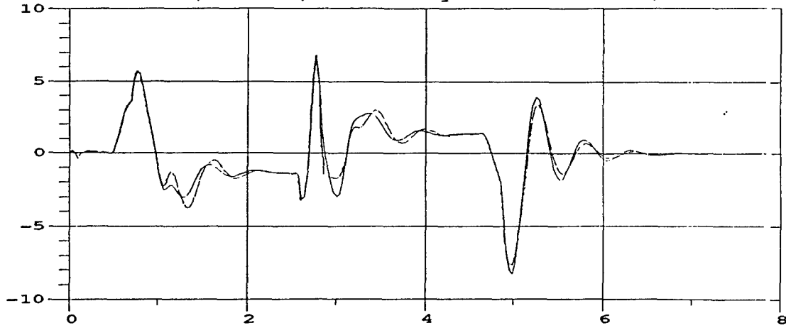
M35A2 Roll Rate; 30 MPH; M105A2 Payload = 3000 lbs, left center
