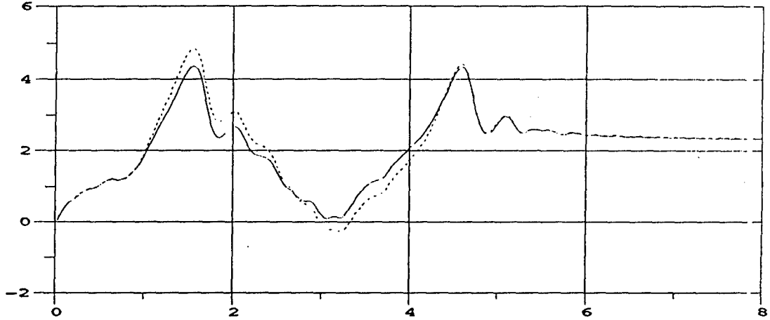
M105A2 Roll Angle; 35 MPH; M105a2 Payload = 1500 lbs, left center
