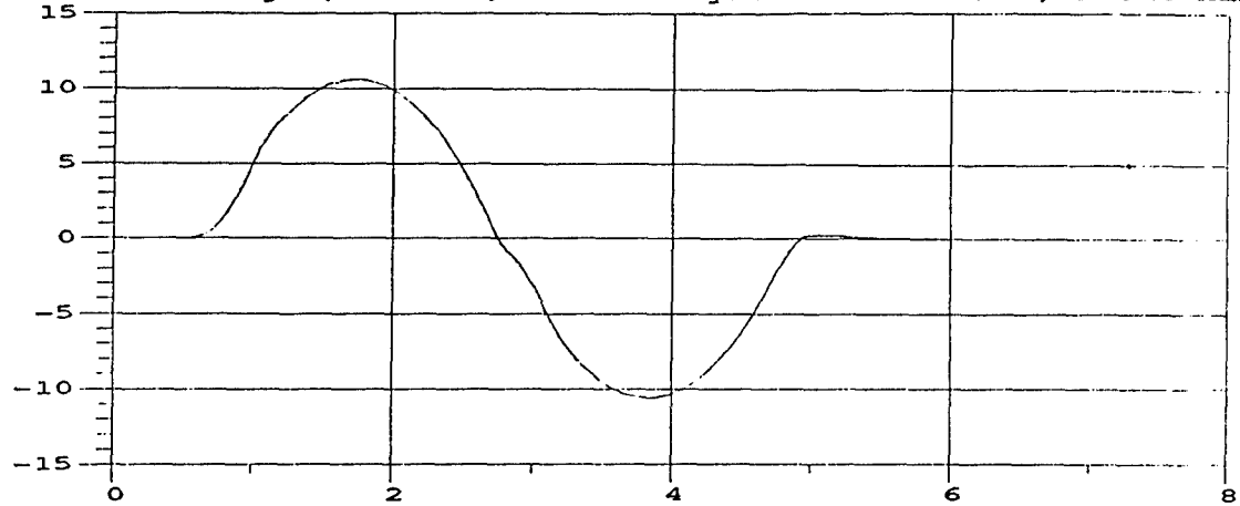
M35A2 Yaw Angle; 30 MPH; M105A2 Payload = 1500 lbs, front half
