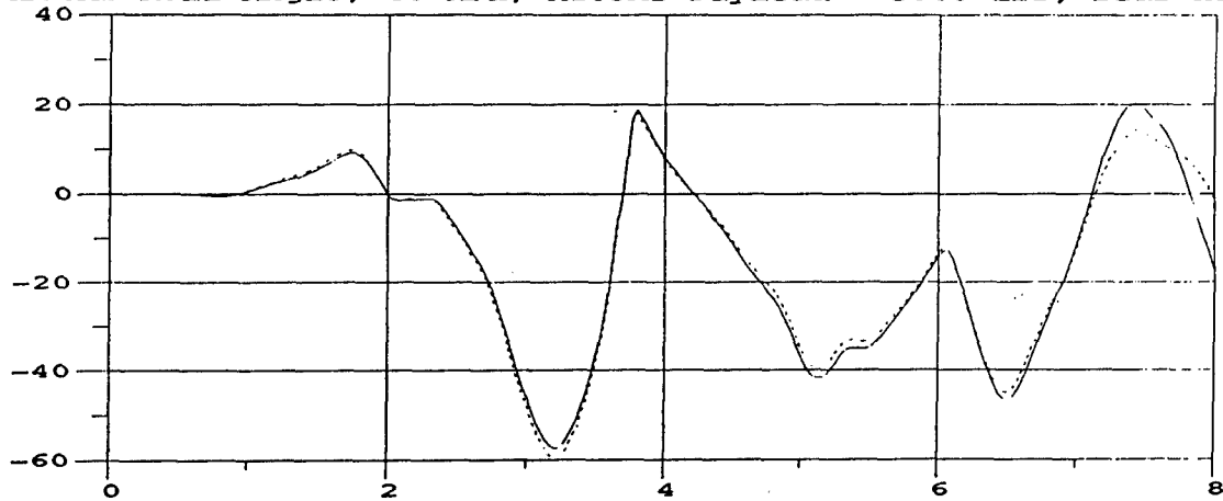
M105A2 Roll Angle; 40 MPH; M105A2 Payload = 3000 lbs, rear half
