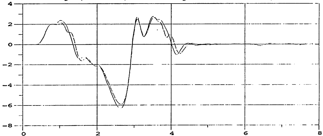
M35A2 Roll Angle; 40 MPH; M105A2 Payload = 3000 lbs, front half
