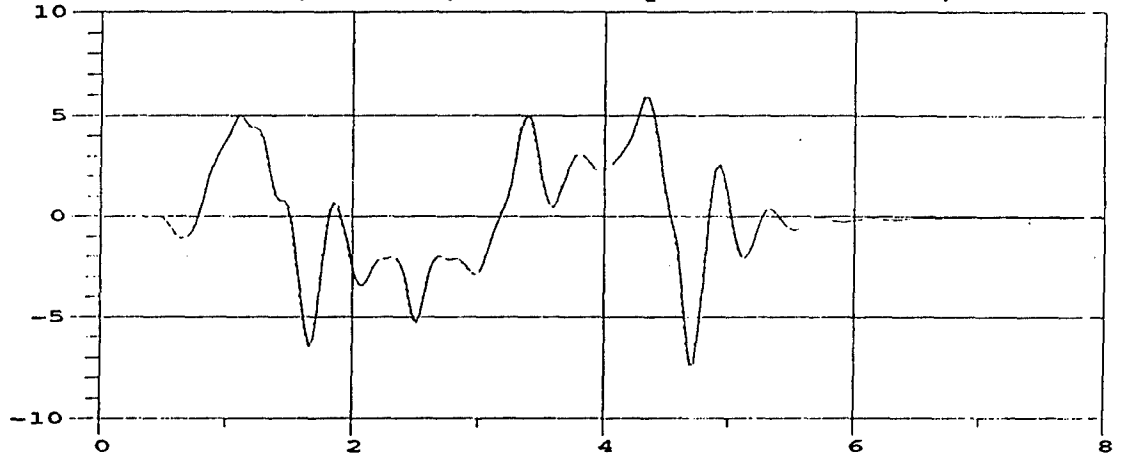
M105A2 Roll Rate; 35 MPH; M105A2 Payload = 1500 lbs, even dist.
