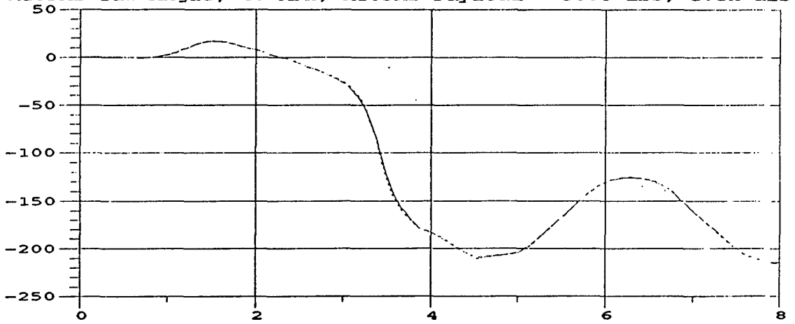
M105A2 Yaw Angle; 40 MPH; M105A2 Payload = 3000 lbs, even dist.
