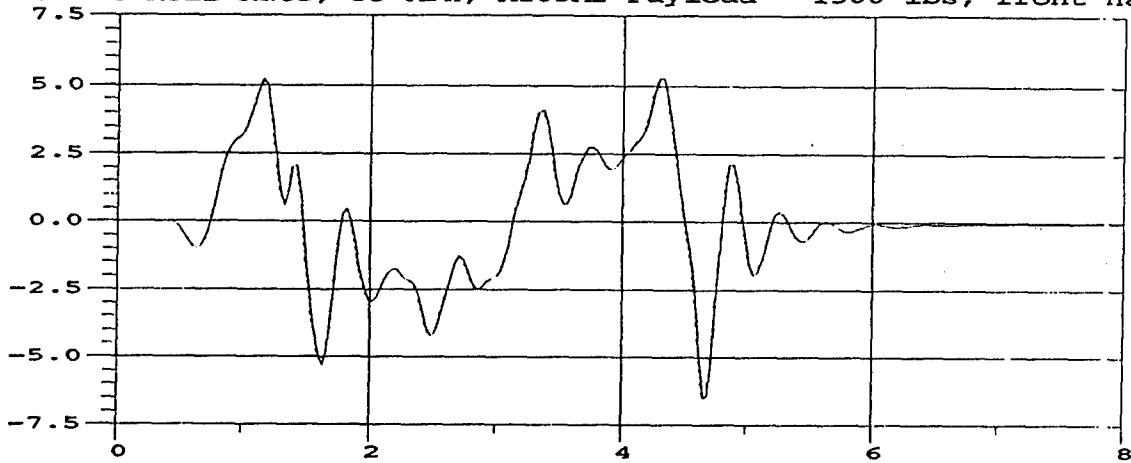
M105A2 Roll Rate; 35 MPH; M105A2 Payload = 1500 lbs, front half
