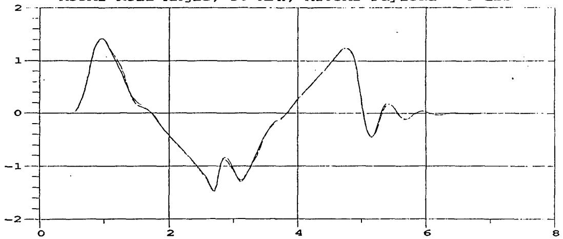
M35A2 Roll Angle; 30 MPH; M105A2 Payload = 0 lbs
