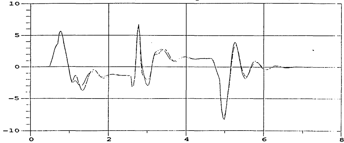
M35A2 Roll Rate; 30 MPH; M105A2 Payload = 3000 lbs, even dist.
