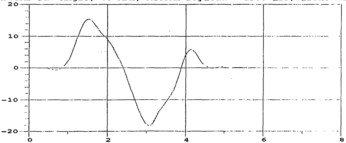
M105A2 Yaw Angle; 40 MPH; M105A2 Payload = 1500 lbs, front half
