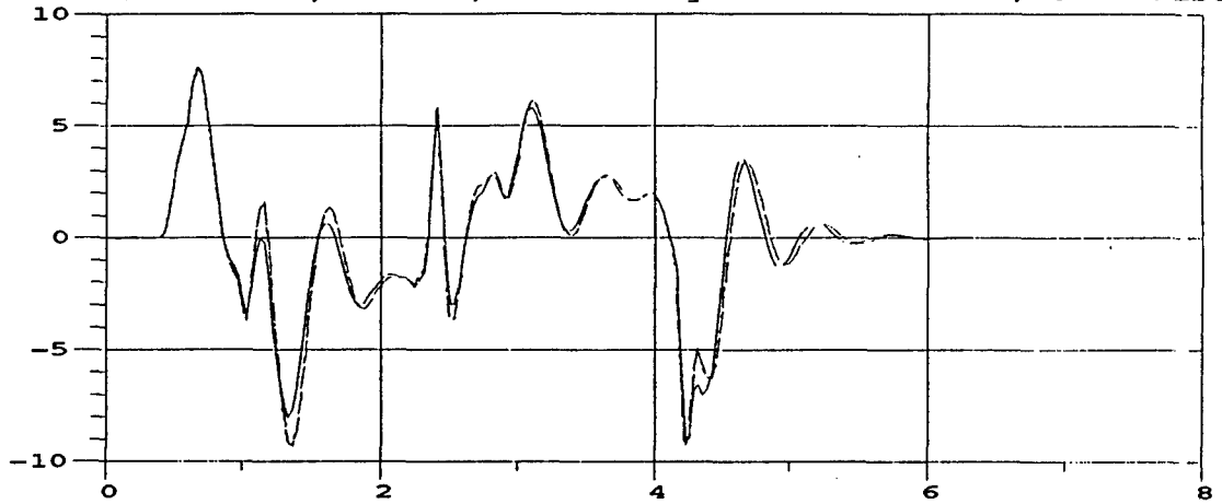
M35A2 Roll Rate; 35 MPH; M105A2 Payload = 1500 lbs, even dist.
