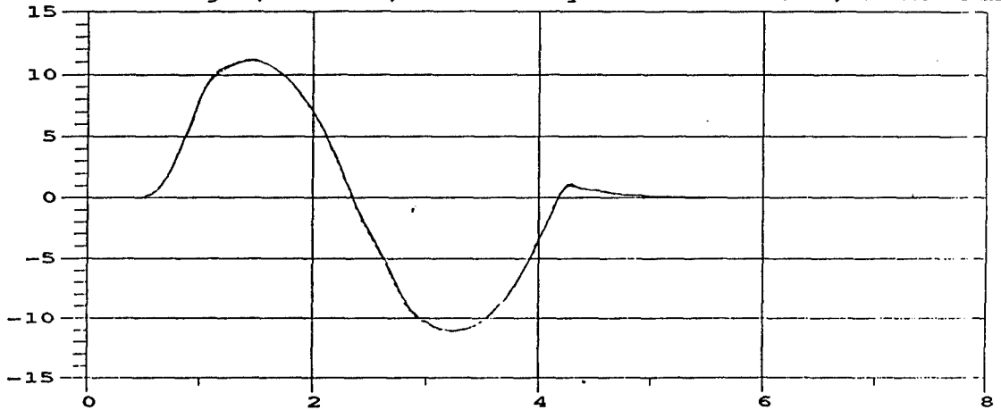
M35A2 Yaw Angle; 35 MPH; M105A2 Payload = 1500 lbs, front half
