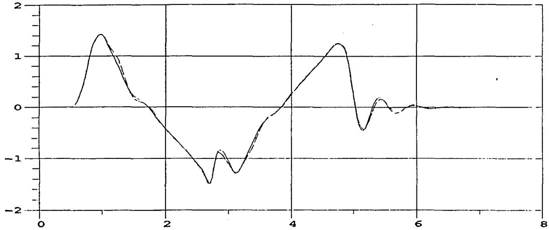
M35A2 Roll Angle; 30 MPH; M105A2 Payload = 3000 lbs, even dist.
