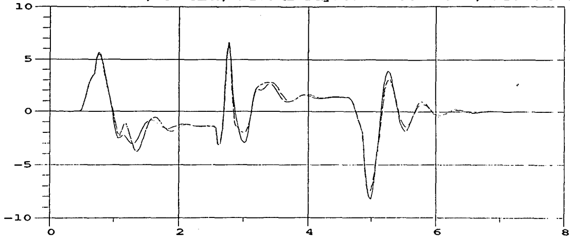
M35A2 Roll Rate; 30 MPH; M105A2 Payload = 3000 lbs, front half
