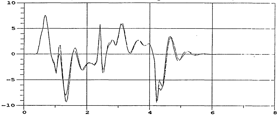
M35A2 Roll Rate; 35 MPH; M105A2 Payload = 3000 lbs, even dist.
