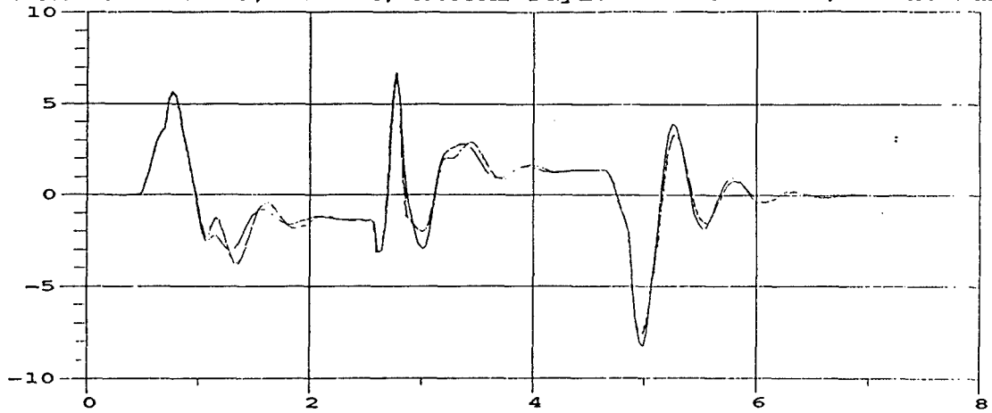
M35A2 Roll Rate; 30 MPH; M105A2 Payload = 1500 lbs, front half
