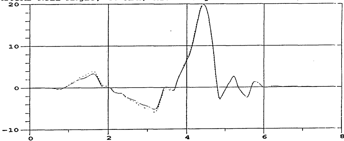
M105A2 Roll Angle; 40 MPH; M105A2 Payload = 1500 lbs, rear half
