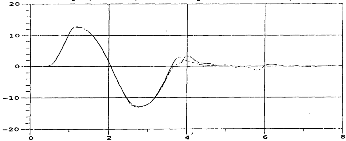
M35A2 Yaw Angle; 40 MPH; M105A2 Payload = 3000 lbs, even dist.
