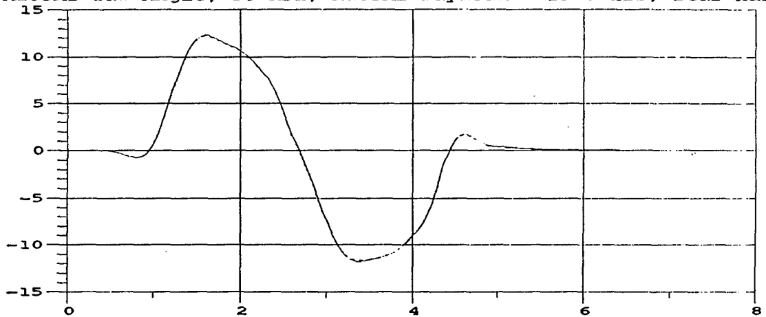
M105A2 Yaw Angle; 35 MPH; M105A2 Payload = 1500 lbs, rear half
