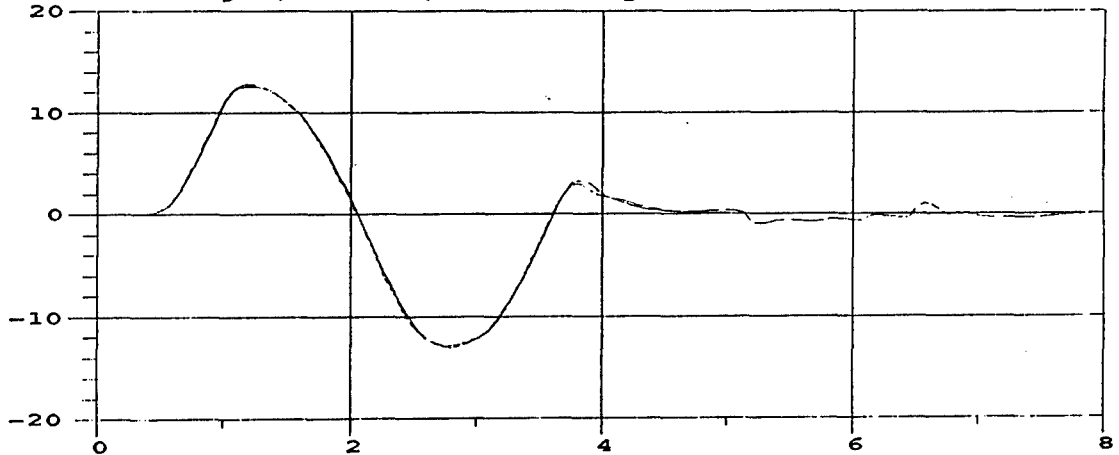
M35A2 Yaw Angle; 40 MPH; M105a2 Payload = 1500 lbs, left center
