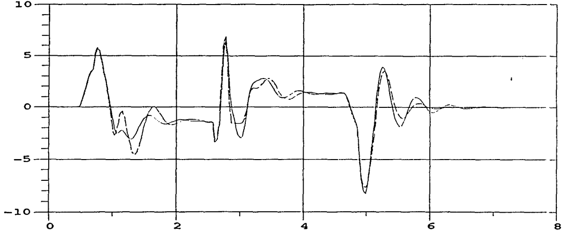
M35A2 Roll Rate; 30 MPH; M105A2 Payload = 3000 lbs, rear half
