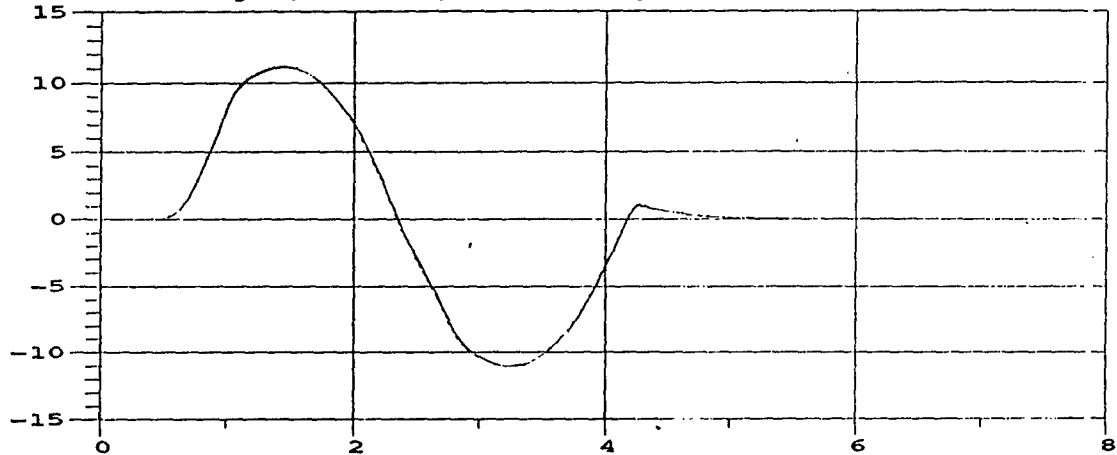
M35A2 Yaw Angle; 35 MPH; M105A2 Payload = 1500 lbs, even dist.
