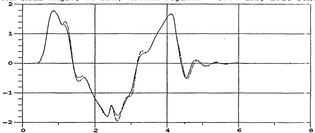
M35A2 Roll Angle; 35 MPH; M105A2 Payload = 3000 lbs, left center
