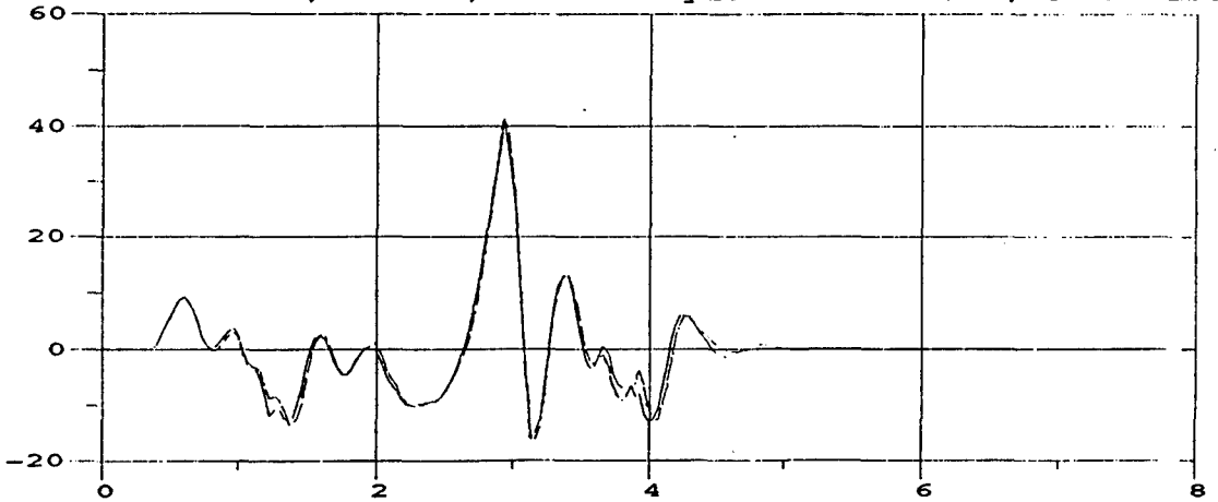
M35A2 Roll Rate; 40 MPH; M105A2 Payload = 1500 lbs, even dist.
