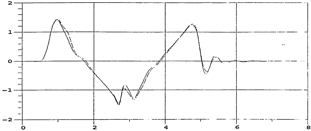
M35A2 Roll Angle; 30 MPH; M105A2 Payload = 3000 lbs, front half
