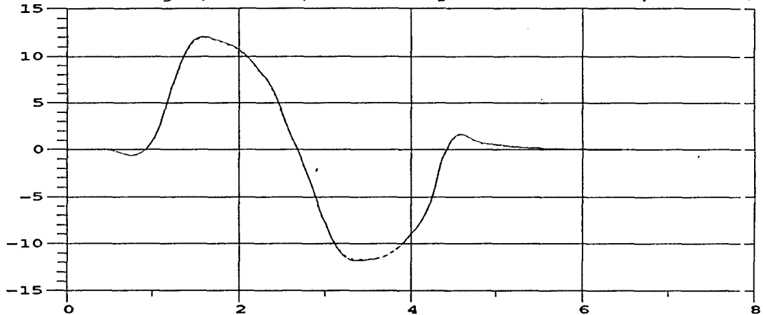
M105A2 Yaw Angle; 35 MPH; M105A2 Payload = 3000 lbs, front half
