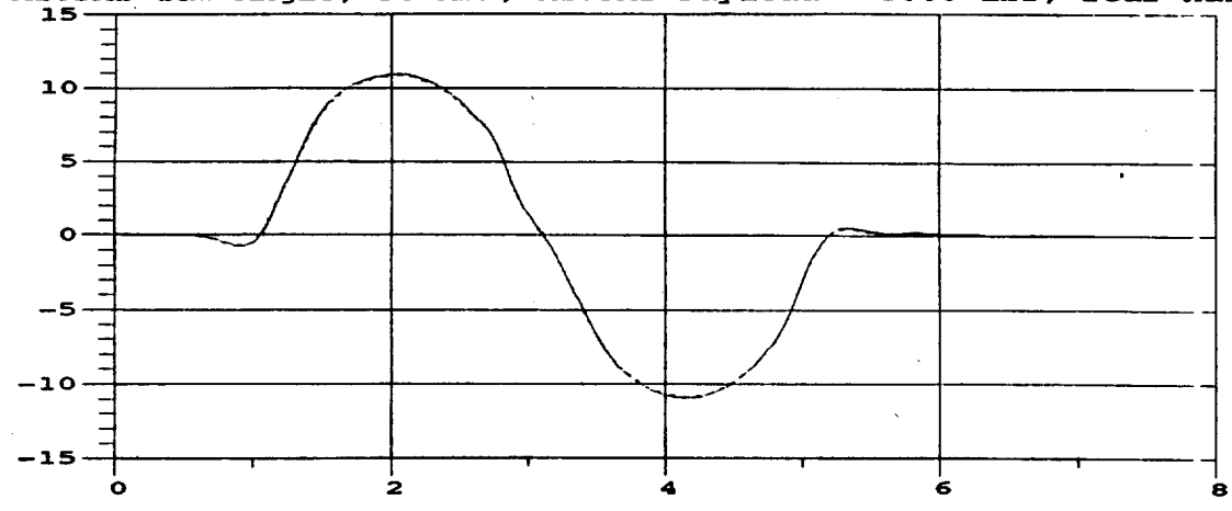
M105A2 Yaw Angle; 30 MPH; M105A2 Payload = 3000 lbs, rear half
