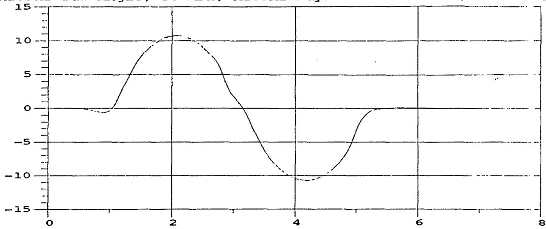
M105A2 Yaw Angle; 30 MPH; M105A2 Payload = 1500 lbs, even dist.
