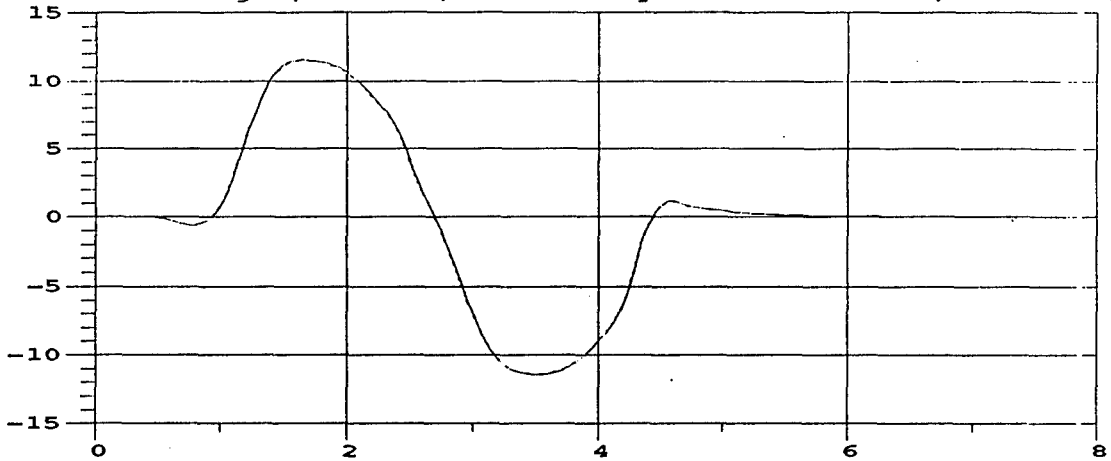
M105A2 Yaw Angle; 35 MPH; M105A2 Payload = 1500 lbs, front half
