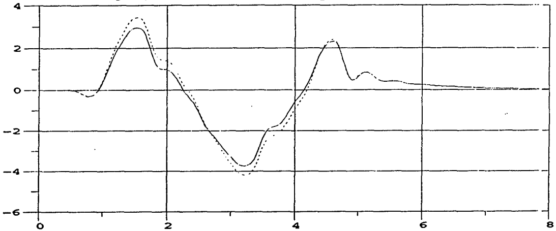
M105A2 Roll Angle; 35 MPH; M105A2 Payload = 3000 lbs, even dist.
