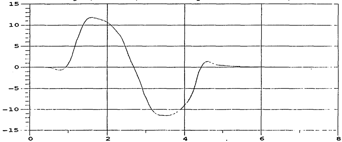
M105A2 Yaw Angle; 35 MPH; M105A2 Payload = 1500 lbs, even dist.
