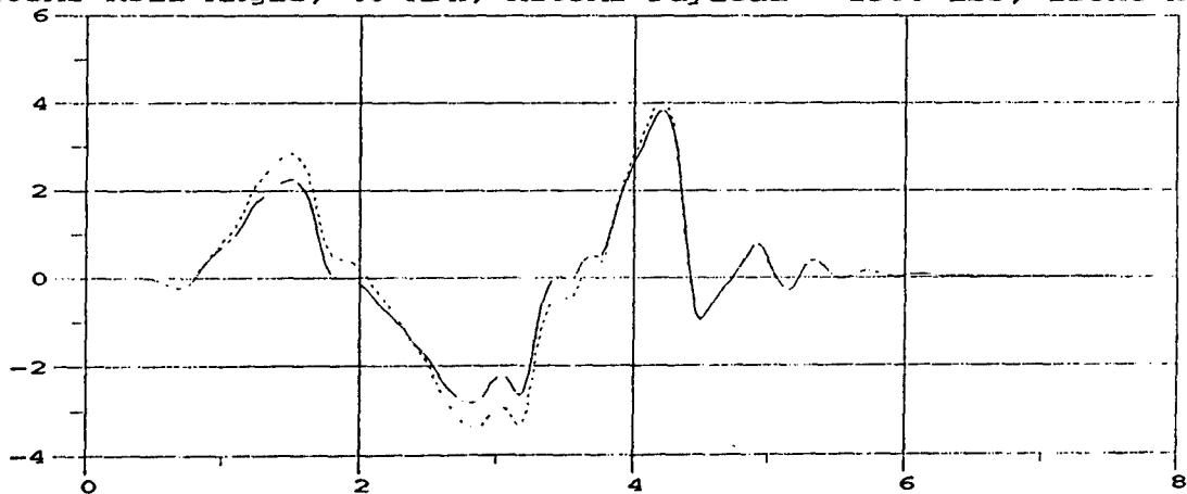
M105A2 Roll Angle; 40 MPH; M105A2 Payload = 1500 lbs, front half
