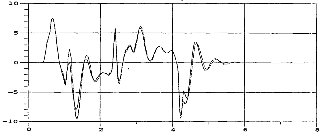
M35A2 Roll Rate; 35 MPH; M105A2 Payload = 1500 lbs, front half
