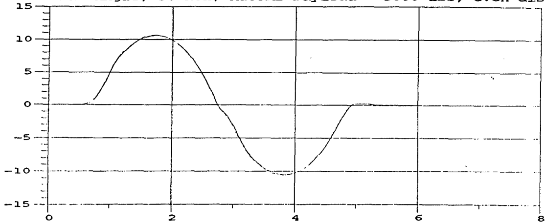
M35A2 Yaw Angle; 30 MPH; M105A2 Payload = 3000 lbs, even dist.
