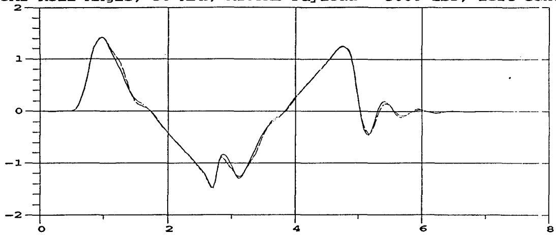
M35A2 Roll Angle; 30 MPH; M105A2 Payload = 3000 lbs, left center
