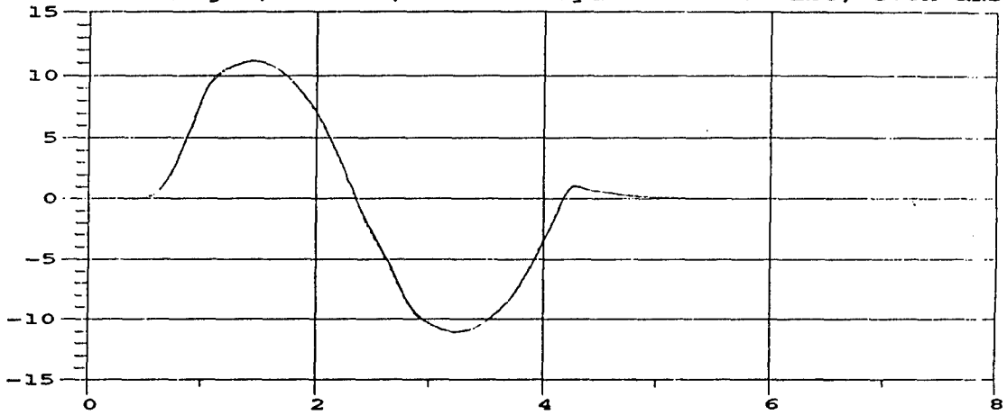
M35A2 Yaw Angle; 35 MPH; M105A2 Payload = 3000 lbs, even dist.
