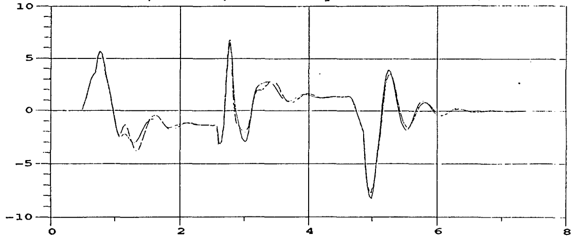
M35A2 Roll Rate; 30 MPH; M105A2 Payload = 1500 lbs, even dist.
