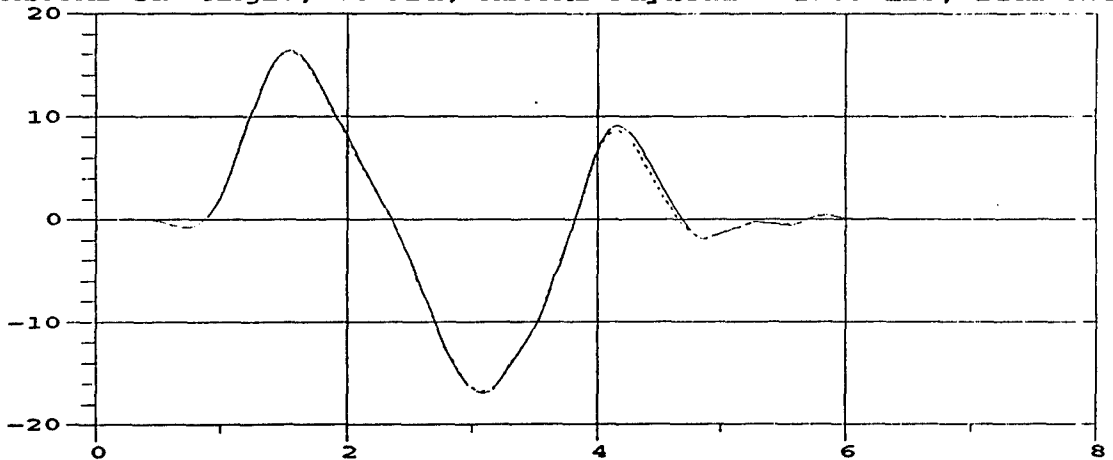
M105A2 Yaw Angle; 40 MPH; M105A2 Payload = 1500 lbs, rear half
