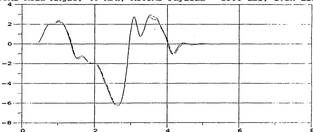
M35A2 Roll Angle; 40 MPH; M105A2 Payload = 1500 lbs, even dist.
