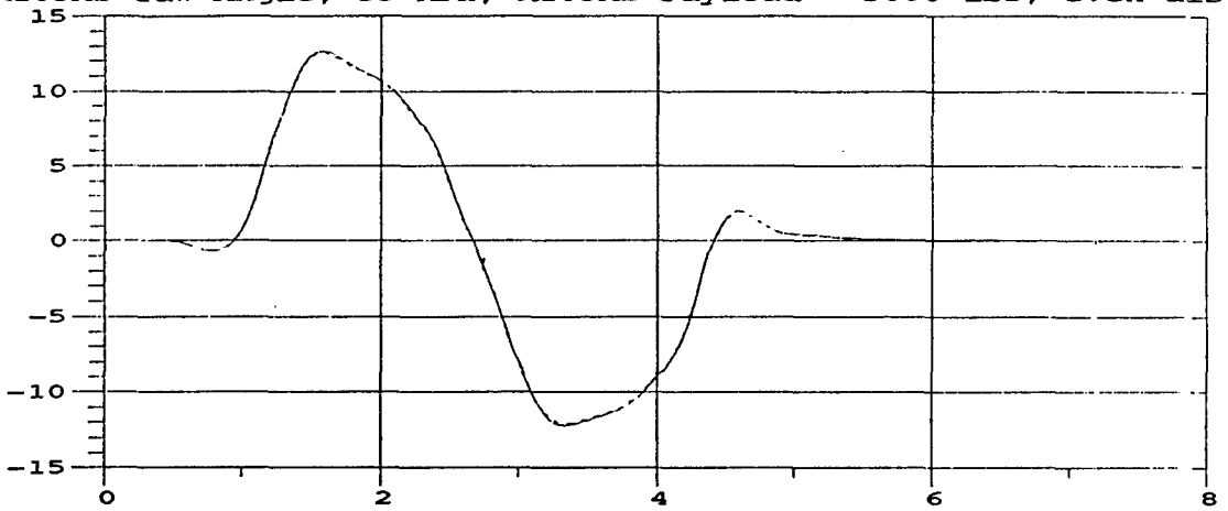
M105A2 Yaw Angle; 35 MPH; M105A2 Payload = 3000 lbs, even dist.
