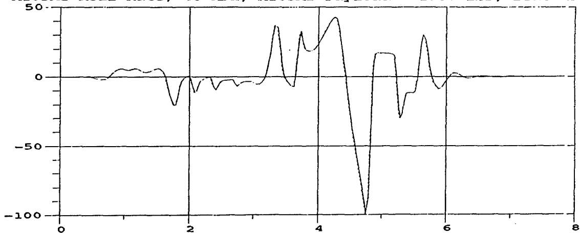
M105A2 Roll Rate; 40 MPH; M105A2 Payload = 1500 lbs, rear half
