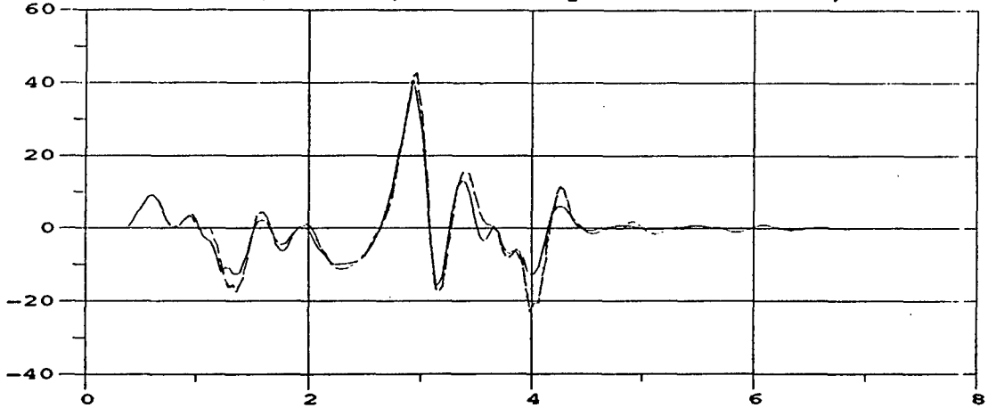
M35A2 Roll Rate; 40 MPH; M105A2 Payload = 1500 lbs, rear half
