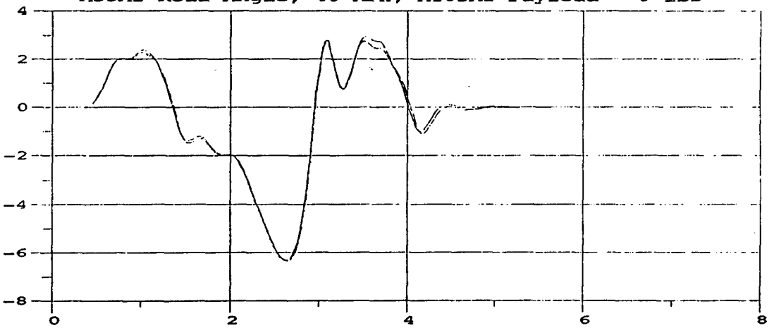
M35A2 Roll Angle; 40 MPH; M105A2 Payload = 0 lbs
