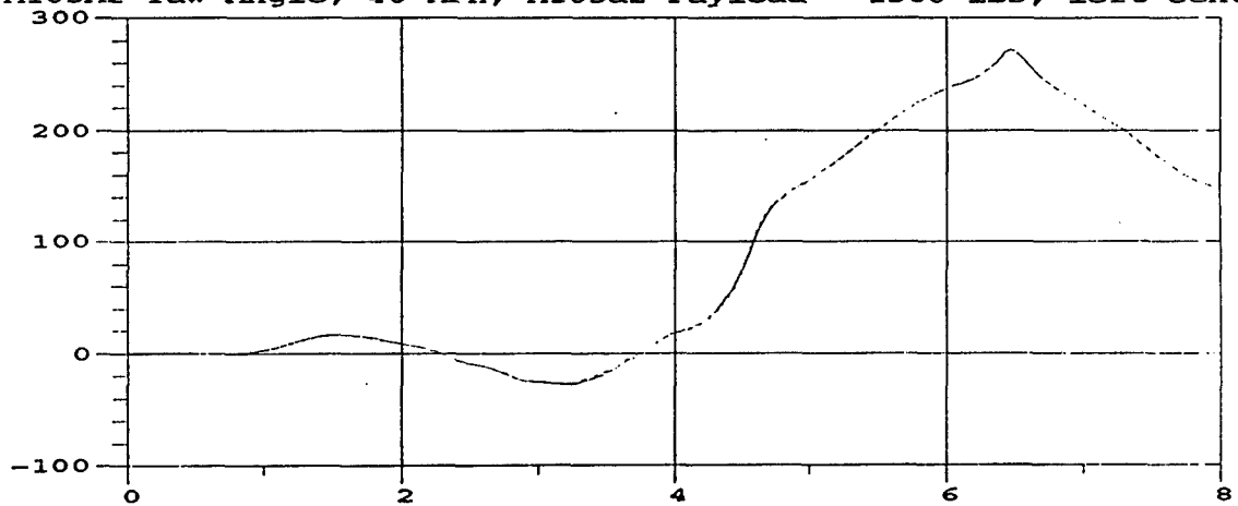
M105A2 Yaw Angle; 40 MPH; M105a2 Payload = 1500 lbs, left center
