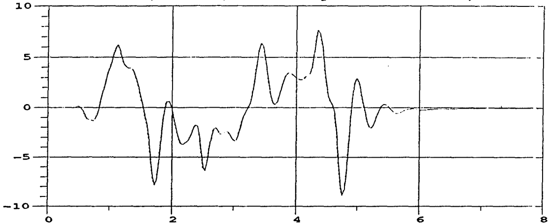
M105A2 Roll Rate; 35 MPH; M105A2 Payload = 1500 lbs, rear half
