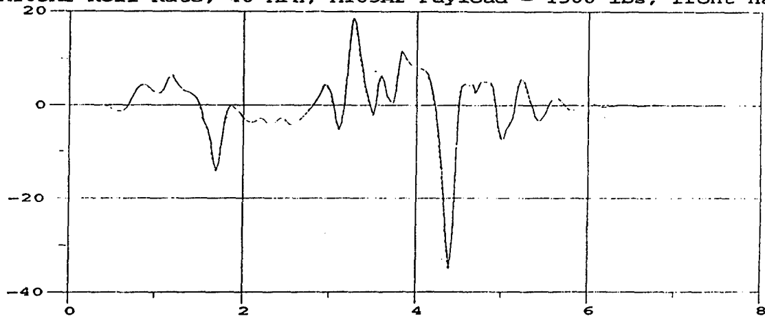
M105A2 Roll Rate; 40 MPH; M105A2 Payload = 1500 lbs, front half
