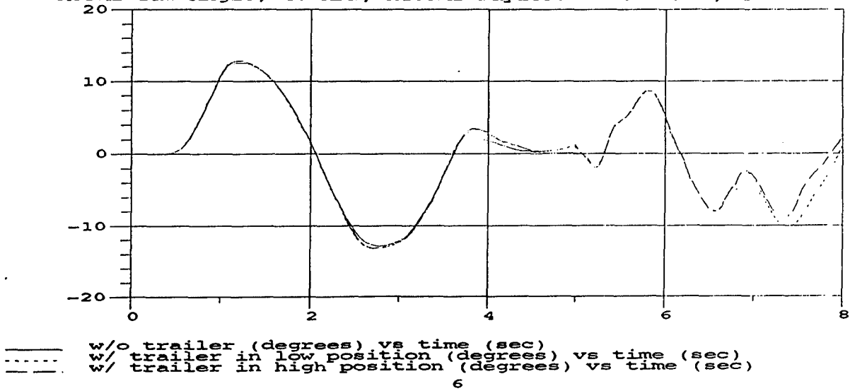
M35A2 Yaw Angle; 40 MPH; M105A2 Payload = 3000 lbs, left center
