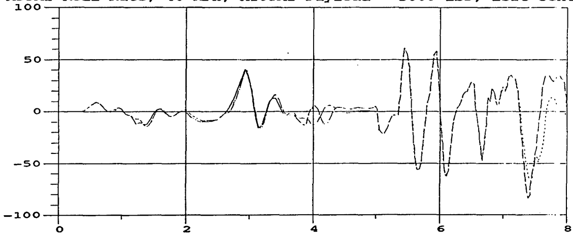
M35A2 Roll Rate; 40 MPH; M105A2 Payload = 3000 lbs, left center
