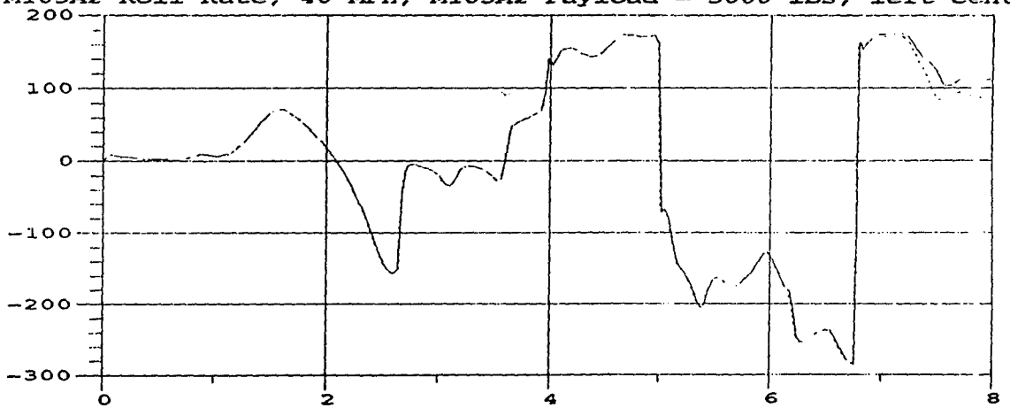
M105A2 Roll Rate; 40 MPH; M105A2 Payload = 3000 lbs, left center
