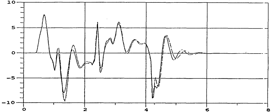
M35A2 Roll Rate; 35 MPH; M105A2 Payload = 1500 lbs, rear half
