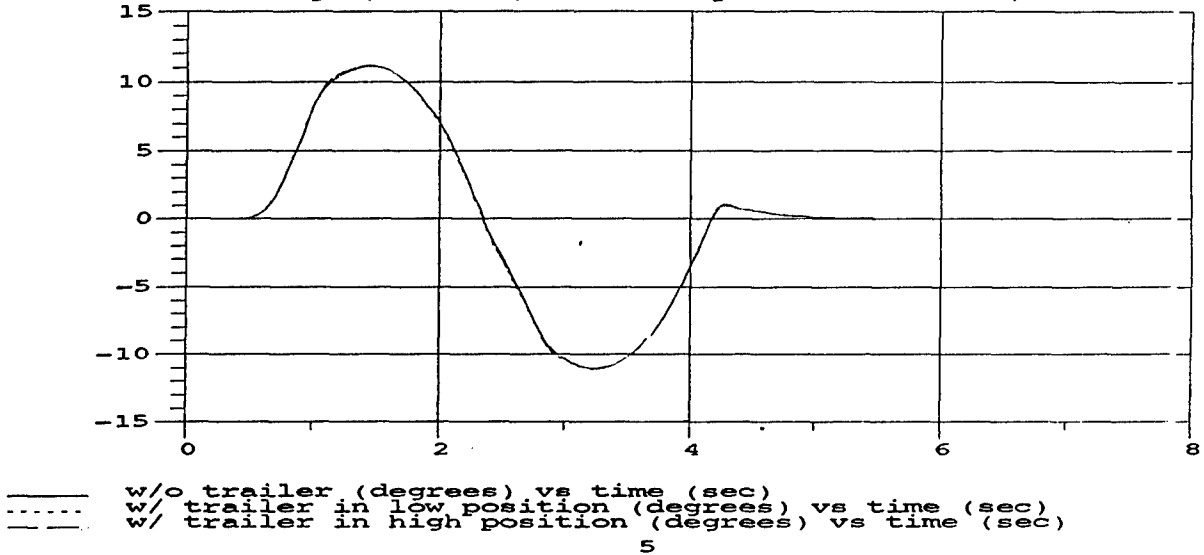
M35A2 Yaw Angle; 40 MPH; M105A2 Payload = 3000 lbs, left center
