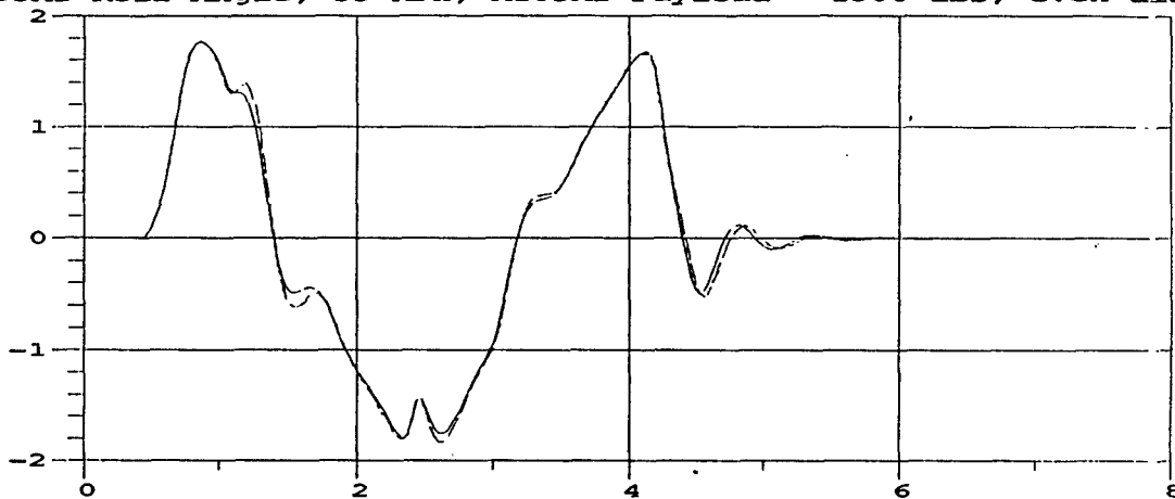
M35A2 Roll Angle; 35 MPH; M105A2 Payload = 1500 lbs, even dist.
