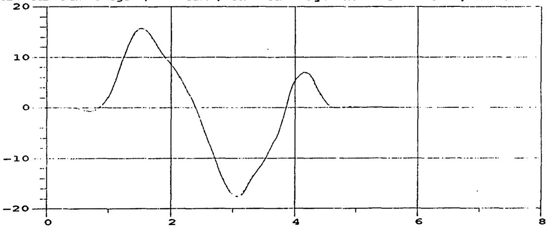
M105A2 Yaw Angle; 40 MPH; M105A2 Payload = 1500 lbs, even dist.
