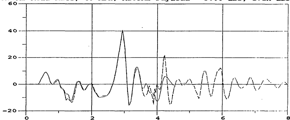
M35A2 Roll Rate; 40 MPH; M105A2 Payload = 3000 lbs, even dist.
