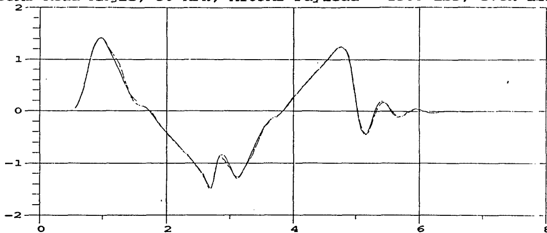
M35A2 Roll Angle; 30 MPH; M105A2 Payload = 1500 lbs, even dist.
