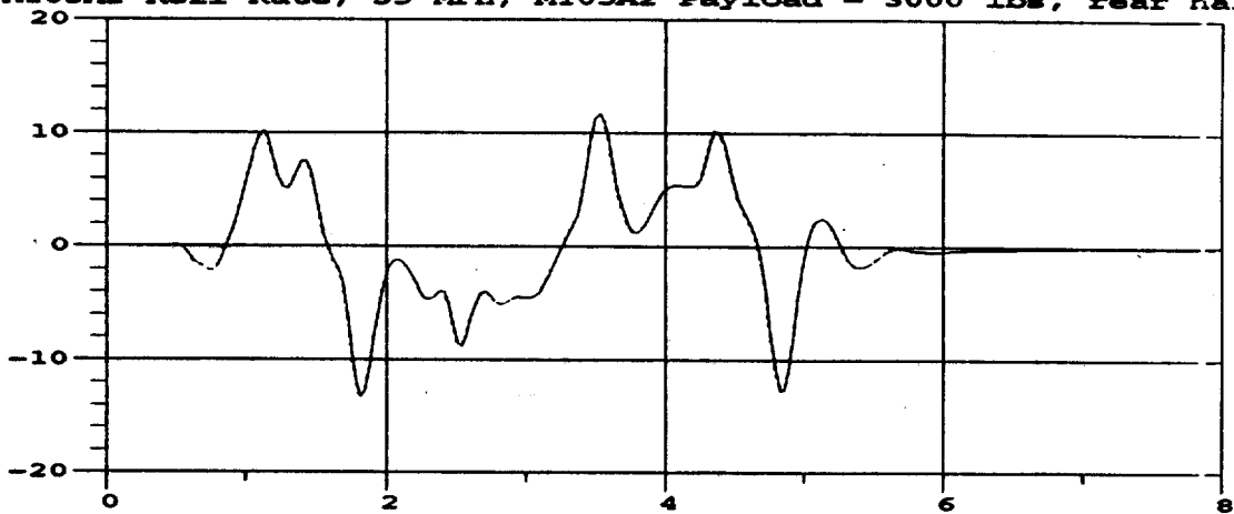
M105A2 Roll Rate; 35 MPH; M105A2 Payload = 3000 lbs, rear half
