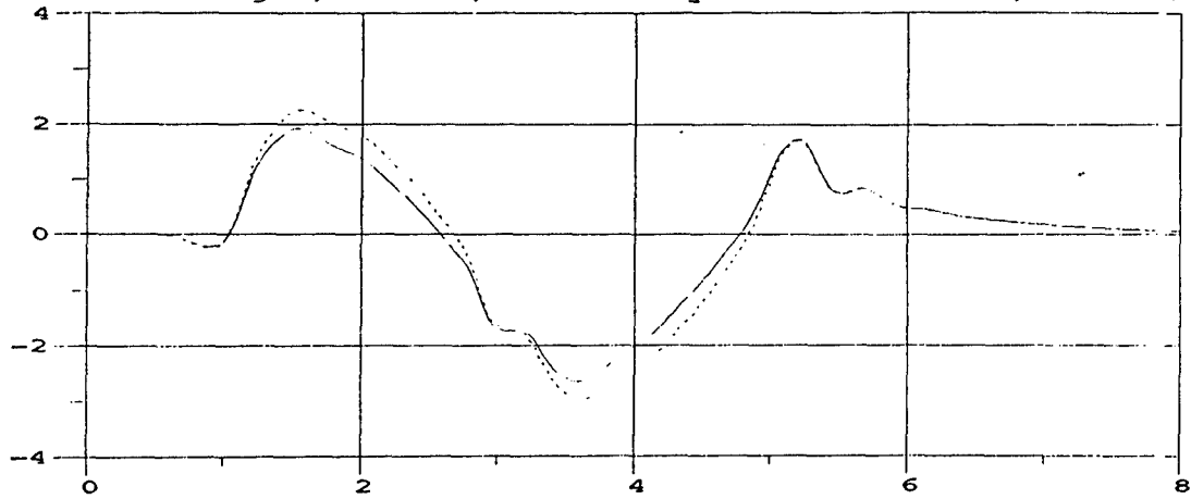
M105A2 Roll Angle; 30 MPH; M105A2 Payload = 3000 lbs, even dist.
