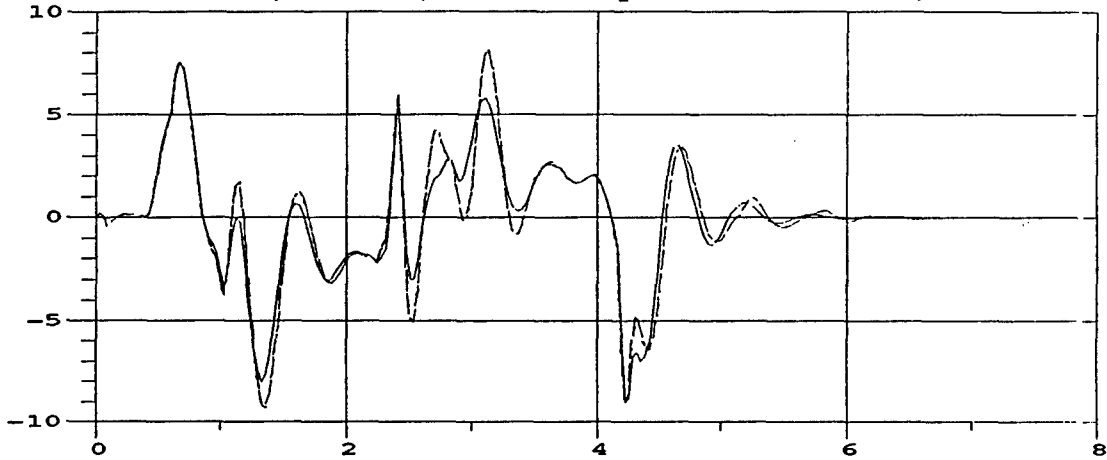
M35A2 Roll Rate; 35 MPH; M105A2 Payload = 3000 lbs, left center
