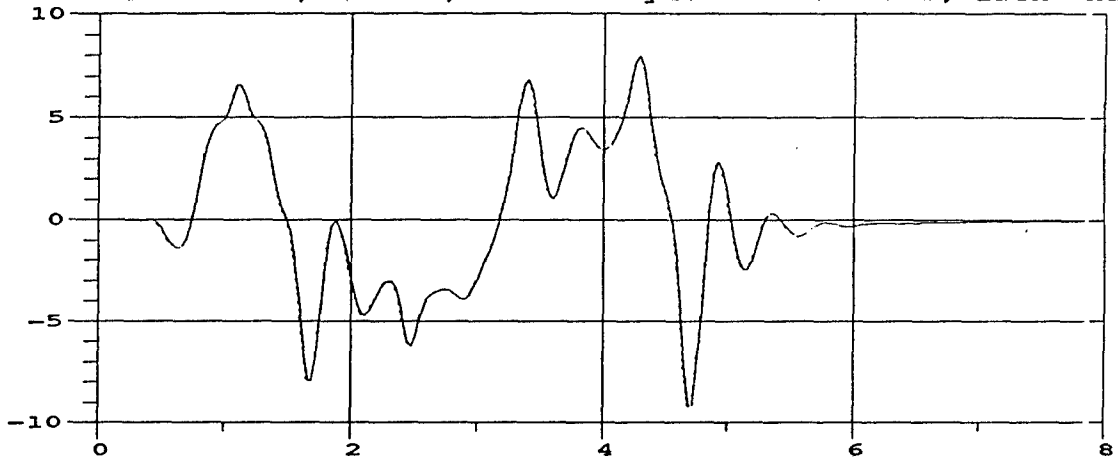
M105A2 Roll Rate; 35 MPH; M105A2 Payload = 3000 lbs, front half
