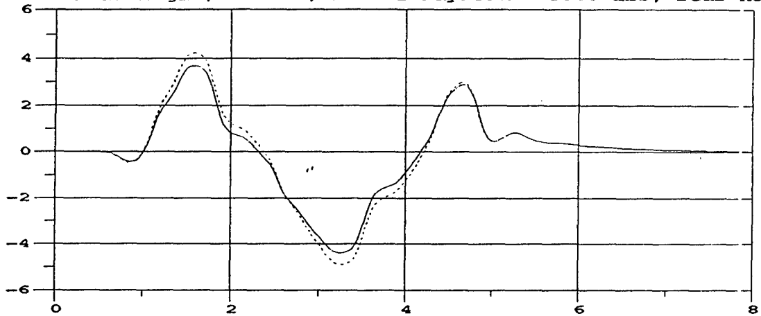
M105A2 Roll Angle; 35 MPH; M105A2 Payload = 3000 lbs, rear half
