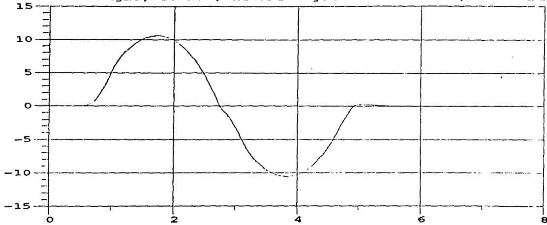
M35A2 Yaw Angle; 30 MPH; M105A2 Payload = 1500 lbs, even dist.
