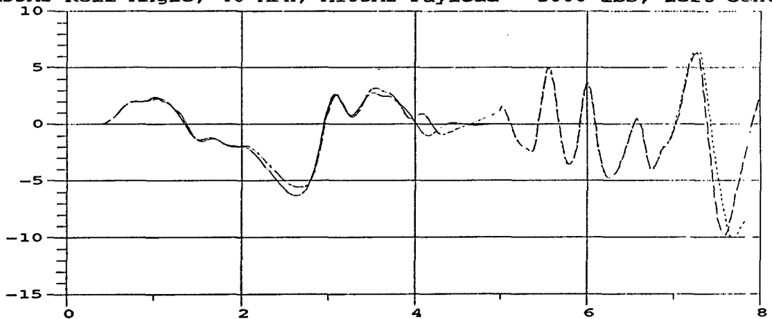
M35A2 Roll Angle; 40 MPH; M105A2 Payload = 3000 lbs, left center
