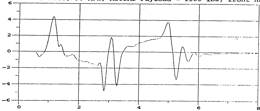
M105A2 Roll Rate; 30 MPH; M105A2 Payload = 1500 lbs, front half
