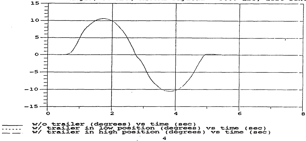
M35A2 Yaw Angle; 35 MPH; M105A2 Payload = 3000 lbs, left center
