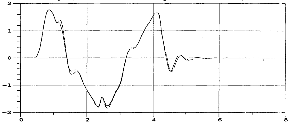
M35A2 Roll Angle; 35 MPH; M105A2 Payload = 3000 lbs, even dist.
