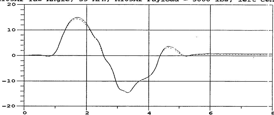
M105A2 Yaw Angle; 35 MPH; M105A2 Payload = 3000 lbs, left center
