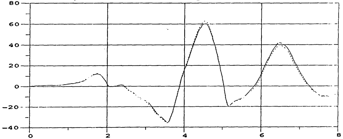
M105A2 Roll Angle; 40 MPH; M105a2 Payload = 1500 lbs, left center
