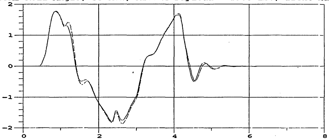
M35A2 Roll Angle; 35 MPH; M105A2 Payload = 1500 lbs, front half
