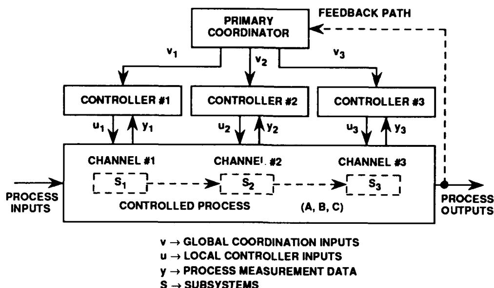
FIGURE 17. DECENTRALIZED MULTILEVEL CONTROL
