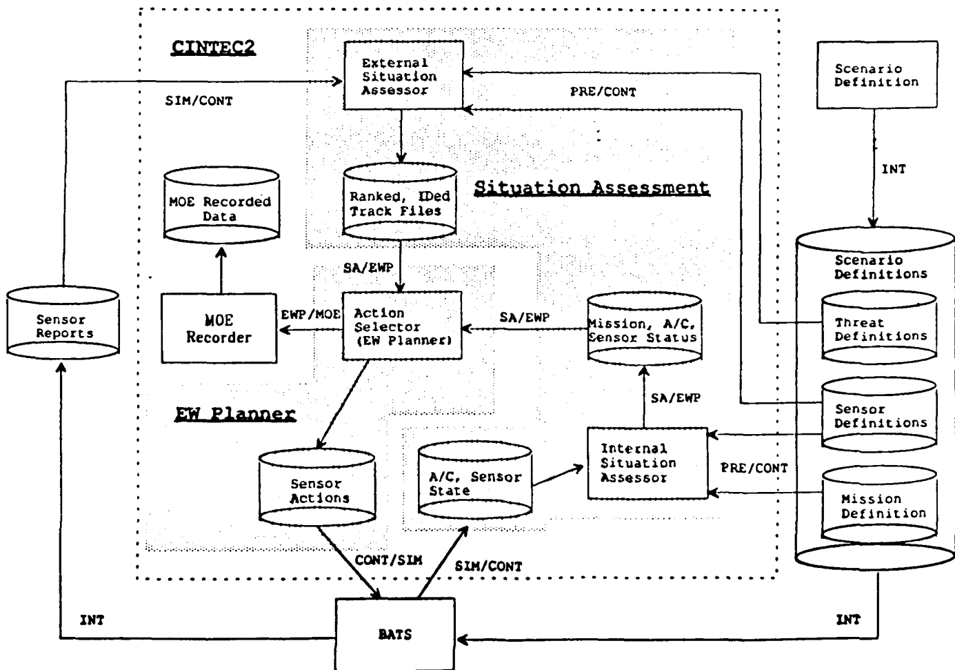
Figure 5 - CINTEC2 Functional Block Diagram
