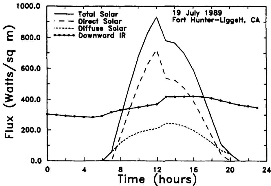
Figure 13. Average Hourly Solar and Infrared Fluxes for 19 July 1989 at Fort Hunter-Liggett, California as Calculated with the IARTP
