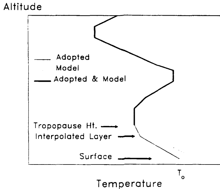
Figure 11. Adopted Temperature Profile When Model Atmosphere Profiles Are Shifted To Match Surface Values. Temperature and altitude axes are for instructive purposes and are not drawn to scale. T_o is the observed surface temperature
