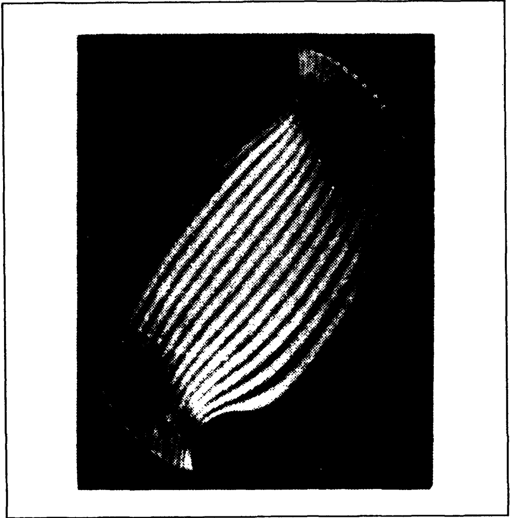
Photograph of a 1 cm diameter AT-cut resonator and its X-ray topograph. The topograph shows the lattice distortion due to the mounting stresses.
