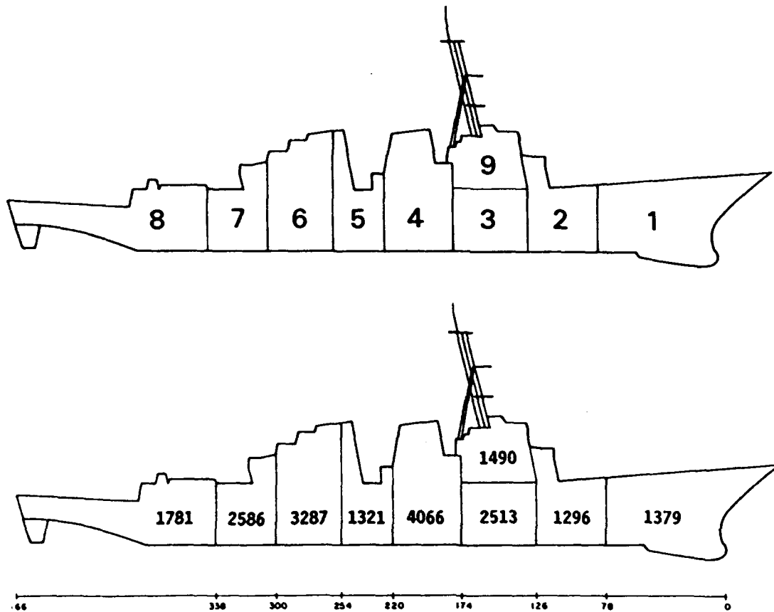
TOTAL CONNECTED 60 HZ LOAD (AMPS) 450V-3PH FOR DISTRIBUTION
