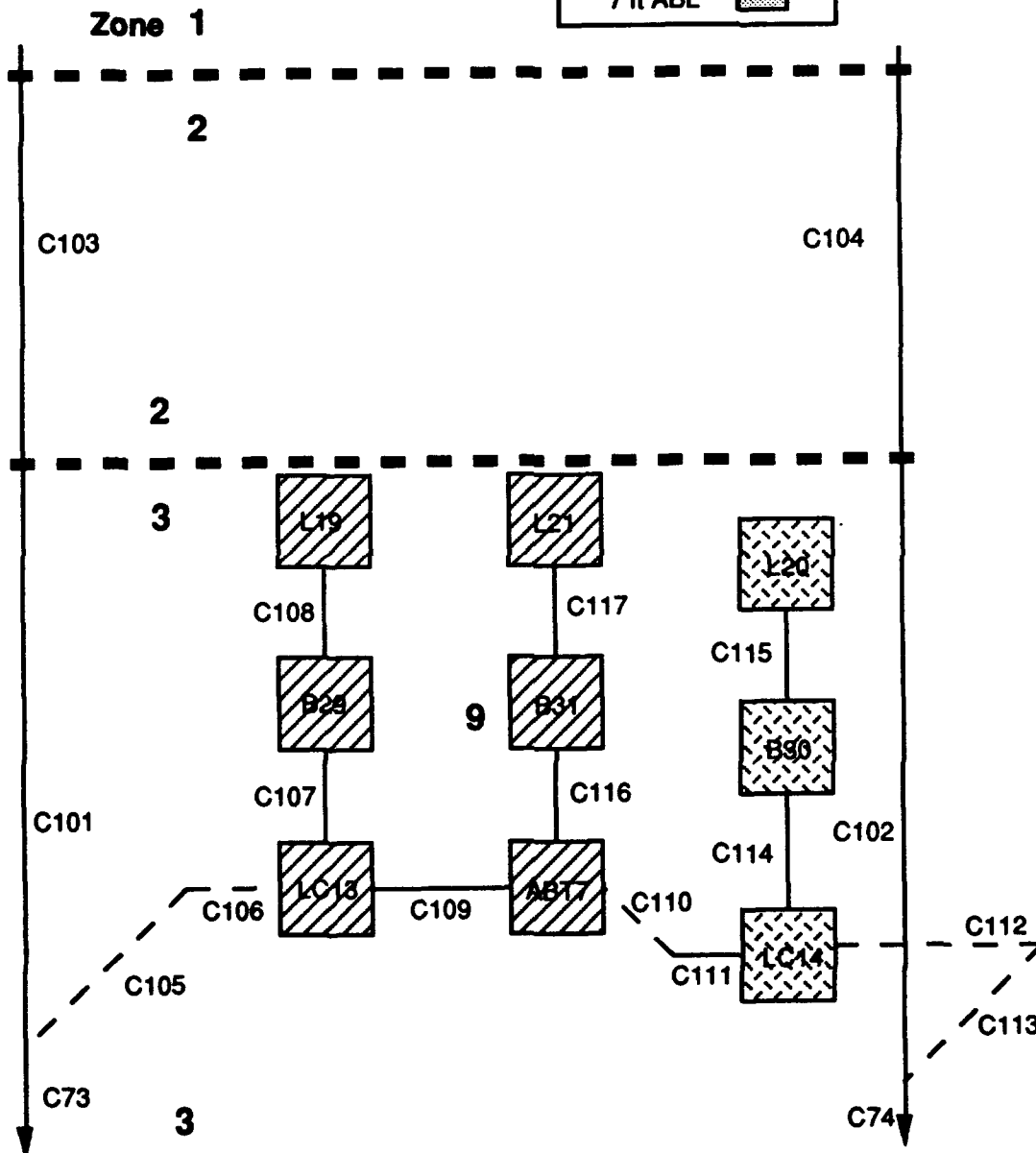
Figure 10. System Interconnection Diagram for Zones 1 - 3 and 9.
