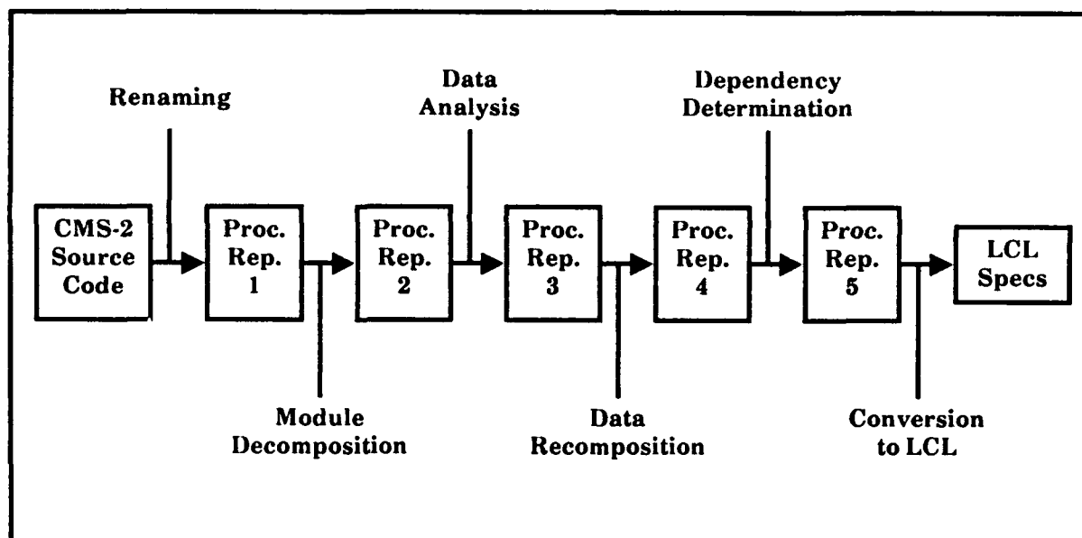
FIGURE 5. TRANSFORMATION OF THE PROCEDURAL REPRESENTATION
