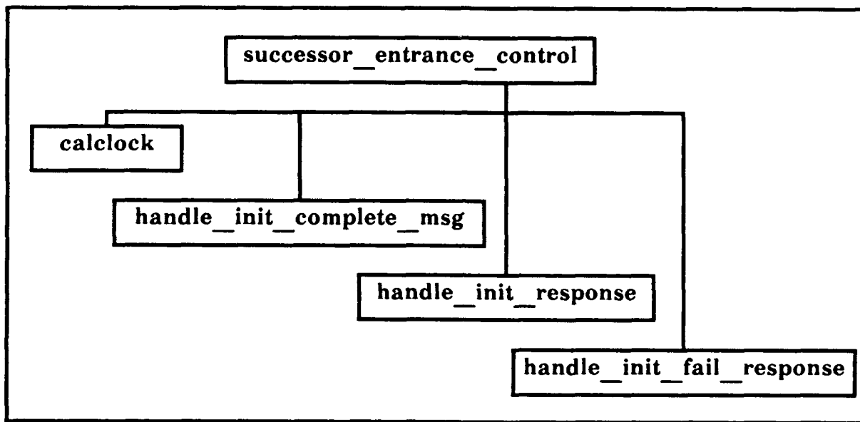
FIGURE 8. THE NEW STRUCTURE OF RCINSUCC AFTER RENAMING AND MODULAR DECOMPOSITION
