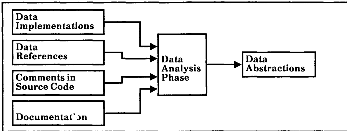
FIGURE 13. INTEGRATION OF DATA ANALYSIS INFORMATION
