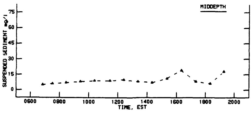
SUSPENDED SEDIMENT AT STATION 4D 7 MAY 1990
