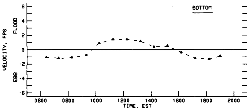
VELOCITIES AT STATION 8C 8 MAY 1990
