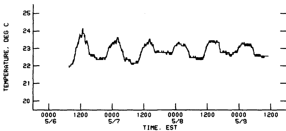
VELOCITY, TEMPERATURE, AND SALINITY AT STATION S1.0 6-9 MAY 1990
