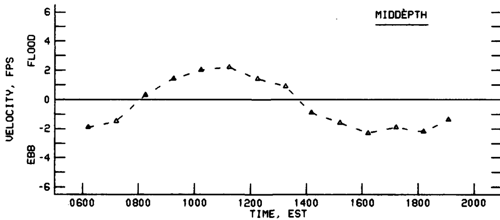
VELOCITIES AT STATION 4C 8 MAY 1990
