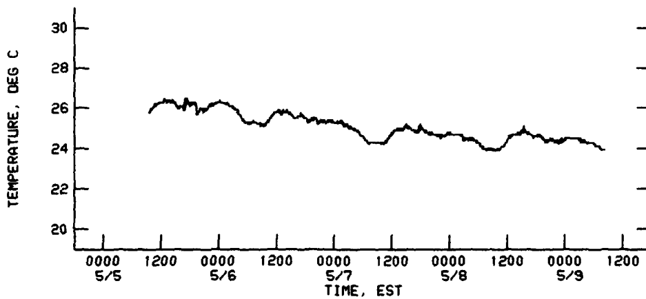
VELOCITY, TEMPERATURE, AND SALINITY AT STATION S7.0 5-9 MAY 1990
