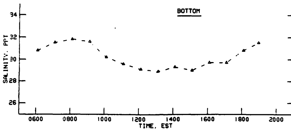
SALINITY AT STATION 4B 8 MAY 1990
