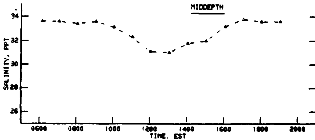
SALINITY AT STATION 1A 7 MAY 1990
