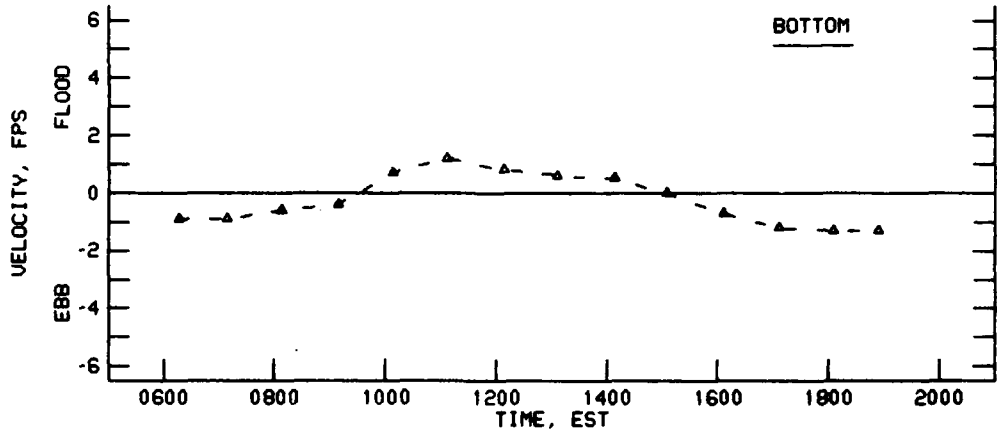
VELOCITIES AT STATION 8B 8 MAY 1990
