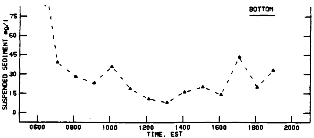
SUSPENDED SEDIMENT AT STATION 4B 8 MAY 1990
