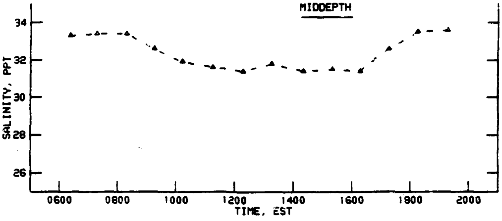
SALINITY AT STATION 2A 7 MAY 1990
