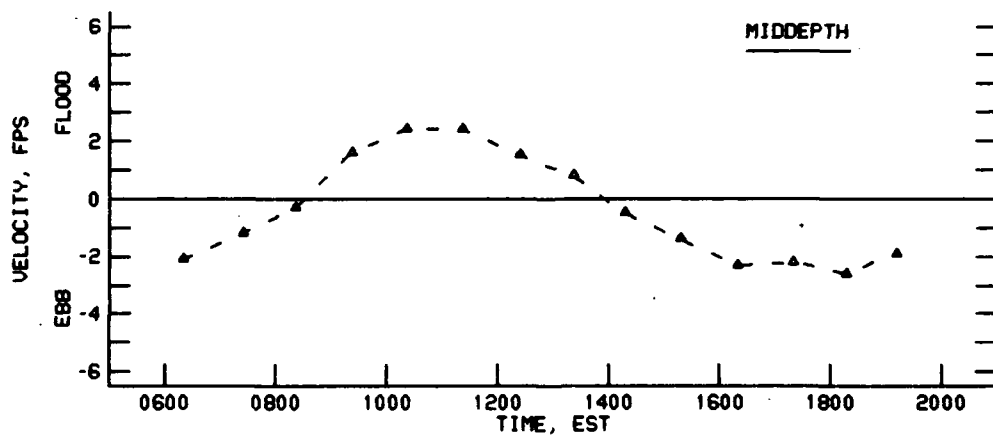
VELOCITIES AT STATION 4D 8 MAY 1990
