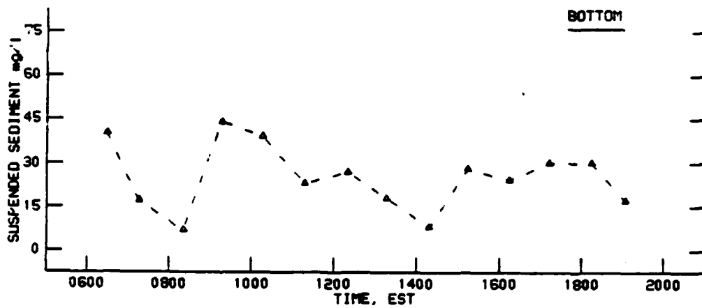
SUSPENDED SEDIMENT AT STATION 3C 7 MAY 1990
