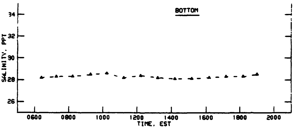
SALINITY AT STATION 8C 8 MAY 1990
