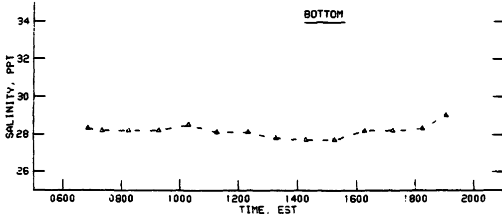
SALINITY AT STATION 7C 8 MAY 1990
