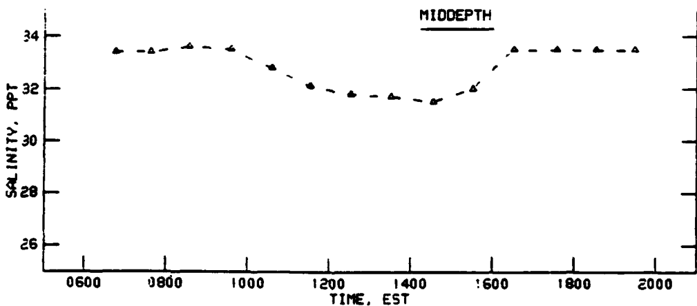
SALINITY AT STATION 1D 7 MAY 1990
