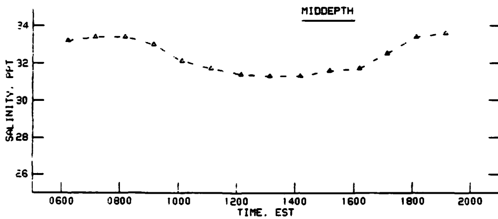
SALINITY AT STATION 2B 7 MAY 1990
