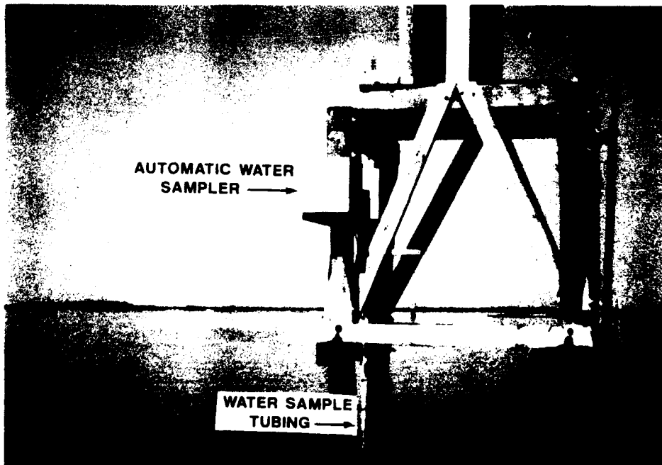
Figure 5. Typical field installation of automatic water sampler
